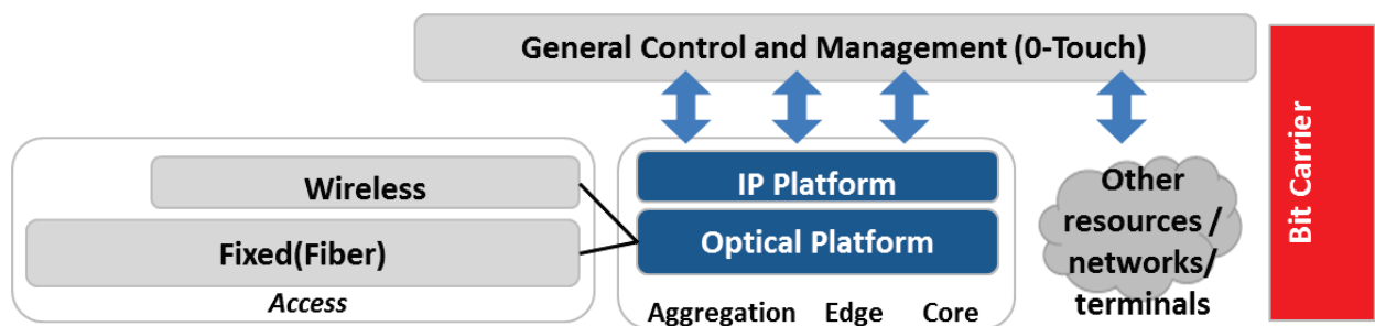
Figure 114: BitCarrier Architecture
