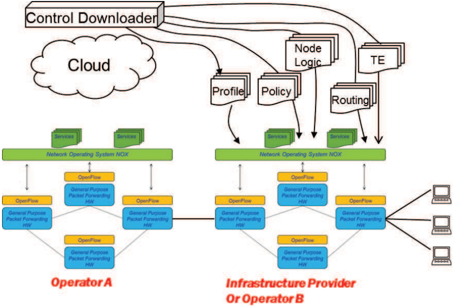
Figure 43: Deperimeterization of Networks by Means of SDN
