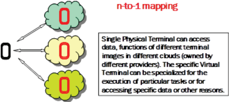
Figure 80: n-to-1 Mapping
