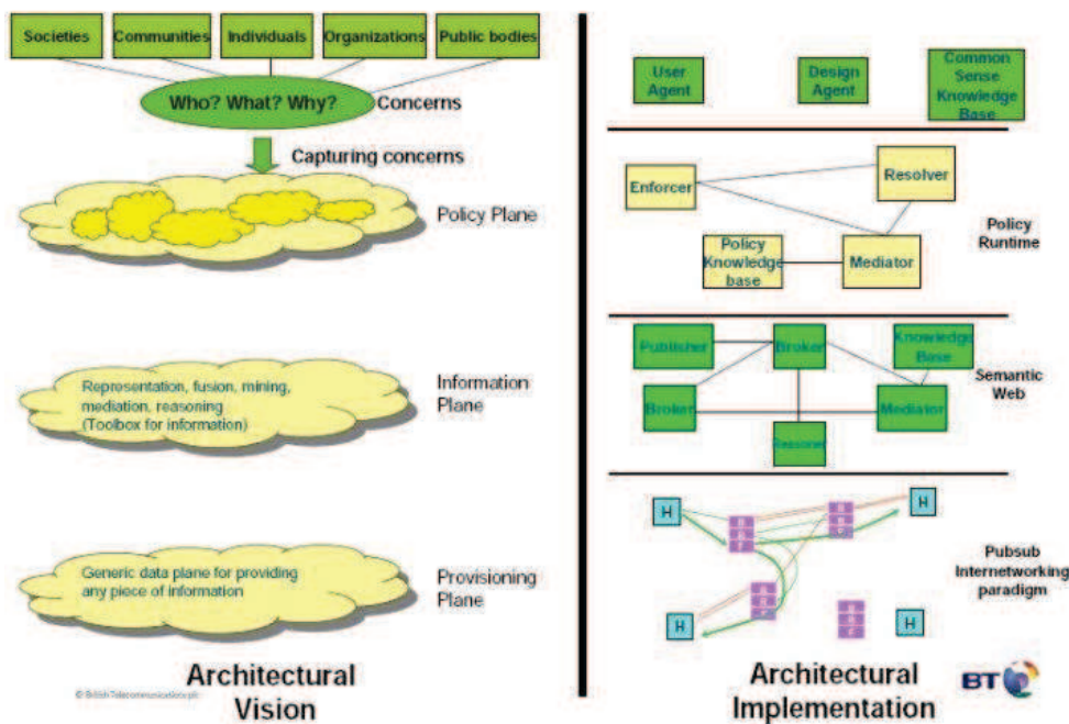
Figure 44: Architectural Vision and Architectural Implementation (Source: BT)
