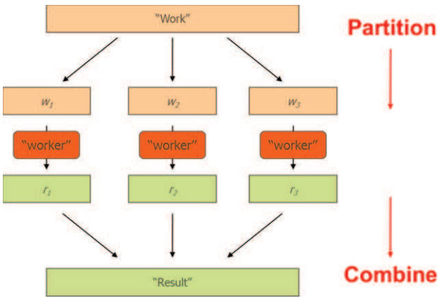
Figure 34: A MapReduce Example
