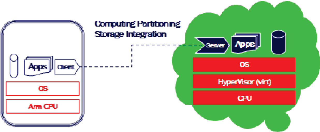
Figure 77: Virtual Terminal as a Functional Enrichment of a Terminal
