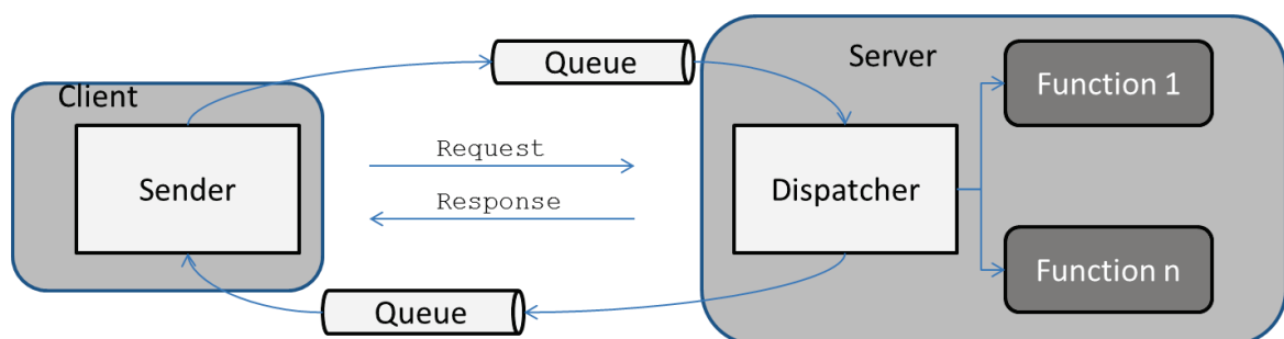
Figure 11: A C-S Relationship Implemented by means of a MP system
