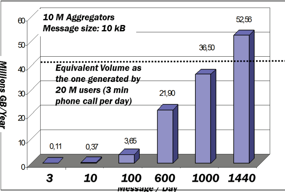
Figure 68: Examples of Traffic Generated by Sensor Aggregators.
