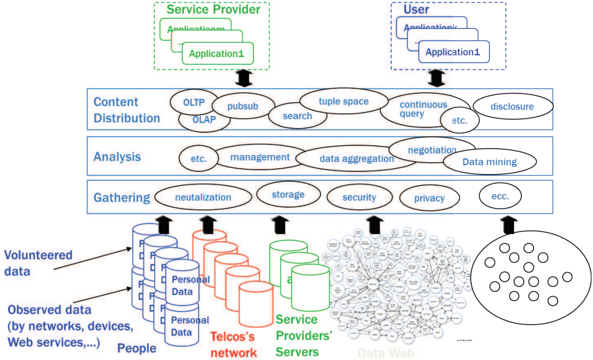
Figure 66: An Architectural Framework for a Data-centric Ecosystem
