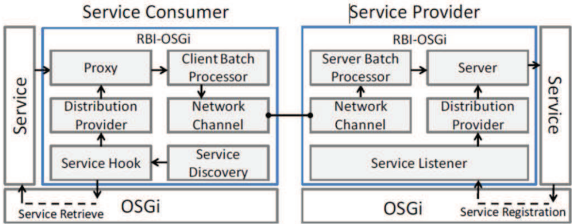
Figure 13: RBI/OSGi Architecture
