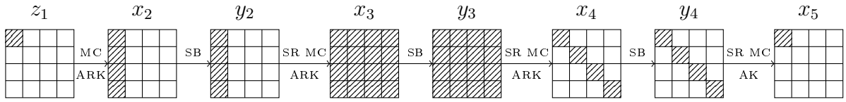
Figure 8.2: The four middle rounds used in the 7-round attack from [DKS10a]. Dashed bytes are active, others inactive.
