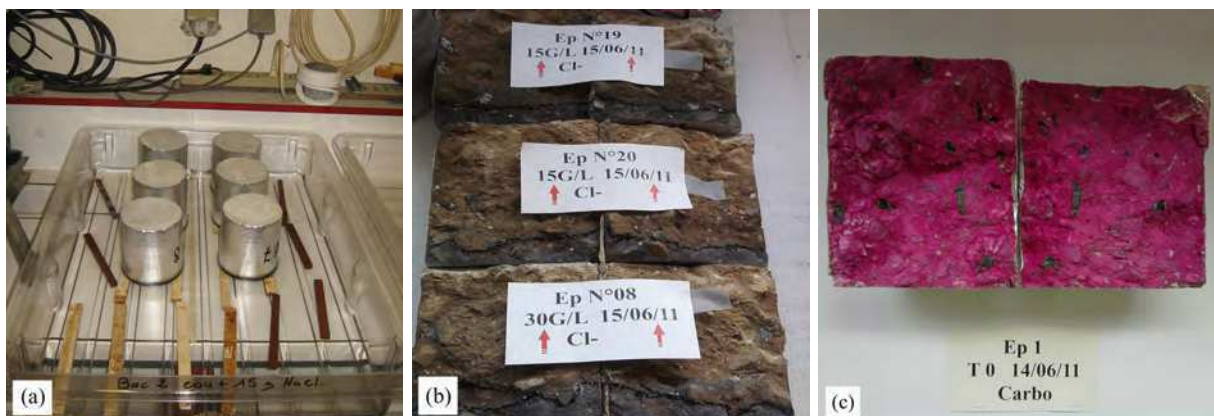
Figure 9.7: Destructive testing of witness cores with (a) conditioning for chloride ingress, (b) chloride ingress by means of \text{AgNO}_3 and (c) carbonisation by means of phenolphthalein.
