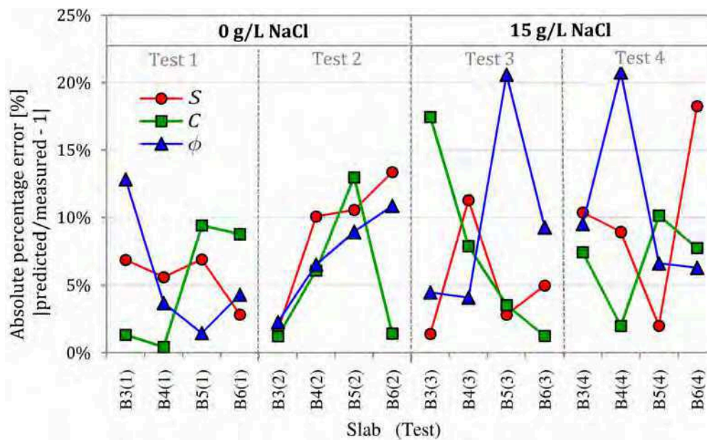
Figure 8.10: Plot of absolute percentage errors of the predicted values for the condition parameters degree of saturation, logarithm of total chloride content and porosity with respect to the measured values.
