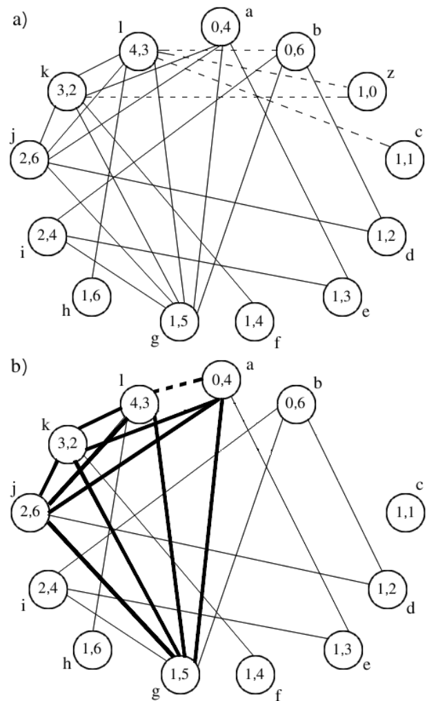
Figure 4 Example of compatibility graph constructed with classical and new methods. The CG of pattern graph PI and peptide graph GI of Figure 1 constructed with (a) classical and (b) new CG building rules. Each CG node is identified by a letter. It represents an association between a node of PI and a node of GI with compatible labels. For example, node 'a' associates node 0 of PI and node 4 of GI that both carry the 'D-Tyr' label. Dashed edges differ between the two CGs and the bold edges correspond to a clique of size 5 (size of PI).
