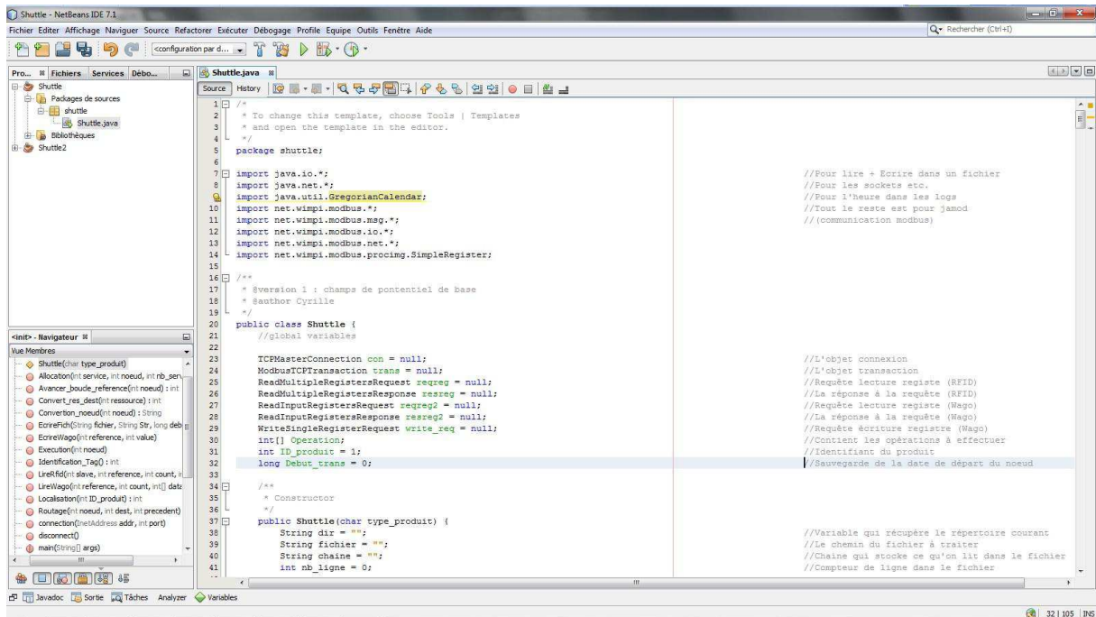
Figure 6.7– Environnement Netbeans
