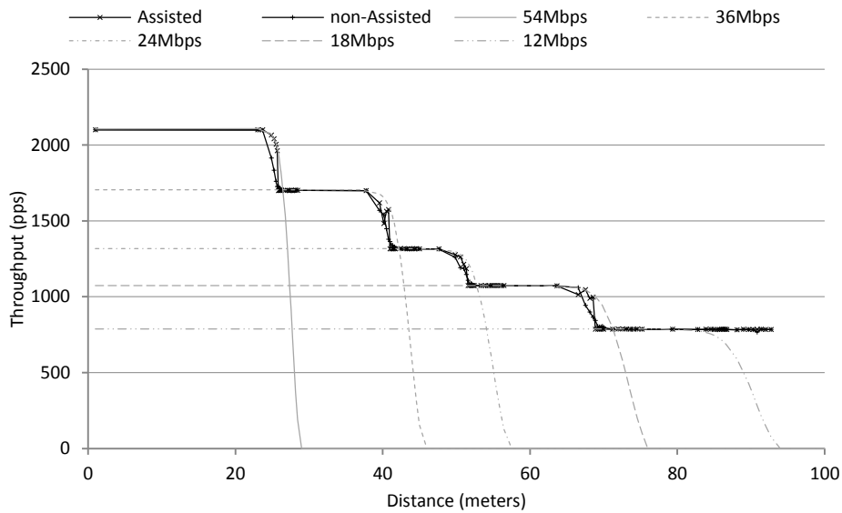
Figure 84. Immediate retry BNAK throughput for 100 members
