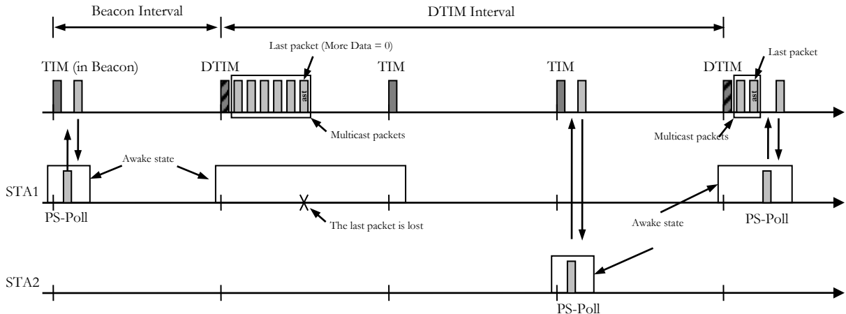
Figure 30. Infrastructure power management operation
