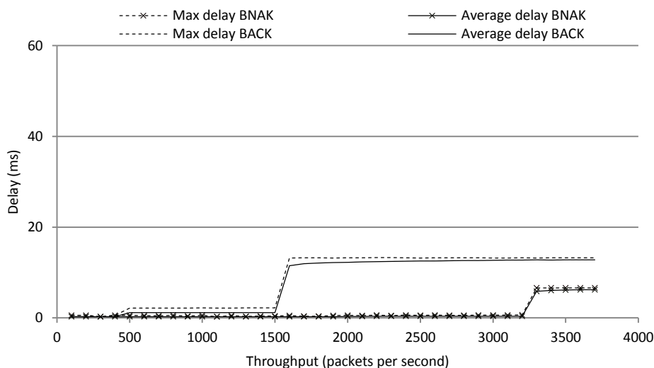
Figure 66. Buffering and transmission delays vs. throughput, G=10 members
