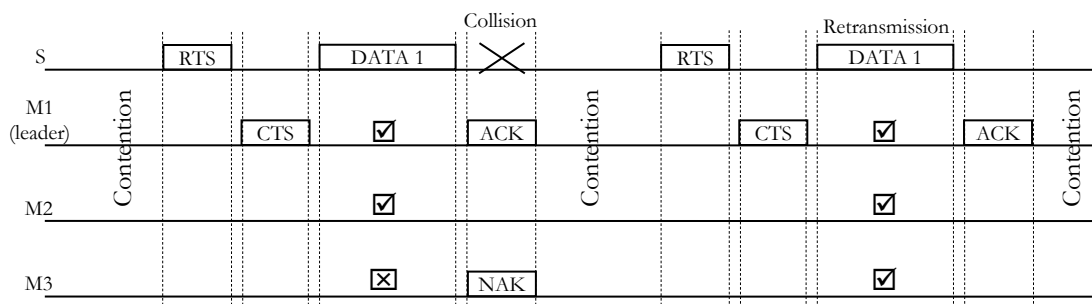
Figure 8. LBP transmission procedure
