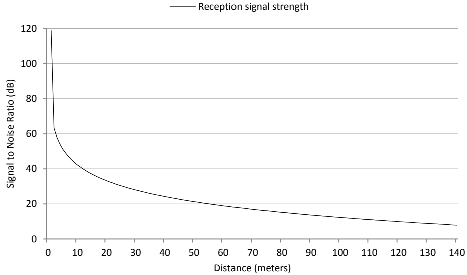
Figure 28. Reception SNIR at different distances from the AP
