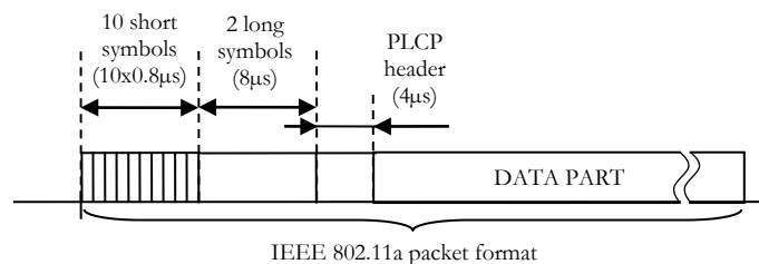
Figure 35. IEEE 802.11a (OFDM) PHY packet format
