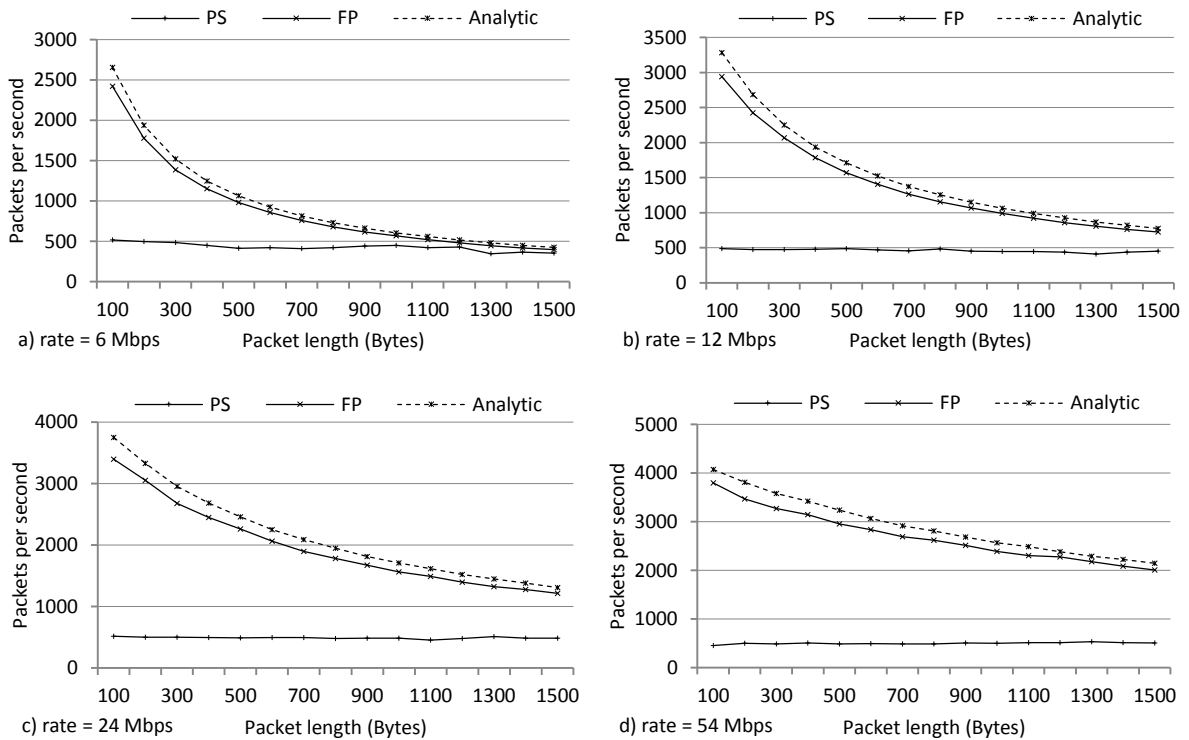
Figure 33. Multicast packets transmission rate for PHY rates of 6, 12, 24 and 54 Mbps
