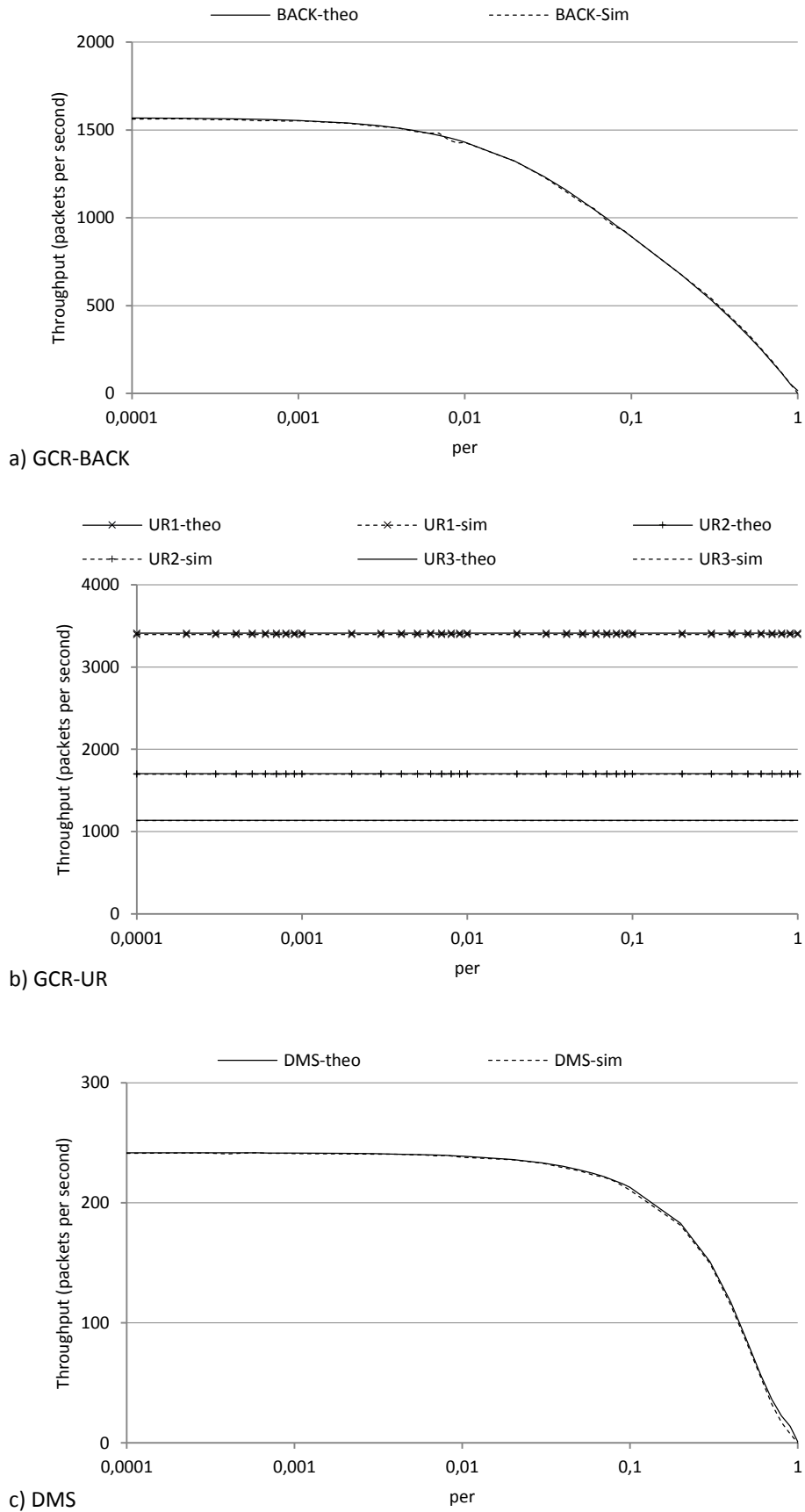
Figure 15. Model validation: throughput estimation of a) GCR-BACK, b) GCR-UR and c) DMS, for a group of 10 members and a data rate of 54Mbps
