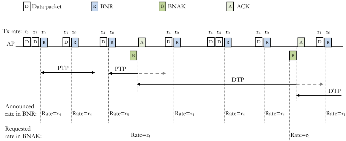
Figure 71. Transmission procedure using BNAK-ARA
