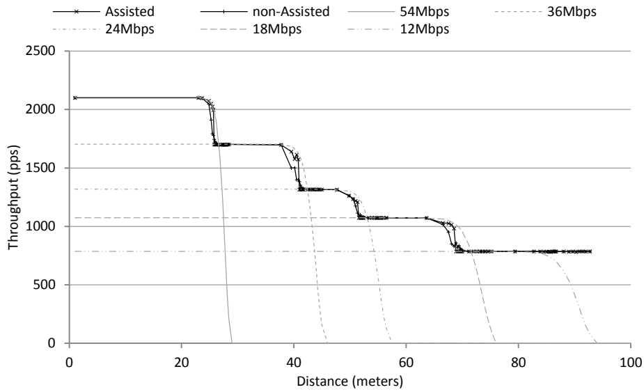
Figure 83. Immediate retry BNAK throughput for 10 members
