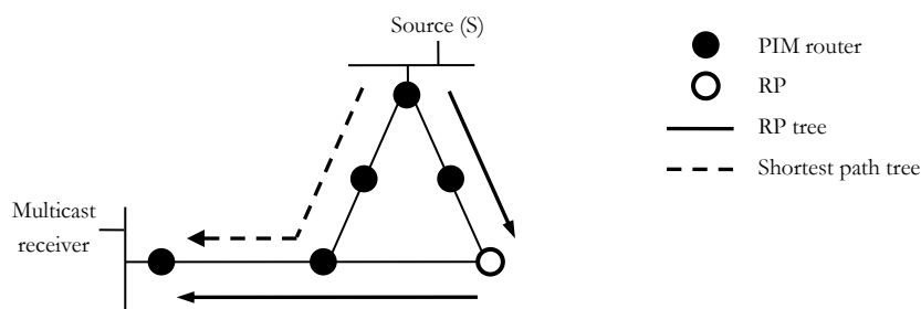
Figure 1. Network components and path creation using PIM
