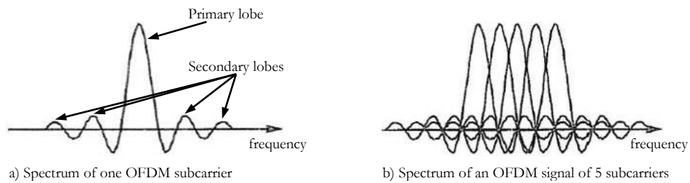
Figure 12. OFDM Subcarriers
