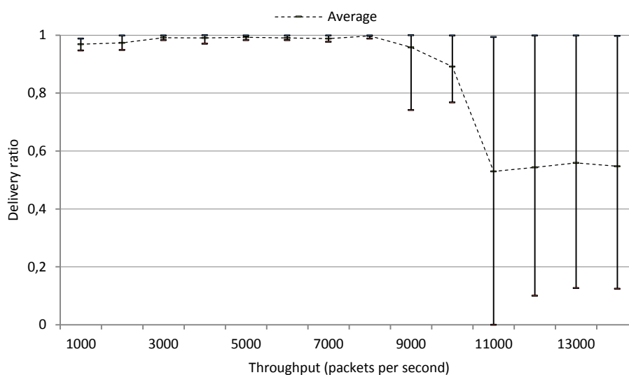
Figure 34. Impact of the packet transmission rate on the delivery ratio of multicast packets
