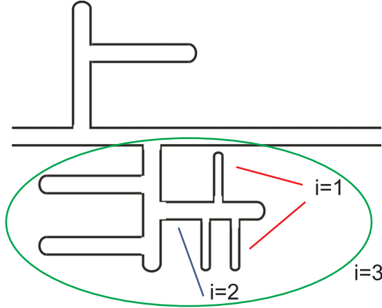
Figure 3.3. Hierarchical model of RNA-like complex. Loops of first level ( i = 1 ), second ( i = 2 ) and third ( i = 3 ) are depicted.
