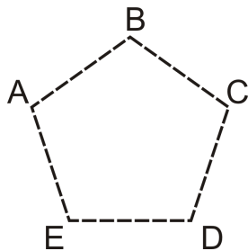
Figure 4.8. The scheme of allowed contacts for the alphabet c = 5/2
