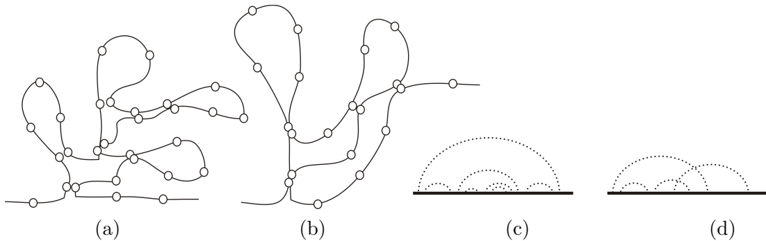
Figure 2.2. Arcs representation of RNA structure. (a,b) Schematic picture of allowed (a) cactus-like and prohibited (b) pseudoknot configurations of the bonds; (c,d): Arc diagrams corresponding respectively to configurations (a) and (b) (note the intersection of arcs in (d)).
