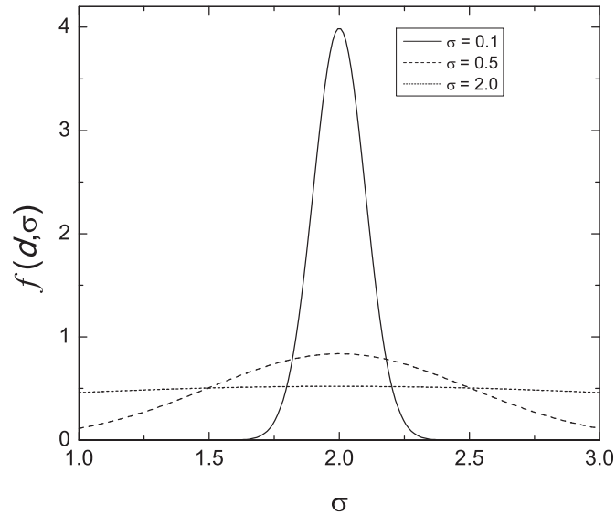
Figure 5.3. Truncated Gaussian distribution. f(\sigma) of distances between nearest-neighboring monomers for \sigma = 0.1; 0.5; 2.0 .
