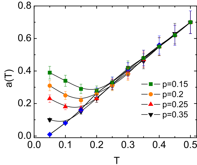
Figure 4.5. The dependence of the logarithmic proportionality coefficient of the pinching energy cost on the temperature. The simulations were done for p = 0.15, 0.2, 0.25, 0.35, 0.5 . For p larger than some threshold p^* ( 0.35 < p^* < 0.5 ), a(T) seems to follow the a(T) = 3T/2 law, corresponding to the molten phase, up to very low temperatures. For p > p^* , the a(T) -dependence deviates from the high-temperature behavior at some temperature, which we identify as a critical temperature of transition to the glassy phase. The data points are averaged over 10^4 realisations.
