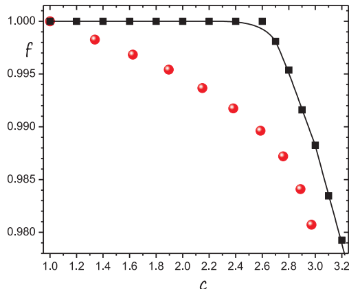
Figure 4.7. The model of correlated alphabet. The dependence of binding probability on the alphabet (the red points). Numerical results are obtained for ensemble of 10^3 samples of the length L = 5000 . For comparison the respective dependence for the Bernoulli model (the black curve) is depicted.
