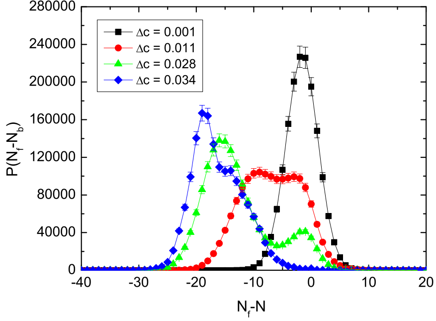
Figure 8.3. Distribution P(N) for different values of the order parameter \Delta c = 0.001, 0.011, 0.028, 0.034 . Y-axis scale is arbitrary.
