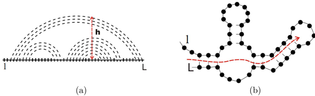
Figure 1.6. Characteristic size of RNA secondary structure. The height diagram (a) in arc representation is defined by the number of base pairs to be unzipped in the largest loop (b) [42].
