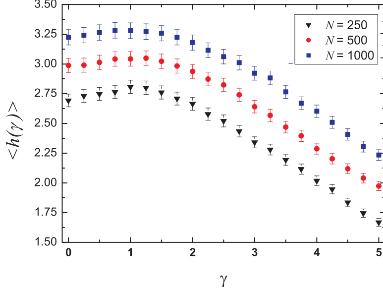
Figure 5.6. Dependence of the height, \langle h \rangle on the control parameter \gamma for the truncated power-law distribution. The simulations were performed for ensemble of 10^4 random samples.
