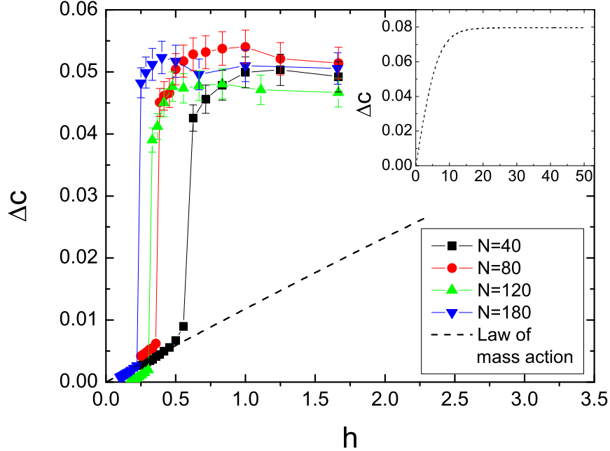
Figure 8.2. The motif distribution \Delta c(h) = c - c(h = 0) in ER networks with p = 0.35 re-equilibrated at different h . Solid lines – numerical results for networks of sizes N = 40, 80, 120, 180 , dashed line – prediction of the law of mass action (8.7). Inset: law of mass action extended to a region of large h .
