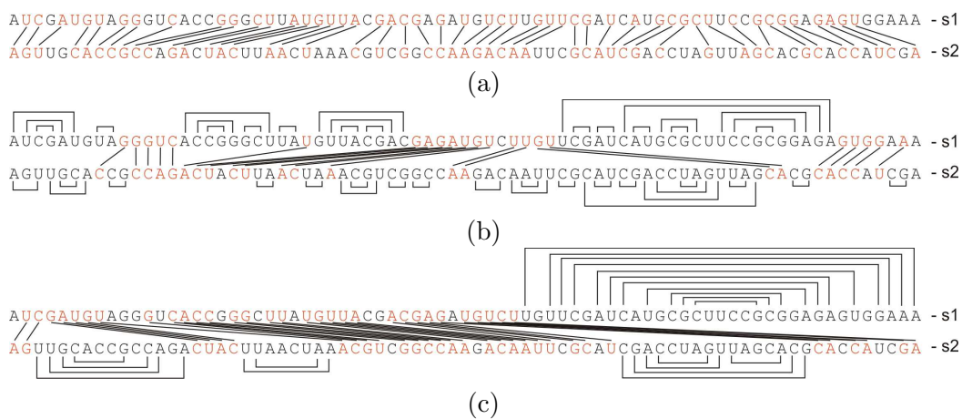
Figure 2.7. Structures recovered from the pair of sequences [100]. (a) Linear structure, (b) branching structure, (c) branching structure with the restriction on the size of the minimal loop (there are no loops less than 4 nucleotides).
