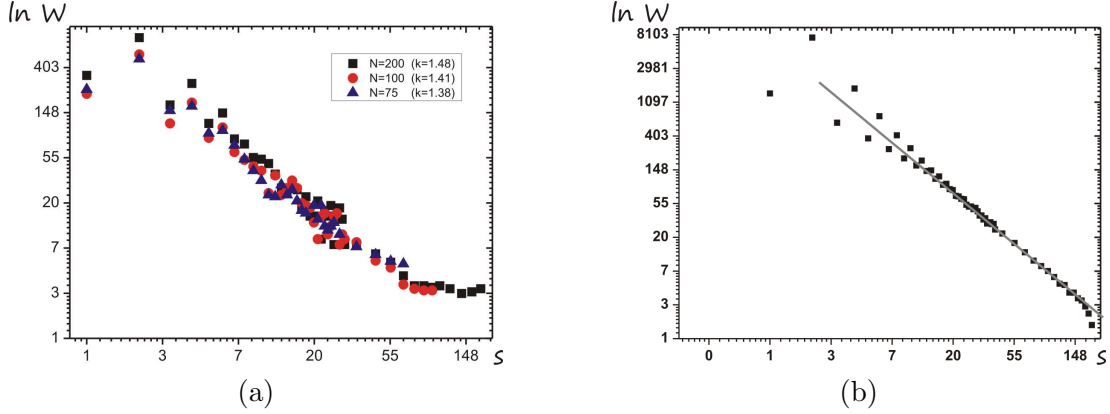
Figure 3.5. Loop length distribution in RNA-type complex. (a) The loop length distribution in a cactus-like complex of two RNAs (The simulations were performed for the ensembles of 10^3 random samples with the sequence lengths n = m = 75, 100, 200 ; for s \geq 30 the distribution function was smoothed over 10 adjacent values); (b) The Motzkin path length distribution (the random walk length is 200, the number of samples is 10^3 , for s \geq 30 the function was smoothed over 10 adjacent values).
