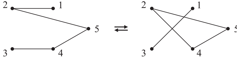
Figure 8.1. Possible triads in a non-directed network and an example of a single permutation step. The links (12) and (34) are removed, and the links (13) and (24) are added instead, thus conserving degrees of all the nodes involved. The network has 5 nodes, so only one elementary reaction occurs: one triad of type 0 ( \{135\} ) and three triads of type 2 ( \{125, 245, 345\} ) are deleted, and one triad of type 3 ( \{245\} ) and three triads of type 1 ( \{125, 135, 345\} ) are created.
