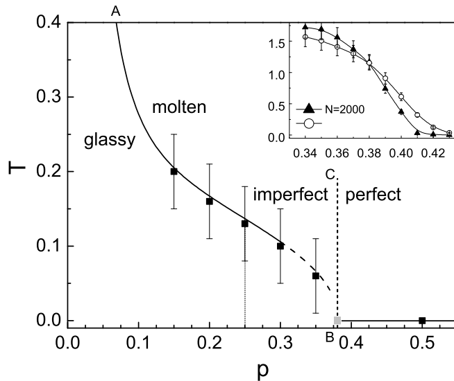
Figure 4.6. The phase diagram of Bernoulli model on the (T, p) plane. The data points correspond to the critical temperature T_c of the molten-glass transition for different values p = 0.15, 0.2, 0.25, 0.3, 0.35, 0.5 . An intensively studied case, corresponding to a 4-letter alphabet ( p = 0.25 ), is highlighted by a thin dashed line. The critical curve (A-B) separates glassy and molten phases. We conjecture that at zero temperature, the critical curve's endpoint B position p^* coincides with the critical point p_c for the perfect-imperfect transition. The thick dashed line (B-C) separates the perfect and imperfect regions of the phase diagram, and the glassy phase lies entirely inside the region, characterized by gaps. Inset – an evidence for the conjecture p^* = p_c : study of the pinching free energy \Delta F(L, T) at zero temperature. In the limit of large L , the glassy phase is absent for p > p^* , characterized by \Delta F(\infty, 0) = 0 . The point p^* can be identified as a crossing point for different \Delta F(L, 0) curves, presented here for L = 1000 and L = 2000 , and it's value is found to be very close to p_c = 0.379 .
