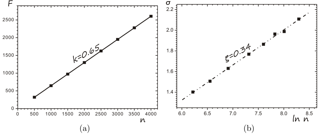
Figure 3.1. Statistics for linear complex of two random RNAs. Free energy (a) and energy fluctuation (b) in dependence on the sequence length.
