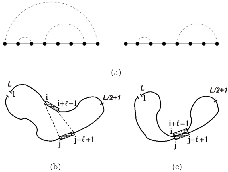
Figure 1.4. The pinch energy calculation procedure. (a) division of a chain into halves restrict the number of possible configurations; (b) shows the positions of two pieces with exactly complementary bases, one of which is between positions 1 and L/2 and the other of which is between positions L/2 + 1 and L . Such a piece of length l \sim \ln L can be found for almost all sequences; (c) shows how restricting configurations to those in which the good match forms Watson-Crick base pairs splits the molecule into two loops, which can still form base pairs within the loops independently of each other [43]
