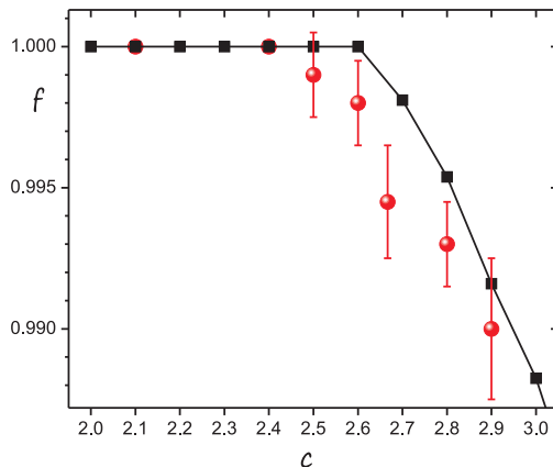
Figure 4.9. The model of rational alphabet. The dependence of binding probability on the alphabet (the red points). Numerical results are obtained for ensemble of 10^3 samples of the length L = 1000 . For comparison the respective dependence for the Bernoulli model (the black curve) is depicted.
