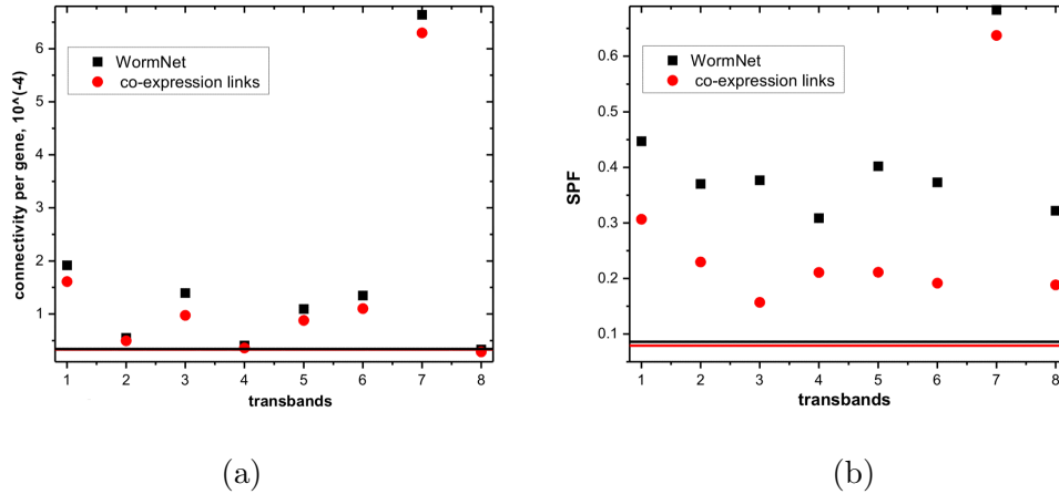
Figure 7.2. Statistical properties of eQTL-hotspots. The connectivity coefficient per gene in an eQTL-hotspot group (a) and the SPF coefficients (b) in whole WormNet (black) and in its expression sub-part (red). The black and red lines are the respective functions for equally sized random set of genes.
