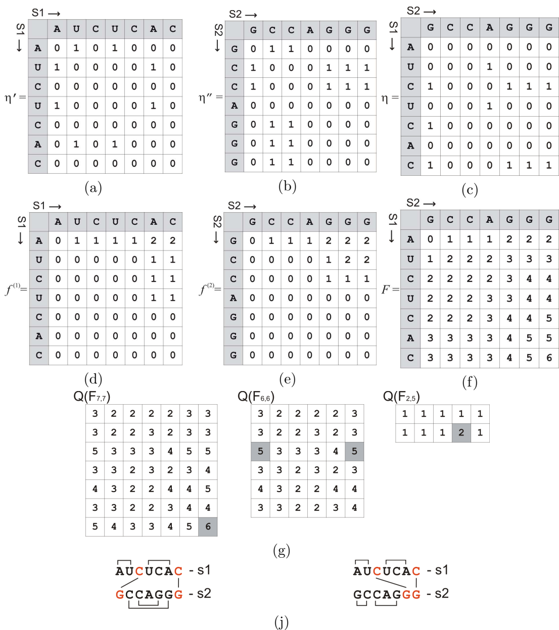
Figure 2.6. The algorithm description for RNA-type complex. Incidence matrices for pairs of chains with possible clover-leaf structures inside each sequence: (a) intra-matching S1-S1, (b) intra-matching S2-S2, (c) inter-matching S1-S2; the free energy matrices: (d) for the 1-st sequence, (e) for the 2-nd and for the complex f ; the matrices Q (g), involved in the structure recovery procedure; (j) the predicted RNA-RNA complex structures.
