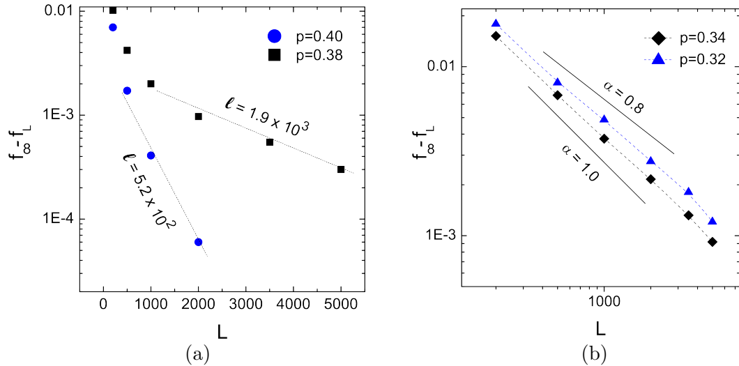
Figure 4.3. Convergence of fraction of links, involved in planar binding, f_L to the limiting value f_\infty in two regimes, p > p_c and p < p_c . (a) In the perfect phase, the exponential convergence is demonstrated for p = 0.38 and p = 0.4 in the semi-logarithmic scale. The screening length \ell(p) diverges as p approaches the critical value p_c . (b) In the imperfect phase, the power-law behavior is shown for p = 0.32 and p = 0.34 in the log-log scale. The exponent \alpha(p) as a function of p takes values between 0.8 and 1. The data points are averaged over 1000 realisations.
