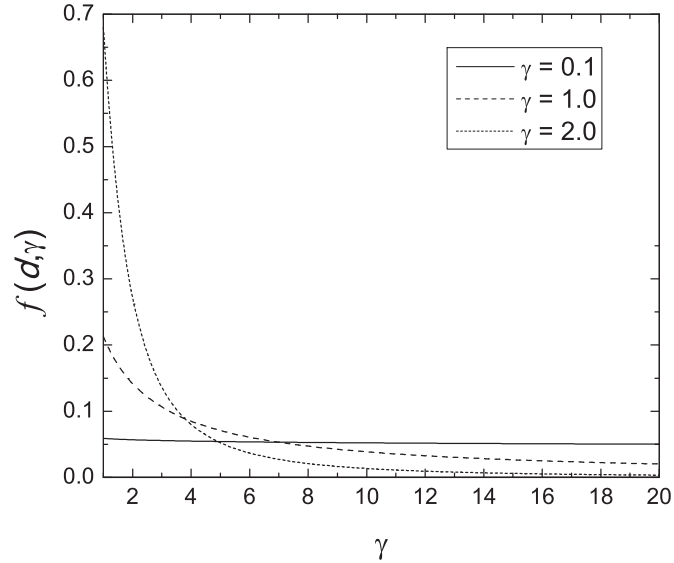
Figure 5.5. Power-law distribution function. f(d, \gamma) of distances between nearest-neighboring monomers for \gamma = 0.1; 1.0; 2.0 .
