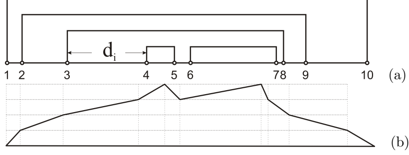
Figure 5.2. Typical configuration of a random interval RNA. Structure is shown by arcs (a), and by a height diagram (b).
