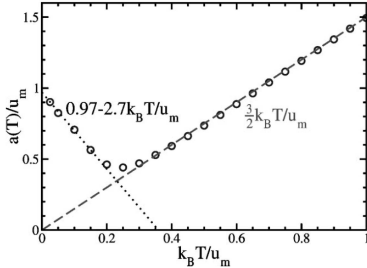
Figure 1.5. Prefactor a(T) of the logarithmic dependence (1.5) for random RNA sequences generated by the sequence disorder model. At high temperatures, the prefactor indicated by the circle is well described by the dashed line (3/2)k_B T expected of the molten phase [43]
