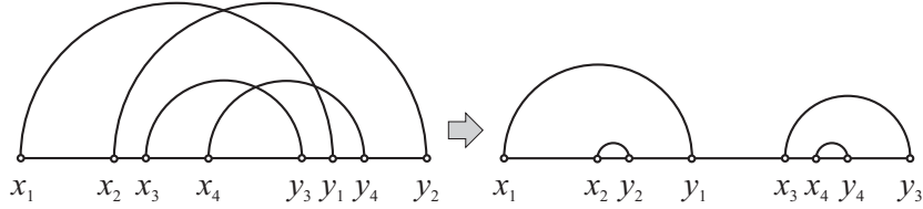
Figure 5.1. Optimization procedure. The use of concave-type cost function leads to the planar pairing.
