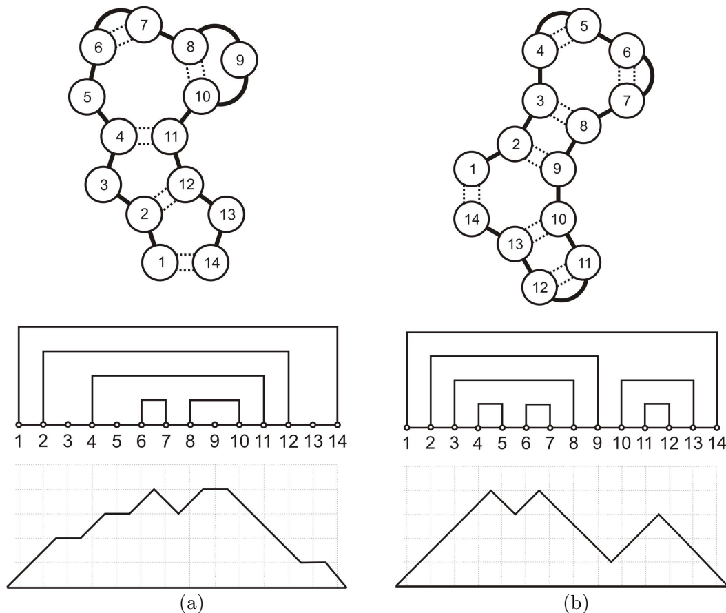
Figure 3.6. Random walk representation of RNA structure. Secondary structure of RNA with gaps and respective Motzkin path (a); perfect matching RNA structure without gaps and respective Dyck path (b).
