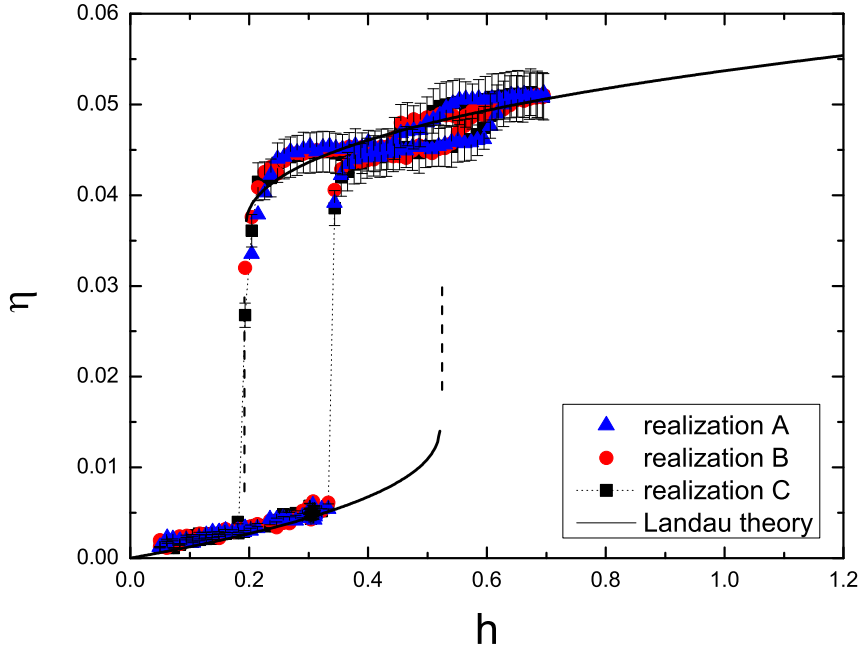
Figure 8.4. Comparison of the numerically observed dependence \Delta c(h) to the solution of the mean-field equation (8.10). The following values of theory parameters are taken \chi = 85 ; b = 4.55 \times 10^3 g = 6.5 \times 10^4 .
