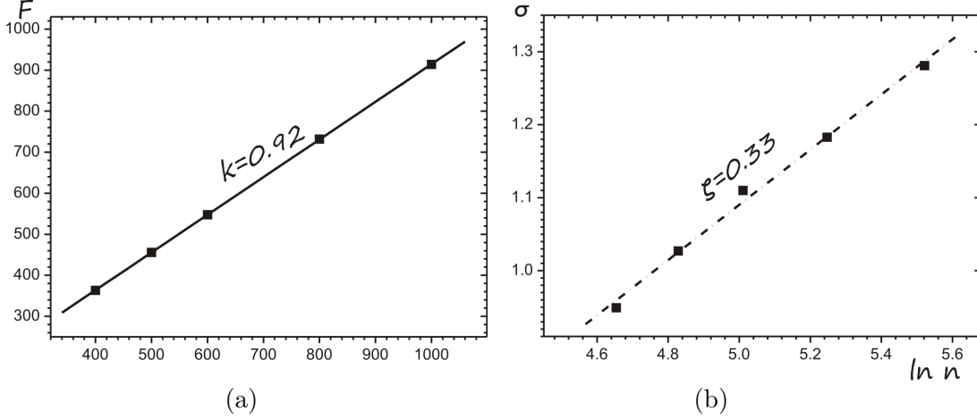
Figure 3.2. Statistics for RNA-type complex of two random RNAs. Free energy (a) and energy fluctuation (b) in dependence on the sequence length.
