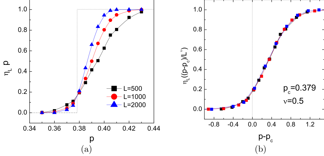
Figure 4.2. Numerical results for Bernoulli random polymer model. (a) The fraction of perfect matchings \eta_L(p) as a function of the density p of ones in the contact matrix V for chain lengths L = 500, 1000, 2000 , averaged over 10^4 realisations. The dashed line corresponds to the thermodynamic limit L \rightarrow \infty , yielding the critical value p_c = 0.379 . (b) The scaling analysis of curves, corresponding to the different chain lengths L . The fitting procedure gives the exponent of the transition width \nu = 0.5 .
