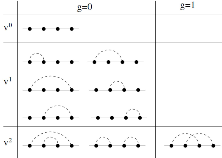
Figure 1.7. All possible arc diagrams with L = 4 . Diagrams with i arcs are associated with the power v^i , and g is the genus.
