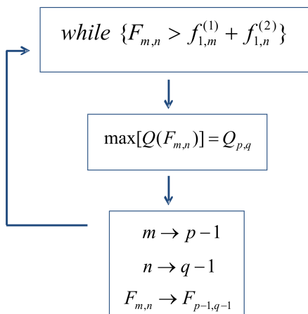
Figure 2.5. The structure recovery algorithm scheme for RNA-type complex.
