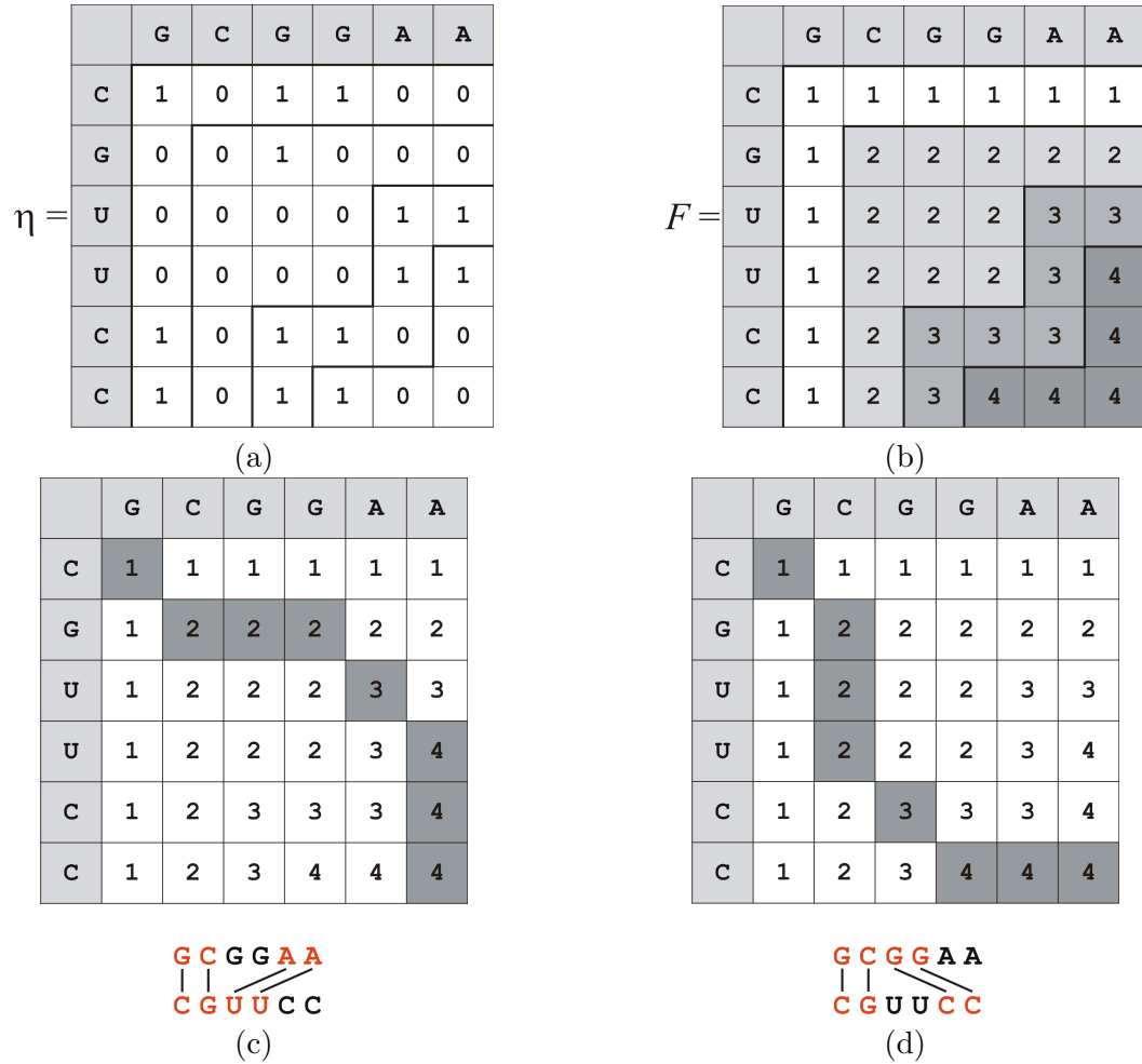
Figure 2.4. Linear pairing algorithm. (a) Incidence matrix \eta , (b) ground state free energy matrix F ; (c)-(d) structure recovery algorithm for linear chains.
