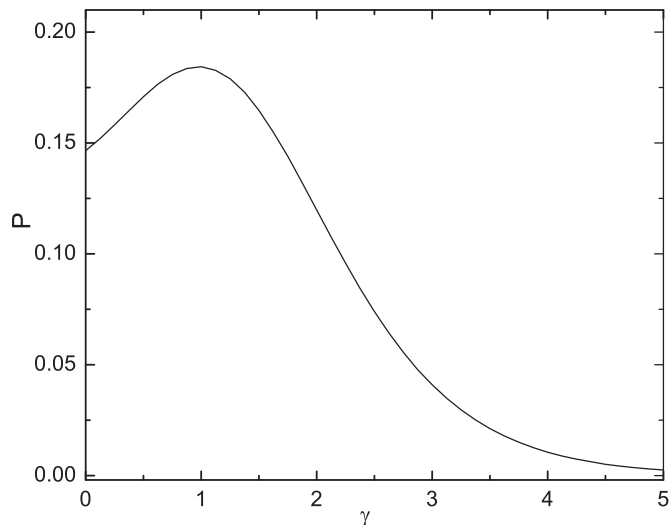
Figure 5.8. Analytical estimate for the truncated power-law distribution. Dependence of the probability P (5.15) on the control parameter \gamma .
