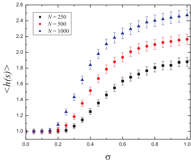
Figure 5.4. Dependence of the average height, \langle h \rangle on the control parameter \sigma for the Gaussian truncated distribution. The simulations were done for ensemble of 10^4 polymers.
