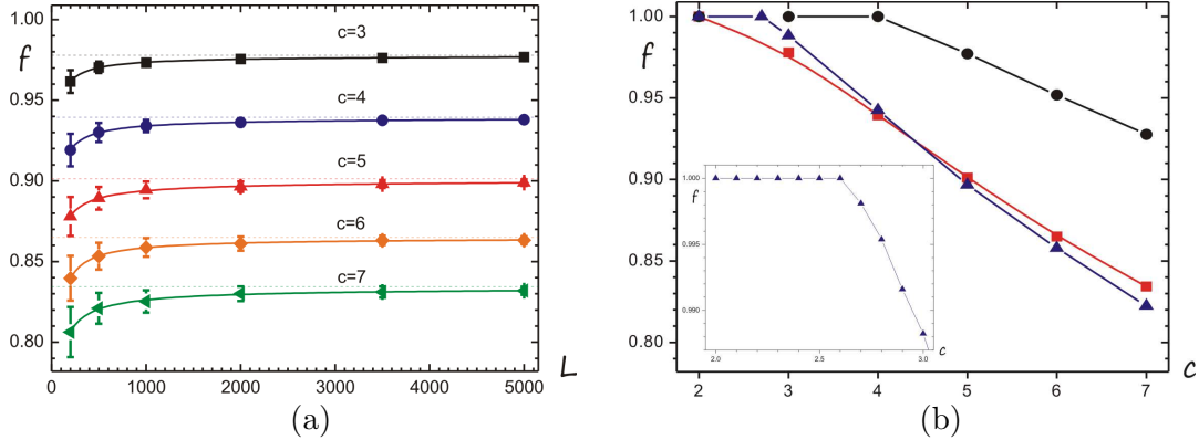
Figure 4.1. Energy dependence for random RNA-type polymers. (a) The dependence of specific free energy on the sequence length at different alphabet c . (b) The dependence of the limiting energy f_\infty(c) on the alphabet for alphabetic sequences (the red curve), for the Bernoulli polymer (the blue curve) and upper analytical estimate (the black curve).
