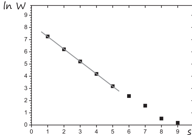
Figure 3.4. Loop length distribution in linear complex of two RNAs. The calculations were performed for random polymers of the length n = 10^4 , the graph is averaged by the ensemble of 10^4 complexes.
