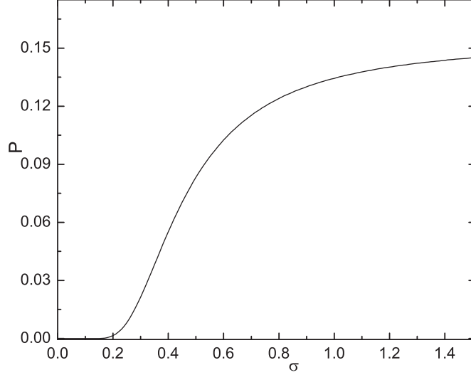
Figure 5.7. Analytical estimate for the truncated Gaussian distribution. Dependence of the probability P (5.15) on the control parameter \sigma .
