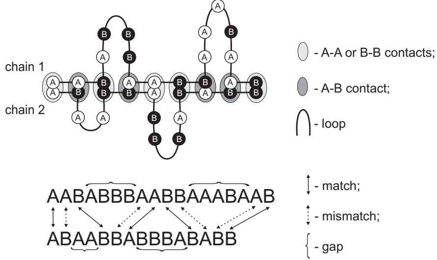
Figure 2.1. Linear pairing complex. Schematic picture of binding of two heteropolymer chains with two types of letters ( c = 2 ).
