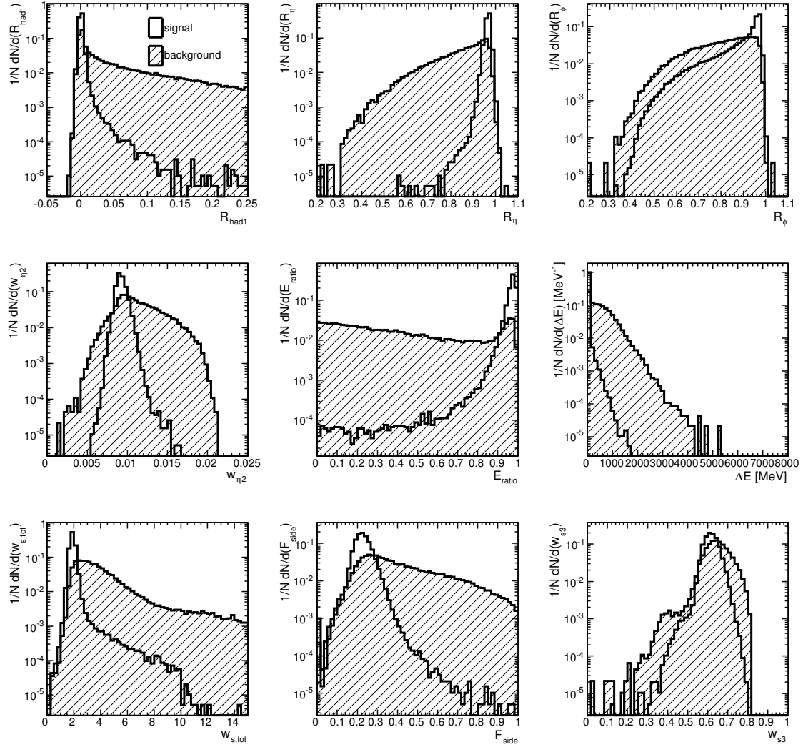
Figure 2.3: Normalized distributions of the calorimetric discriminating variables in the region 0 < |\eta| < 0.6 for E_T > 20 GeV for true and fake photons reconstructed as converted before any selection.
