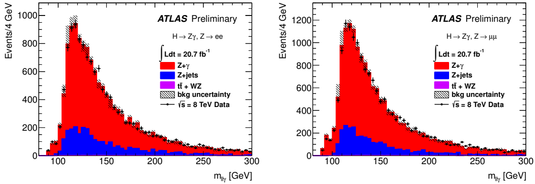
Figure 4.11: Three-body invariant mass ( m_{\ell\ell\gamma} ) distribution of selected events in \sqrt{s} = 8 TeV data (dots) and from the various background sources (histograms, from the simulation) normalized to the yields determined as described in the text, for Z \rightarrow ee (left) and Z \rightarrow \mu\mu (right) channels. The background uncertainty includes statistical uncertainties and systematic uncertainties from the inputs taken from the simulation, as detailed in the text.
