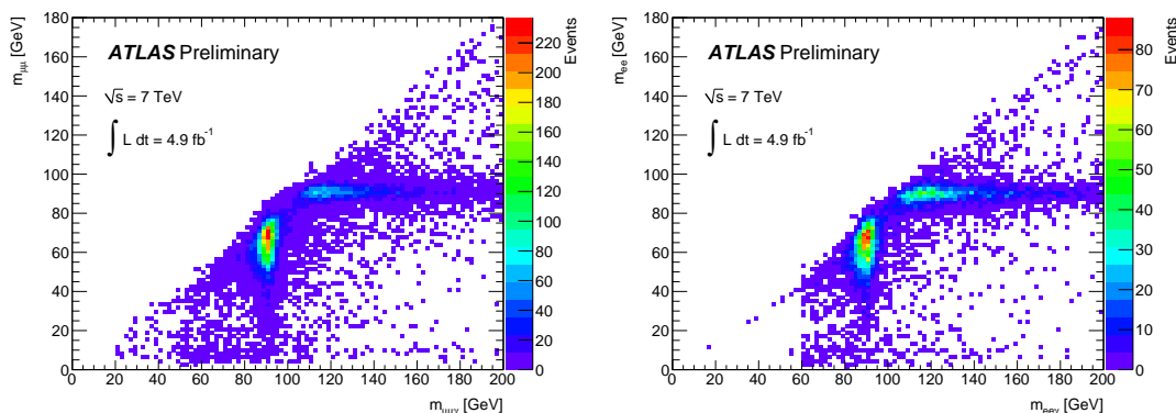
Figure 2.8: Distribution of the invariant masses m_{ll\gamma} vs m_{ll} from photon candidates in the full 2011 data set after event selection, for \mu\mu\gamma (left) and ee\gamma (right) events.
