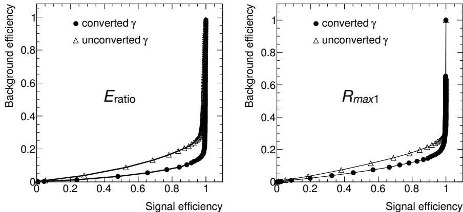
Figure 2.5: True (signal) versus fake (background) efficiency of a selection based only on the variable E_{ratio} (left) or the variable R_{max1} (right), for photon candidates reconstructed in |\eta| < 0.6 and with 25 \text{ GeV} < E_T < 40 \text{ GeV} before any selection, separately plotted for unconverted (open triangles) and converted (full circles) candidates.
