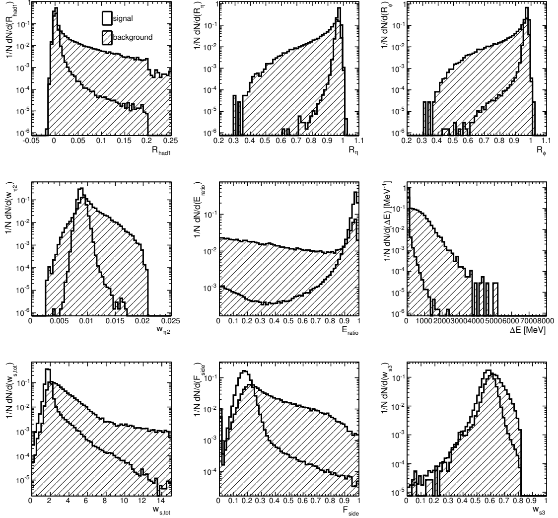
Figure 2.2: Normalized distributions of the calorimetric discriminating variables in the region 0 < |\eta| < 0.6 for E_T > 20 GeV for true and fake photons reconstructed as unconverted before any selection.
