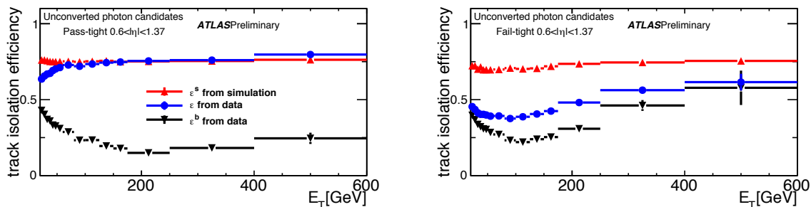
Figure 2.10: Track isolation efficiencies for unconverted signal and background photon candidates with 0.6 < |\eta| < 1.37 passing ( \epsilon_p : left figure) or failing ( \epsilon_f : right figure) the tight criteria, as measured in data and from MC simulated samples. The red triangles show the signal track isolation efficiency as obtained from simulation, whereas the black triangles show that of background, as determined from data using the relaxed-tight photon control sample. The blue circles show the overall track isolation efficiency found in data (signal and background together). Only statistical uncertainties are shown.
