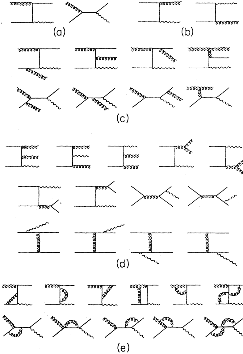
Figure 3.1: Selection of Feynman diagrams for prompt photon production: (a) \mathcal{O}(\alpha_s) Compton subprocess, qg \rightarrow q\gamma (and \bar{q}g \rightarrow \bar{q}\gamma ); (b) \mathcal{O}(\alpha_s) annihilation subprocess, q\bar{q} \rightarrow g\gamma ; (c) \mathcal{O}(\alpha_s^2) subprocess qg \rightarrow \gamma qq (and \bar{q}g \rightarrow \gamma \bar{q}q ); (d) \mathcal{O}(\alpha_s^2) subprocesses q\bar{q} \rightarrow \gamma gg and q\bar{q} \rightarrow \gamma q\bar{q} ; (e) one-loop graphs for the Compton subprocess that contribute to the \mathcal{O}(\alpha_s^2) calculation [129].
