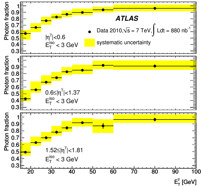
Figure 3.8: Fraction of isolated prompt photons as a function of transverse energy in the photon candidate sample selected in 0.88 \text{ pb}^{-1} of pp collisions at \sqrt{s} = 7 \text{ TeV} , for the three pseudorapidity ranges under study.
