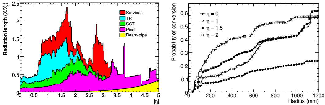
Figure 1.8: Left: material in the inner detector (distance from the beampipe R < 1150 mm), in units of radiation length, as a function of |\eta| . Right: probability of a photon to have converted as a function of R for different values of pseudorapidity.
