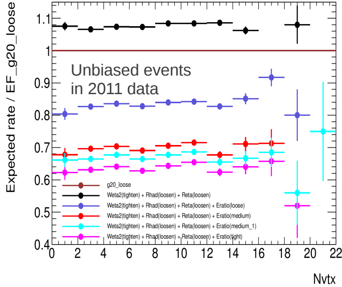
Figure 2.18: Ratio between the rate of various single-photon triggers (with E_T threshold equal to 20 GeV) proposed for the 2012 data-taking and the rate of the single-photon trigger with 20 GeV threshold used in 2011, based on data collected with the high-level photon trigger operating in pass-through mode.
