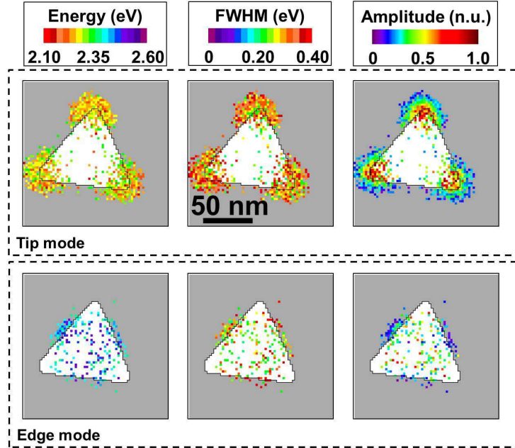
Figure 4.5: EELS multipole fitting. Maps of the energy, FWHM and amplitude of the peaks whose central energy and FWHM match the resonances appearing in the Tip EEL spectrum (Tip mode) and in the Edge EEL spectrum (Edge mode).
