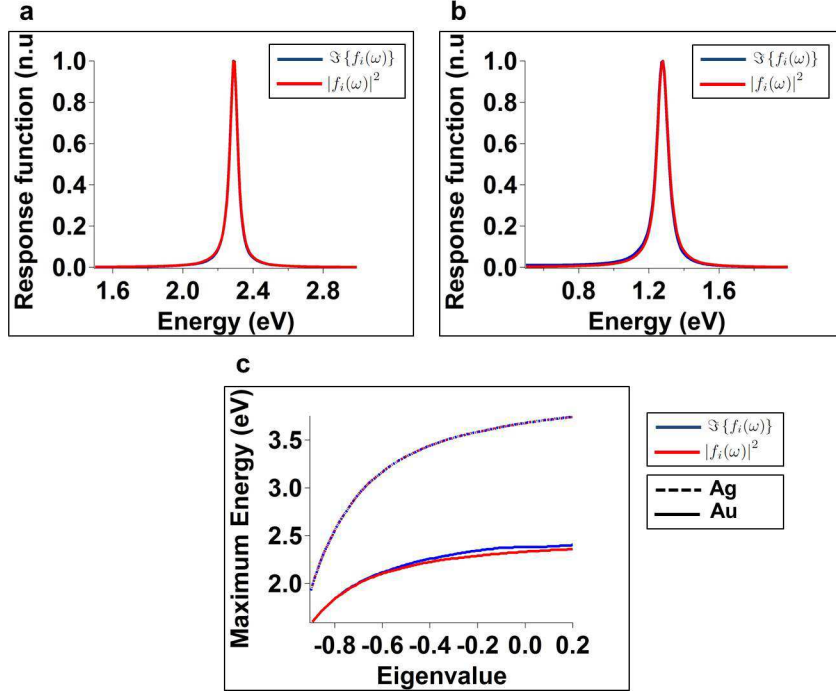
Figure B.4: \Im\{f_i(\omega)\} and |f_i(\omega)|^2 for different parameters. a) \epsilon_1(\omega) = \epsilon_{Ag}(\omega) , \epsilon_2(\omega) = 1 and \lambda_i = -0.85 . b) \epsilon_1(\omega) = \epsilon_{Au}(\omega) , \epsilon_2(\omega) = 1 and \lambda_i = -0.95 . c) Maximum of \Im\{f_i(\omega)\} and |f_i(\omega)|^2 as a function of the eigenvalue of the mode \lambda_i .
