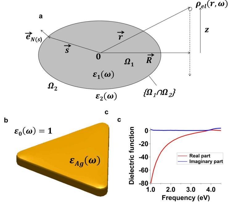
Figure 2.2: a) Schematic representation of a generic 3D system consisting in some object \Omega_1 of local dielectric function \epsilon_1(\omega) embedded in a matrix \Omega_2 of local dielectric function \epsilon_2(\omega) . In this sketch, O denotes the origin of the vector space, \vec{r} an arbitrary vector, \vec{s} a vector pointing to the interface \{\Omega_1 \cap \Omega_2\} and \vec{e}_{N(s)} a normal unit vector located at position \vec{s} on the boundary pointing outside the object. The fast electron whose trajectory along the z axis writes \vec{r}_e(t) = \vec{R} + \vec{v}t = R\vec{e}_\perp + z\vec{e}_z enters the Maxwell equations through an external charge density current \rho_{el}(\vec{r}, t) in real space, or \rho_{el}(\vec{r}, \omega) in Fourier space. b) System modelled numerically: a silver nanoprism embedded in vacuum. c) Real and imaginary part of the local dielectric function of silver. Obtained from [74].
