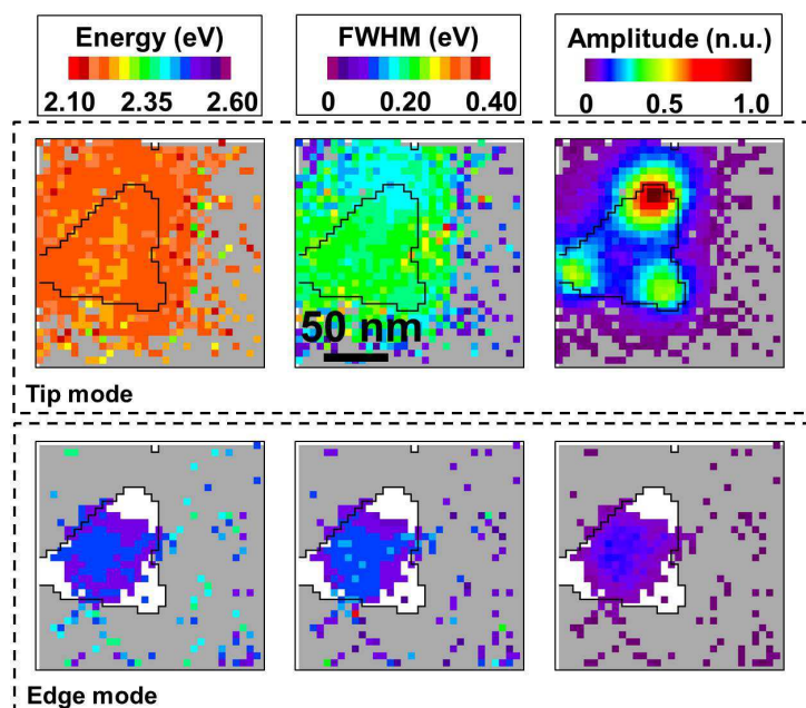
Figure 4.7: CL multippeak fitting. Maps of the energy, FWHM and amplitude of the peaks whose central energy and FWHM match the resonances appearing in the Tip CL spectrum (Tip mode) and in the Edge CL spectrum (Edge mode).
