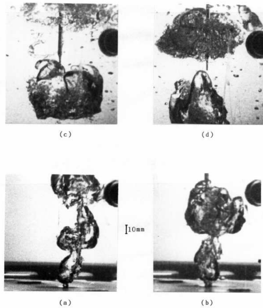
Figure 5.9 Large bubbles occurring at different positions in the plume. ( Q = 876 \text{ Ncm}^3/\text{s} , h_p = 400 \text{ mm} , d = 6.35 \text{ mm} , probe at centreline z = 110 \text{ mm} for (a) and (b), z = 200 \text{ mm} for (c) and (d) photographs).
