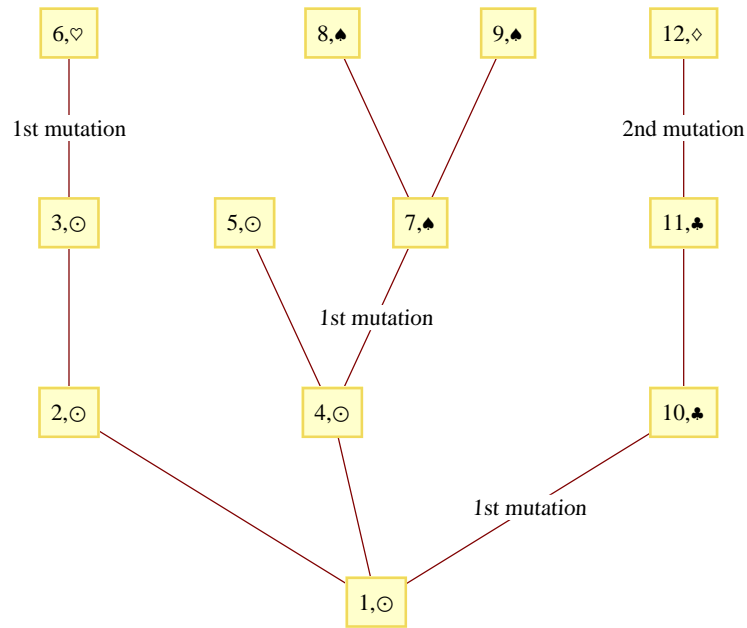
FIGURE 2.1 – The Galton-Watson process with neutral mutations. The symbols \ominus, \heartsuit, \clubsuit, \diamond, \spadesuit represent the different alleles. At the same time we enumerate all the vertices.
