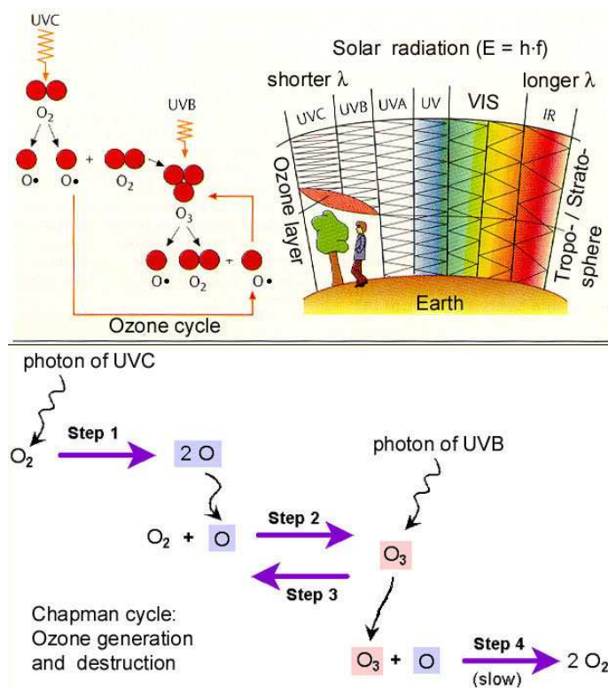
Figure 1.7: A graphical representation of the production and destruction of ozone through the Chapman cycle (image courtesy: http://biophysics.sbg.ac.at ).
