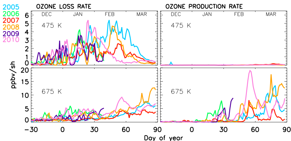
Figure 4.6: Vortex averaged ( \geq 65^\circ EqL) chemical ozone loss and production rates at 475 and 675 K, expressed in \text{ppbv sh}^{-1} , for the Arctic winters 2004/05–2009/10. The data are exempted from temporal smoothing to explicitly show the effect of daily movement of vortex and its impact on ozone production and loss rates.
