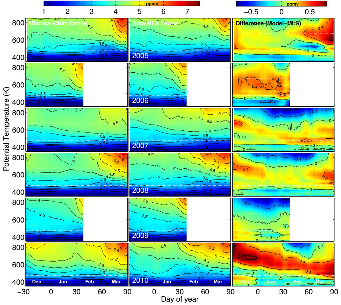
Figure 4.2: Temporal evolution of the vertical distribution (350–850 K) of vortex averaged ( \geq 65^\circ EqL) ozone (ppmv) for the Arctic winters 2004/05–2009/10. Left: MIMOSA-CHIM calculations, Middle: MLS measurements and Right: The difference between modelled and measured ozone. The model fields are sampled at location of the MLS observations. Due to early vortex dissipation caused by major SSWs, the analysis does not extend beyond 10 February in 2006 and 2009. Both model results and data are smoothed for seven days. The white dotted lines represent the study altitudes 475 and 675 K.
