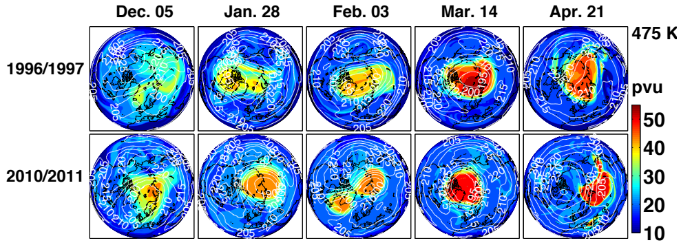
Figure 5.2: Temporal evolution of the polar vortex during selected days of the Arctic winters 1996/97 and 2010/11 at 475 K. The overlaid white contours are temperature in Kelvin.
