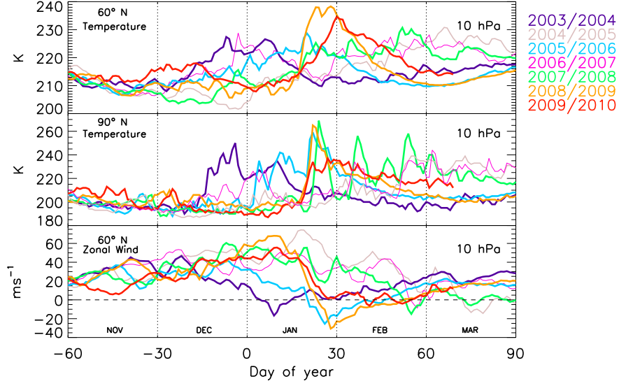
Figure 2.1: Temporal evolution of the zonally averaged temperature and zonal wind in the ECMWF operational analysis for the Arctic winters 2003/04–2009/10. The dashed horizontal line represents 0 \text{ ms}^{-1} and the dotted vertical lines separate each month.
