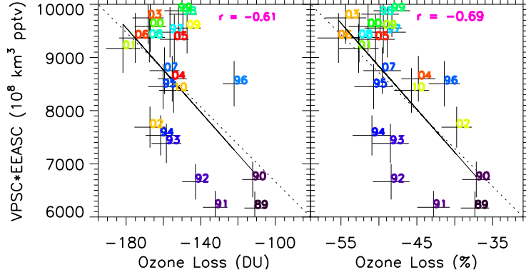
Figure 7.6: The correlation between ozone loss estimated from ground-based measurements (Table 7.1) and the product of V_{PSC} and EEASC. The V_{PSC} are calculated from the ECMWF operational analyses for the period 1989–2010.
