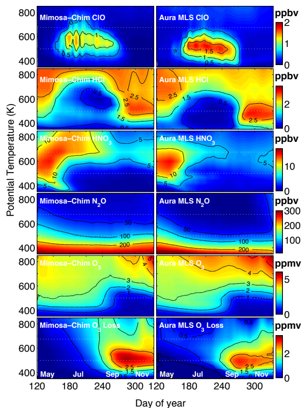
Figure 8.6: The vortex averaged ( \geq 65^\circ EqL) vertical and temporal evolution of CIO, HCl, HNO 3 , N 2 O, O 3 and ozone loss from the MIMOSA-CHIM model and MLS measurements. The data are the average of seven Antarctic winters 2004–2010 and are smoothed for 7 days.
