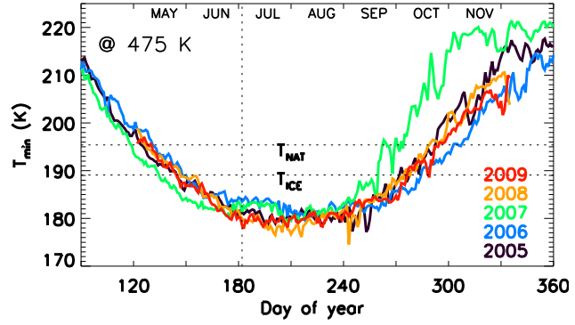
Figure 6.7: ECMWF daily minimum temperatures extracted over 50–90° S at 475 K for 2005–2009. The horizontal lines represent the T_{\text{NAT}} and T_{\text{ICE}} . The dotted vertical line represents 1 July.
