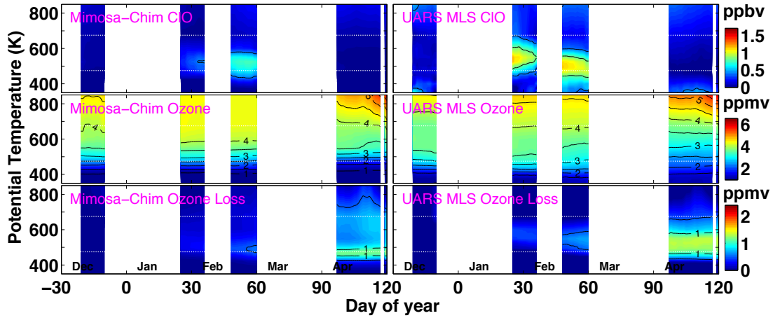
Figure 5.4: Temporal evolution of the vertical distribution of ClO, O 3 and ozone loss from MIMOSA-CHIM and UARS MLS for the Arctic winter 1996/97. The model fields are sampled at the location of MLS observations for each measurement inside the vortex and then averaged for the corresponding day. Both measurements and model data are smoothed for seven days. The model and MLS ClO coincident profiles are selected for SZAs <89° and local time between 10 and 16 h. The MLS ClO profiles are bias corrected. The white dotted lines represent 475 and 675 K.
