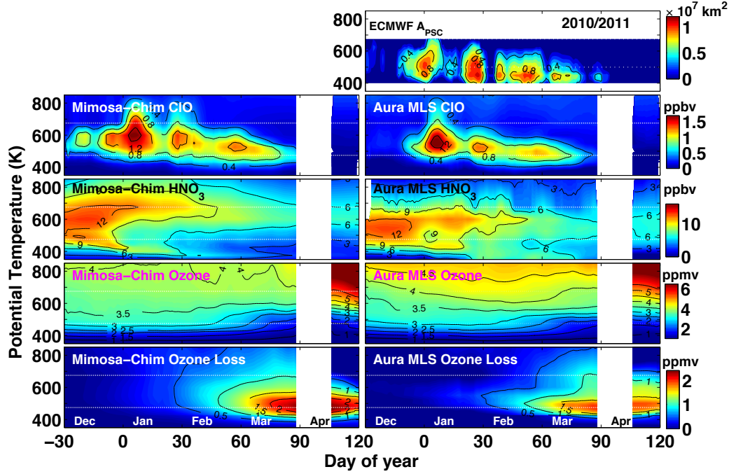
Figure 5.5: Temporal evolution of the vertical distribution of CIO, HNO 3 , O 3 and ozone loss from MIMOSA-CHIM and Aura MLS for the Arctic winter 2010/11. The model fields are sampled at the location of MLS observations for each measurement inside the vortex and then averaged for the corresponding day. Both model results and measurements are smoothed for seven days. The model and MLS CIO coincident profiles are selected for SZAs <89° and local time between 10 and 16 h. The MLS CIO profiles are bias corrected (see text). The A PSC computed from the ECMWF operational analyses is also shown (top panel). The white dotted lines represent 475 and 675 K.
