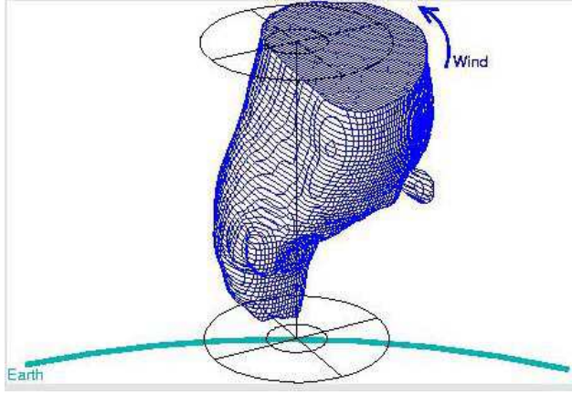
Figure 1.4: A three dimensional view of the Arctic vortex in the 2003/04 winter (image courtesy: JPL/NASA).
