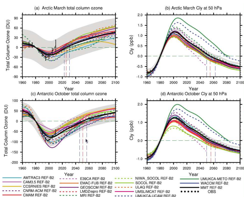
Figure 3: Multi-model simulations and projections of stratospheric ozone and \text{Cl}_y from the recent chemistry-climate model validation exercise (SPARC, 2010). Each model result is represented by different line styles and colour codes, the average of the model results is noted by MMT, and the observations are represented by OBS.
