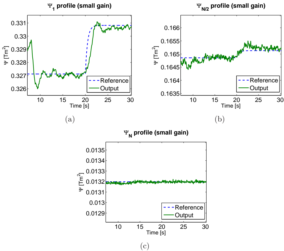
Figure 3.6: Regulation around \bar{\psi} with LMI controller with a more restricted gain than in Figure 3.5 (plain line: numerical simulation, dashed line: the reference). (a) Evolution and reference of the state \psi_1 ; (b) evolution and reference of the state \psi_{N/2} ; (c) evolution and reference of the state \psi_N .
