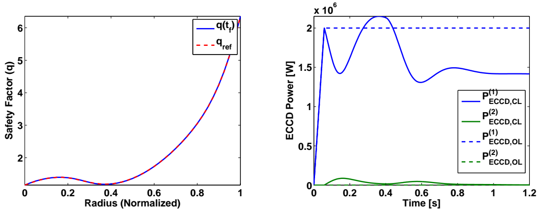
(b) Final safety factor profile and reference. (c) Applied ECCD power and open-loop reference value.
