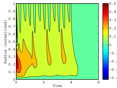
Figure B.9: Contour plot of the evolution of the state with disturbance acting until t = 4 s and time-varying diffusivity.
