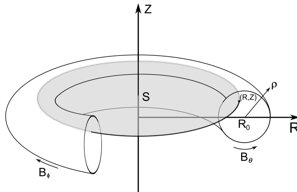
Figure 2.1: Coordinates (R, Z) and surface S used to define the poloidal magnetic flux \psi(R, Z) .
