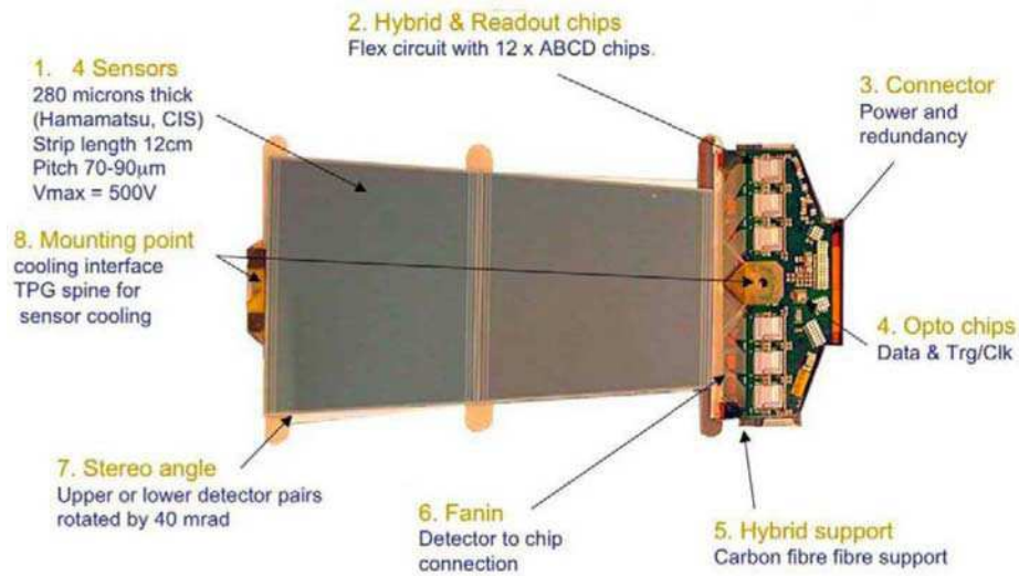
Figure 3.6: One of the types of SCT endcap modules [101].
