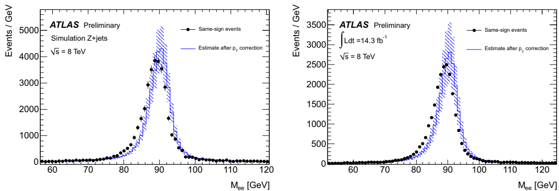
Figure 7.9: Closure test on simulated Z \rightarrow e^+e^- (left) and data (right) events. The black circles show the distribution of same-sign events while the blue histograms show the distribution of the reweighted opposite-sign events. The distributions are not expected to overlay exactly, due to the loss of energy of the trident electrons for the same-sign peak.
