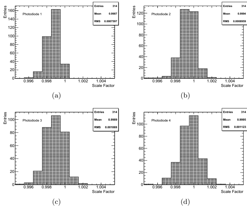
Figure 4.37: Distributions of the scale factors of the photodiodes 1 (a), 2 (b), 3 (c) and 4 (d) for all the alpha scans in the period D.
