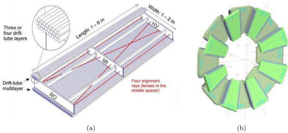
Figure 3.14: a) Mechanical structure of a MDT chamber showing the multilayers and the alignment system. b) Layout of a CSC endcap showing the eight small and eight large chambers [4].
