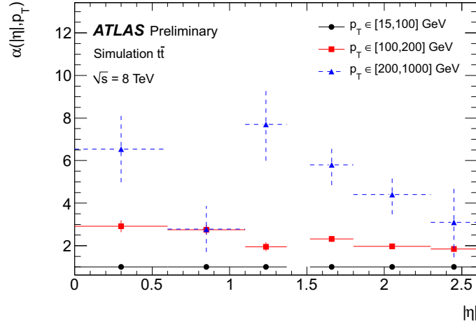
Figure 7.7: Correction factor \alpha(|\eta|, p_T) = \epsilon(|\eta|, p_T) / \epsilon(|\eta|, p_T < 100 \text{ GeV}) for t\bar{t} events computed by truth-matching, as a function of |\eta| and for different p_T bins. By definition, the correction factor is 1 in the first p_T bin.
