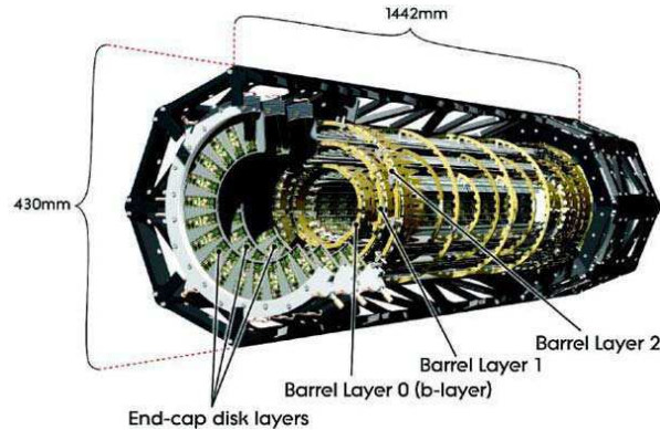
Figure 3.4: A schematic view of the active region of the pixel detector consisting of barrel and end cap layers.
