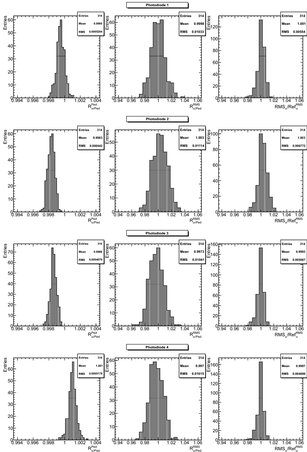
Figure 4.9: Distributions of the ratios R_{\alpha/Ped}^{Ped} (left), R_{\alpha/Ped}^{RMS} (center) and RMS_{\alpha}/Ref_{\alpha}^{RMS} (right) for the period D for the photodiodes 1, 2, 3 and 4, from top to bottom, respectively.
