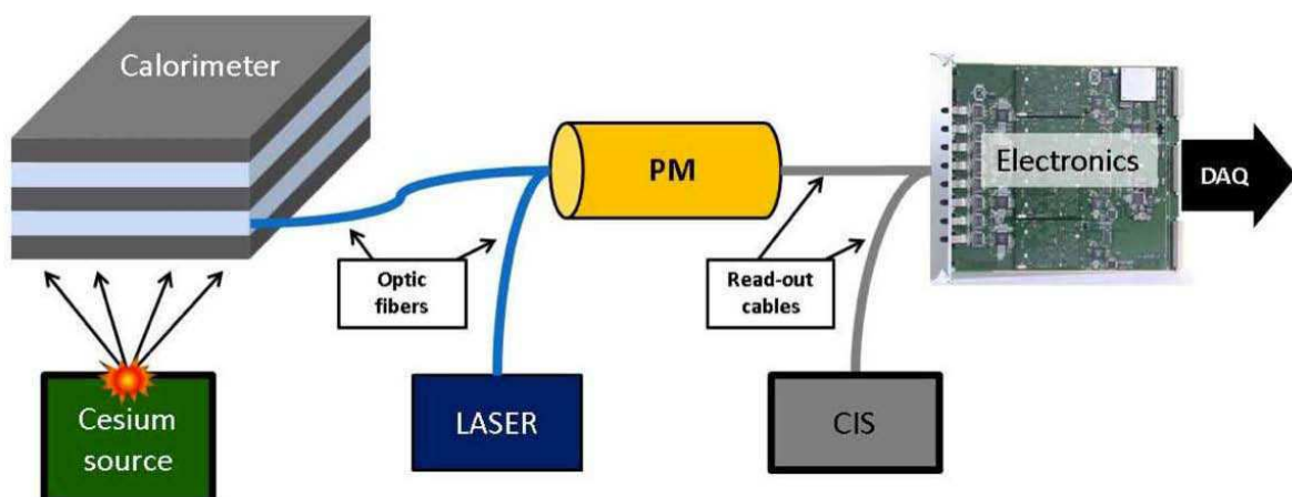
Figure 4.1: Hardware calibration chain of ATLAS TileCal.
