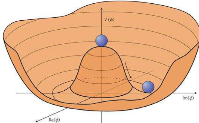
Figure 1.1: The Higgs potential as a function of \Phi in the plane \mathcal{R}(\Phi) - \mathcal{I}(\Phi) for \mu^2 < 0 and \lambda > 0 [43].
