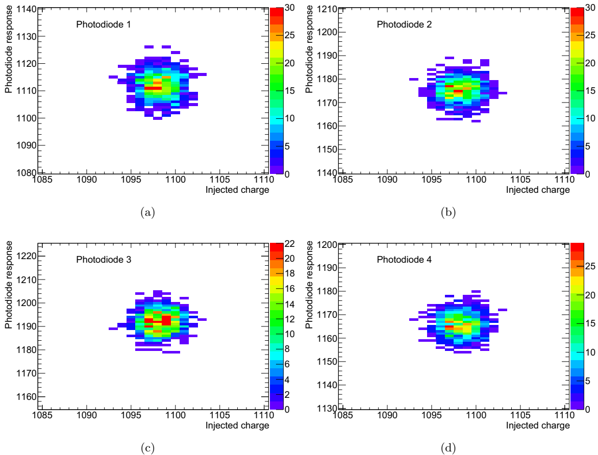
Figure 4.14: Response of the photodiodes electronics versus the injected charge for the photodiodes 1 (a), 2 (b), 3 (c) and 4 (d), in the single charge injection mode after pedestal subtraction.
