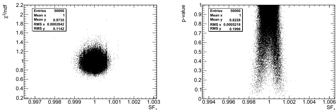
Figure 4.22: \chi^2/ndf (left) and p-value (right) as a function of the best scale factor found SF_1 for each simulated alpha scan. These values have been computed using the \chi^2 test and the Kolmogorov test, respectively. In this example SF_0 = 1 .
