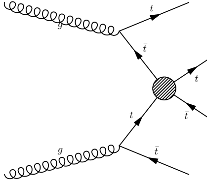
Figure 1.6: Feynman diagram example illustrating the production of four top quarks via contact interaction.
