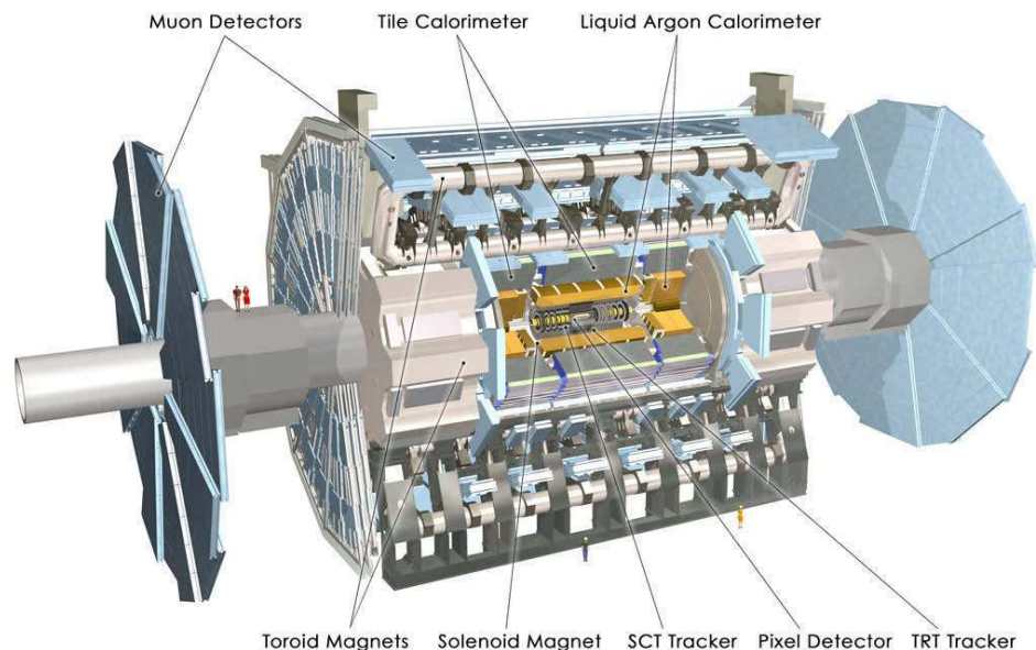
Figure 3.1: The Atlas detector.
