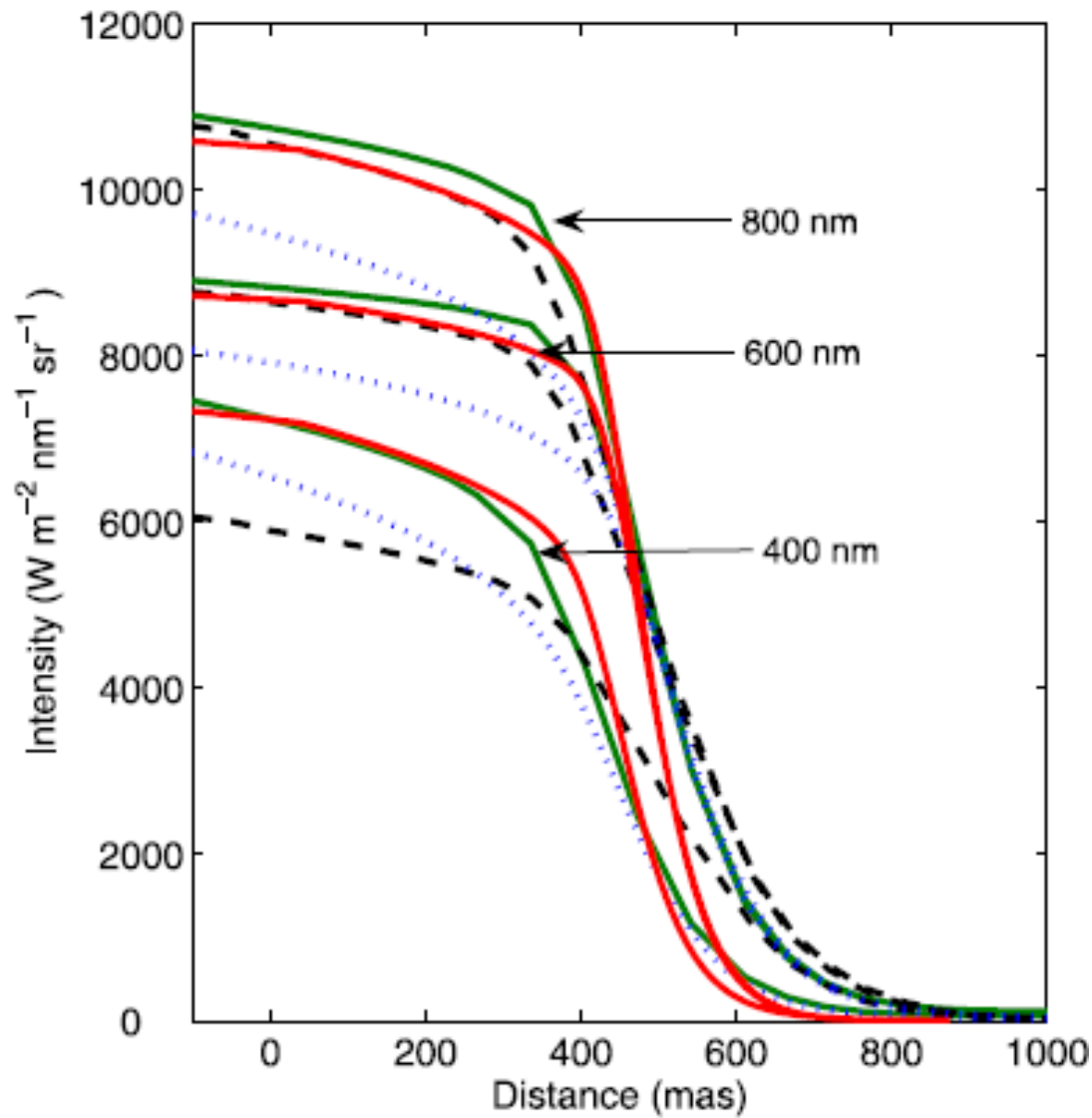
Figure 9 Limb shapes for three wavelengths predicted by SH09 (red), FCH09 (black), VAL-C (blue), and COSI (green) for 400, 600, and 800 nm.
