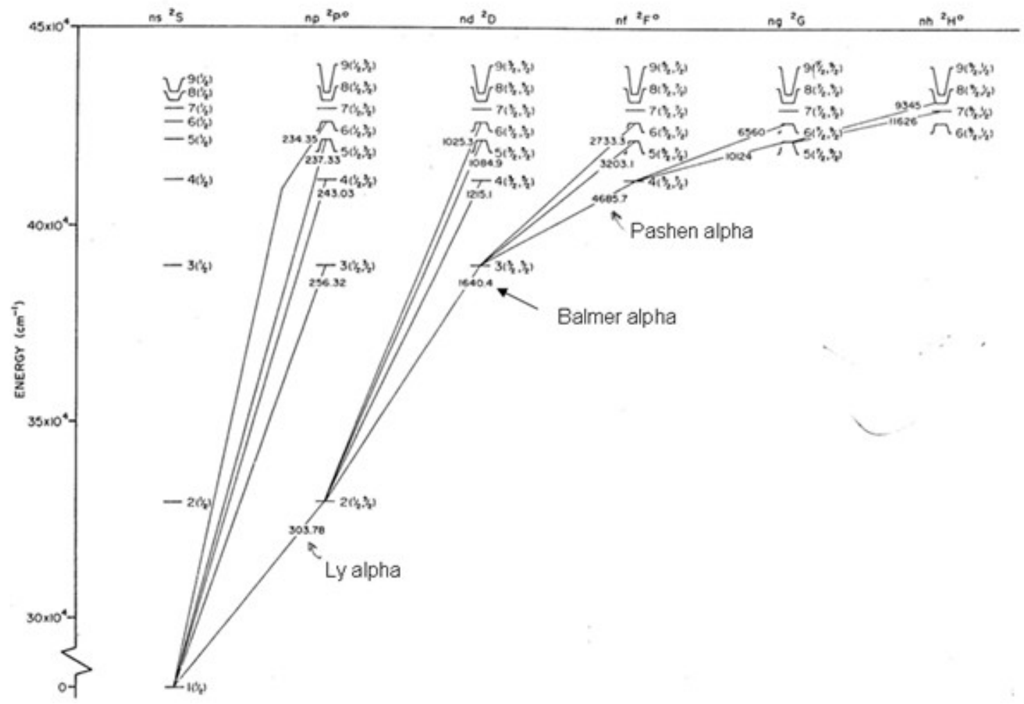
He II GROTRIAN DIAGRAM (1 electron, Z=2) (HI sequence, Configuration: n1)
