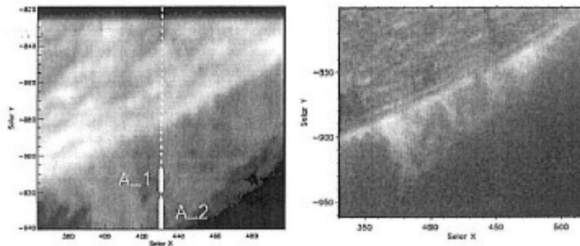
Fig. 1. Left: H-Lyman \beta image of the prominence obtained by rastering the area with the SUMER slit. The position of the spectrometer slit used is marked at the centre of the raster by the dashed line. The two white thick segments, named A_1 and A_2, mark the two portions of the slit used for the present analysis (see text). Right: the same prominence, but on a different scale, in a Big-Bear Solar Observatory H- \alpha image obtained on 8 October 1999. On this image we can see the whole extent of the feature.
