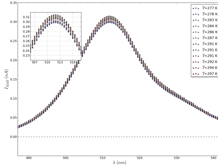
Figure 4.20: Spectra of the green LED05 ( \langle \lambda_p \rangle = 512 \text{ nm} ). This spectrum shows a small bump at high wavelength, but in that case, due to a too few current, the LED works at sub-regime and shows an increase of the the measured current I_{NIST} as the temperature increase. The wavelength is almost not shift along all temperatures range.
