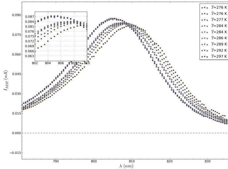
Figure 4.23: For spectra of the near-IR LED10 ( \langle \lambda_p \rangle = 810 \text{ nm} ) the behaviour is similar to the red LED07 shown on figure 4.22.
