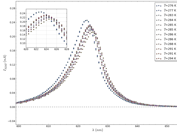
Figure 4.22: Spectra of the red LED07 ( \langle \lambda_p \rangle = 625 \text{ nm} ). In that case not only the flux decrease, but it is evident that the all the spectrum shift with its central wavelength.
