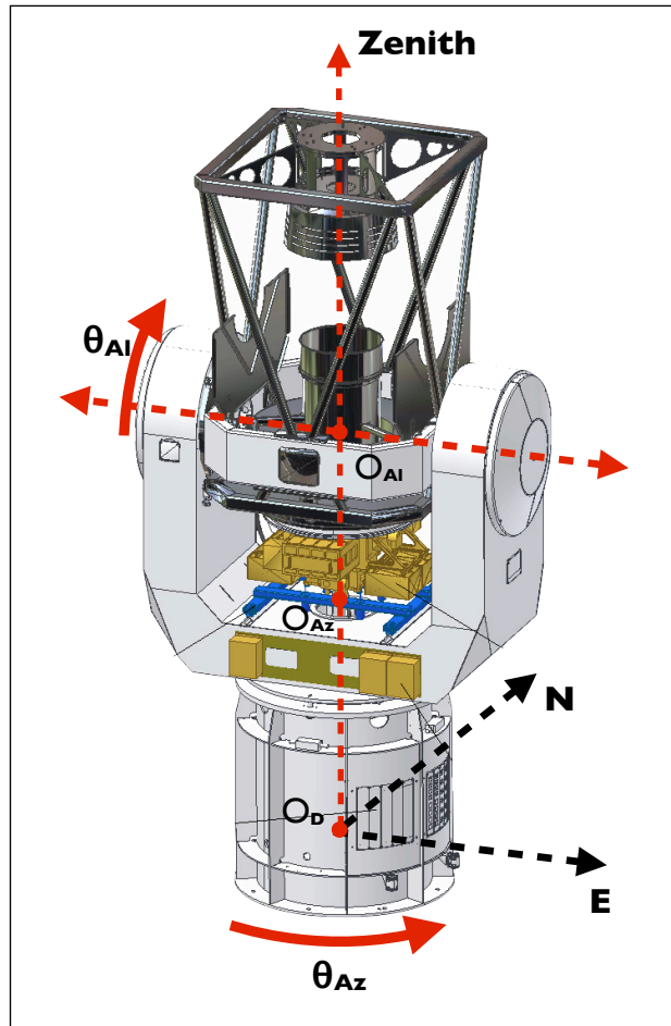
Figure 7.7: Origins and main reference frames for the telescope mount and primary mirror ( O_{Al} , O_{Az} ), and for the dome position O_D .
