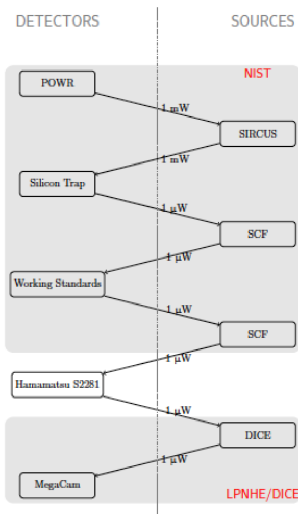
Figure 2.6: NIST metrology chain (Regnault 2013).
