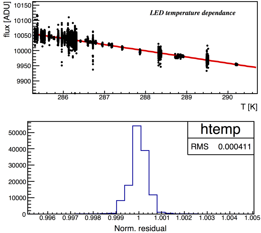
Figure 5.1: (Up) - The plot shows the dark corrected flux contribution of the LED23 ( \langle \lambda_p \rangle = 464 \text{ nm} ), as a function of the temperature measured by the Lakeshore-probe. The response is linear over all range of measured temperatures. The flux variations are due to readout noise coming from the not perfect shielded Keithley-NIST connection and from electromagnetic interference generated inside the cable. (Bottom) - This figure shows the residual distribution from the linear law fit (red line). Here the RMS represents the relative uncertainties and its value is \sim 4 \cdot 10^{-4} .
