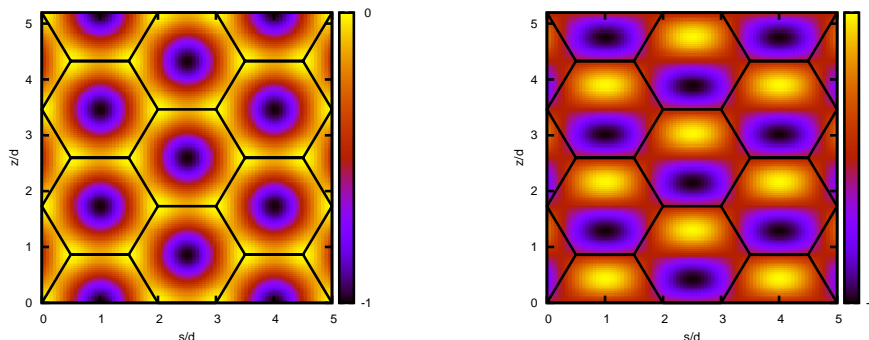
Figure 25: Potential landscape V(s, z) (left) and its derivative \partial_z V (right) for one oxygen atom at the distance \sigma of a graphene plane (distances are normalized by the C-C-distance d = 0.142 nm)
