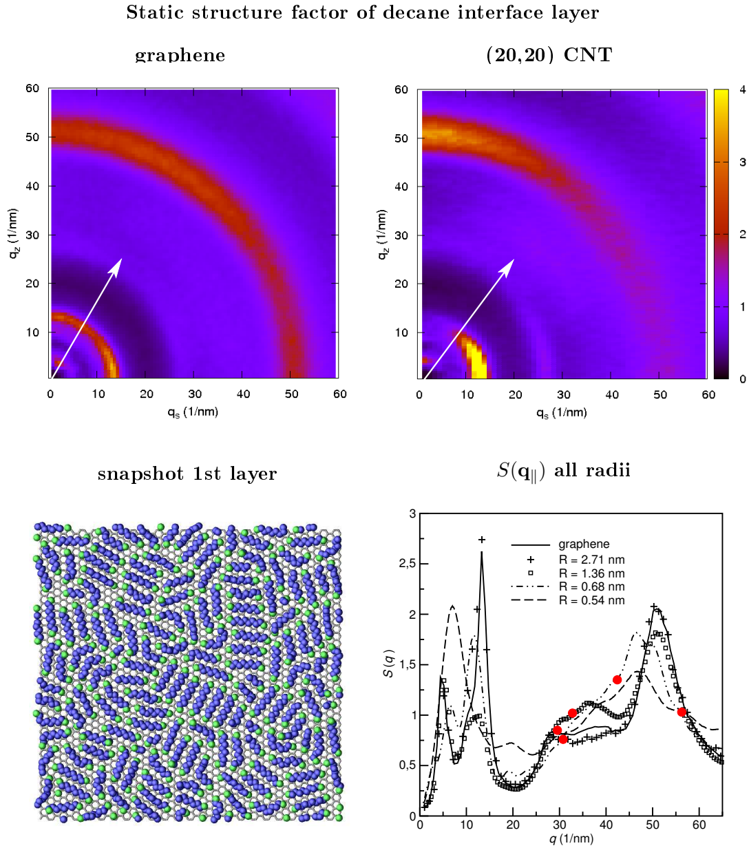
Figure 46: First liquid layer for decane/graphite interfaces. Lower left: The rod-like decane molecules adhere parallel to the wall and build a liquid layer of molecular thickness. Upper: 2-dimensional static structure factor of the interface decane layer on graphene ( upper left ) and in a CNT with radius 1.36 nm ( upper right ). For decreasing tube diameter, the decane molecules align more and more in the direction of the tube axis, and the structure factor gets anisotropic. Lower right: Static structure factor of all considered decane/graphite systems in direction of the wave vector \mathbf{q}_{\parallel} determining the periodic liquid/wall potential. Due to the developing anisotropy, S(\mathbf{q}) changes drastically with the radius. Furthermore, length and direction of \mathbf{q}_{\parallel} are radius-dependent (white vectors). This leads to an unsystematic curvature dependence of the commensurability factor S(\mathbf{q}_{\parallel}) (marked with the red dots). Note that the displayed structure factors are the ones for the \text{CH}_2 -pseudo-atoms (blue blobs in the snapshot); two characteristic lengths appear in the SF, the intramolecular bond length, and the distance between two parallel aligned decane molecules.
