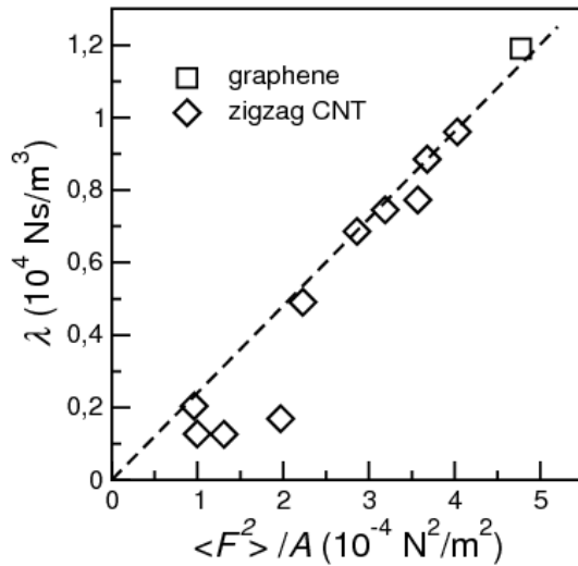
Figure 34: The friction coefficient \lambda is proportional to the rms force \langle F^2 \rangle / \mathcal{A} in the low confinement regime ( R > 1 nm). For smaller radii, confinement effects influence the water dynamics and via the decorrelation time of the force autocorrelation function also the friction coefficient \lambda = \beta \tau_F \langle F^2 \rangle / \mathcal{A}
