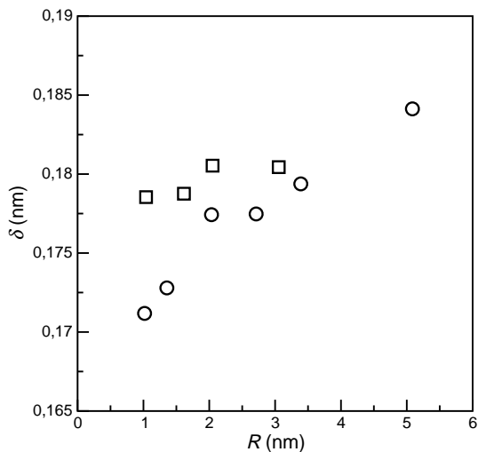
Figure 19: Depletion length of water in graphene slabs of size H = 2R (□) and of water in CNT with radius R (○) - according to the definitions Eq. (22) and (23). Note the small variation of \delta over the range of diameter studied.
