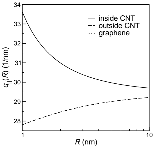
Figure 29: Radius dependence of the absolute value of the wave vectors |\mathbf{q}_+| = |\mathbf{q}_-| = q_{||} . \mathbf{q}_{\pm} are the reciprocal lattice vectors defining the periodicity of the water-carbon potential for a water molecule in the first layer near a graphitic wall. They change with curvature since bending the wall leads to a deformation of the potential landscape for water in its proximity. Inside or outside CNT, the periodicity of the energy landscape for water in the first layer is given by the projection of the carbon structure on the first layers position. q_{||} increases with curvature for water inside and decreases for water outside an armchair CNT.
