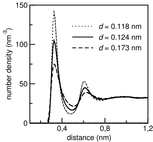
Figure 31: Water density profile in proximity of different 'artificial' graphene walls for constant temperature T = 300 \text{ K} and pressure p = 1 \text{ atm} . The carbon wall atoms are organized in a honeycomb lattice in all three setups, but with different C-C distances d . The model value for real graphene is d = 1.42 \text{ \AA} . The layering effect of water at the graphene wall is stronger for higher carbon surface densities (shorter C-C distance).
