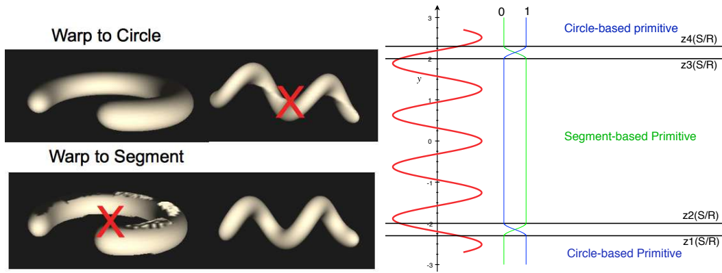
FIGURE 2.14 – Transition between the two kind of primitives in function of \frac{S}{R}
