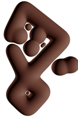
FIGURE 4.24 – Point with Inverse kernel of degree 3 and segment with Inverse kernel of degree 4 are used at the same time.
