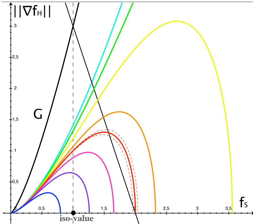
FIGURE 4.28 – Each colored graph correspond to the graph of (f_S, \|\nabla f_H\|) for the blending of two line skeleton in the plane situated at equal distance of each skeleton from a distance of 0 in cyan to a distance of 3.16 in blue (the equation of the curves are given in Appendix C.3). In red is the distance of 2 which corresponds to the tangential case between the two shapes to be bended : the inclined line leaving from (2, 0) , is the required direction of projection in order to obtain exactly the wanted iso-value in the point of null gradient in the tangential case. This figure emphasizes the facts that make us think that there exists a correction corresponding to our constraint to obtain a good blending : the colored graphs do not cross one another which means that we do not have contradictory constraint.
