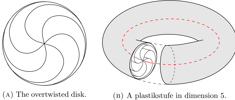
FIGURE 4. The easiest two examples of bLobS are the overtwisted disk, and a plastikstufe in a 5-dimensional contact manifold. In both of the pictures above, the objects do not quite correspond to the definition of the bLob , because the boundary is a closed Legendrian leaf. We can imagine that these models have been obtained by deforming the embedding in a neighborhood of the boundary using Proposition I.2.5.
