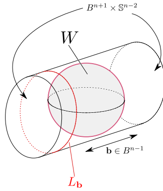
FIGURE 1. We find a family of Lobs by deforming the sphere to the boundary of a bi-disk. One of the two parts of the boundaries will then be foliated by Lobs.
