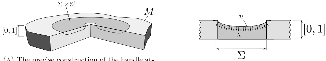
(B) The vector field X is tangent to the top face and transverse to the hypersurface \mathcal{H} , which is \Sigma pushed inside [0, 1] \times \Sigma relative to its boundary. Everything above \mathcal{H} has been discarded to make room for the handle.
