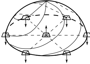
FIGURE 3. In dimension 3, it is well-known that we can get rid of 1-dimensional singular sets of a Legendrian foliation by slightly tilting the surface along the singular set. The figure depicts an overtwisted disk with singular boundary. By pushing the interior of the disk up keeping its boundary fixed, we obtain the standard form of an overtwisted disk whose boundary is a compact leaf of the foliation.
