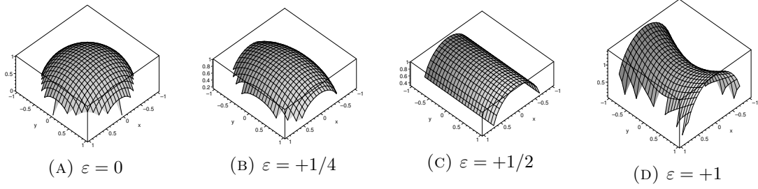
FIGURE 3. As a model situation, we study a 1-parameter family of pluri-subharmonic functions in \mathbb{C}^2 , and consider for each one the level set 1/2 . The surfaces represented here are the intersection of these level sets with the 3-dimensional slice \mathbb{C} \times \mathbb{R} . The induced Legendrian foliation for each of those intersections can be seen in Fig. 2.(A), and Fig. 2.(B) that correspond to the graph (A) and (B) respectively. The hyperbolic case in Fig. 2.(C) corresponds to graph (D). The holomorphic disks attached to these surfaces are just the subsets of the horizontal flat planes lying beneath these graphs.
