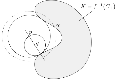
FIGURE 2. Constructing a disk that has a single maximum on its boundary.
