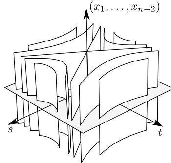
FIGURE 1. The singularities of a neat singular foliation look locally like the product of \mathbb{R}^{n-2} with a foliation in the plane. The directions \partial_{x_1}, \dots, \partial_{x_{n-2}} correspond to the secondary foliation associated to a contact form.
