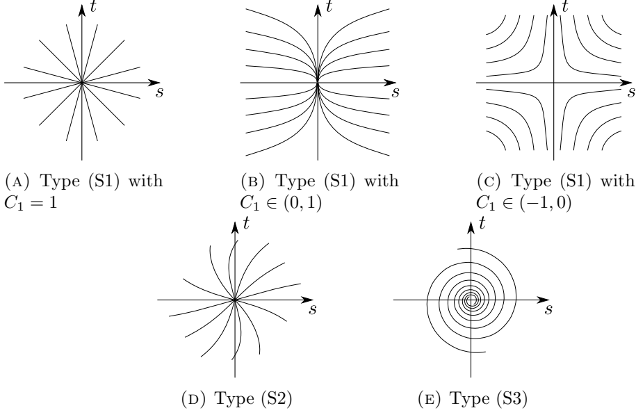
FIGURE 2. The linearized singularities correspond to one of the five possible cases sketched here (or to type (S1) with C_1 = 0 which we have omitted because the linearization does not necessarily correspond to the actual shape).
