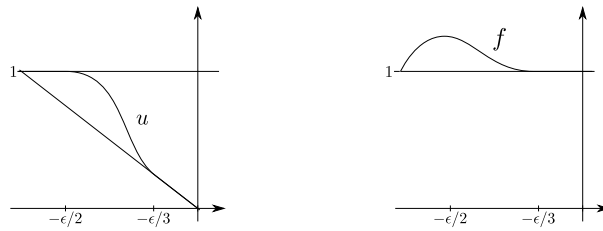
FIGURE 1. The functions u and f .
