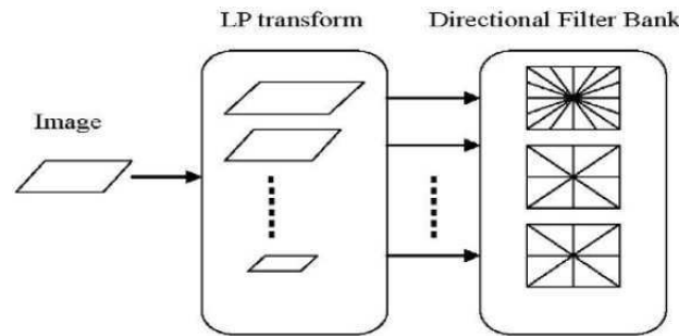
Figure 2.10 Framework of the contourlet transform.
