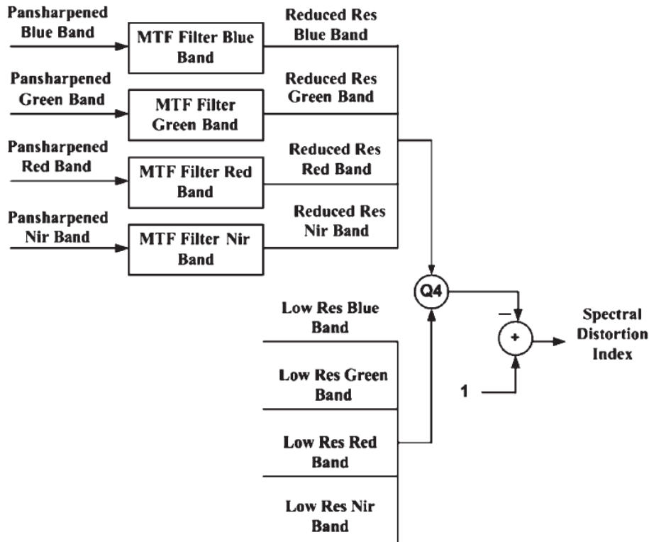
Figure 3.1 Flowchart of spectral quality assessment [101]
