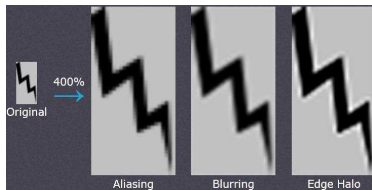
Figure 2.1 Interpolation artifacts 1
