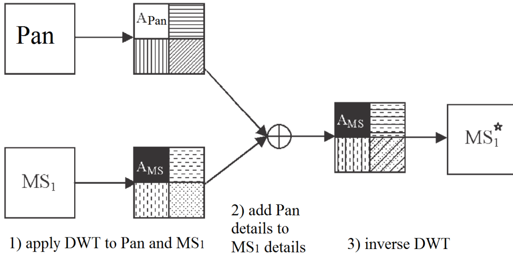
Figure 2.8 Fusion using a conventional DWT [129].
