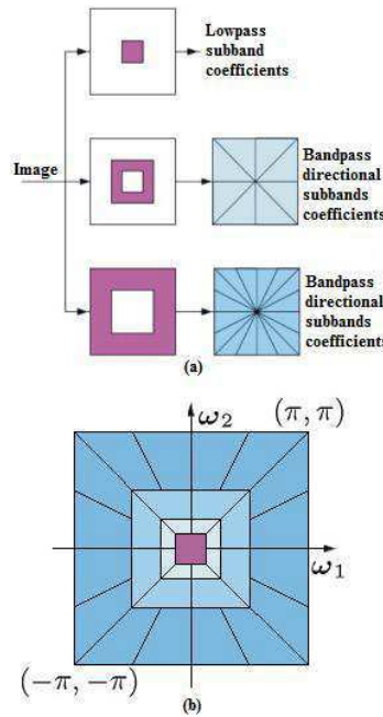
Figure 4.10 Nonsubsampling contourlet transform. (a) Implementation of NSCT. (b) Frequency partitioning in idealized form.
