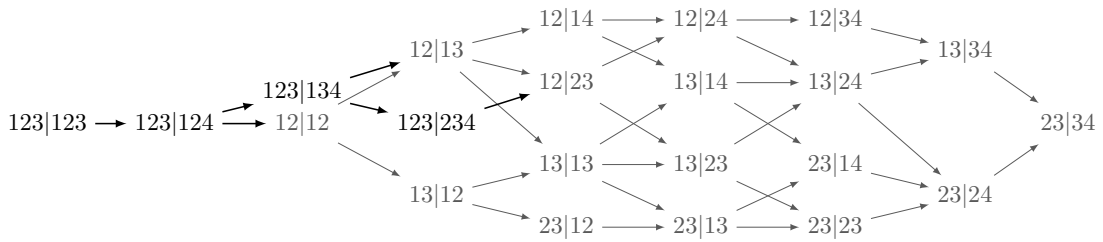
Figure 7.2: All chains consisting of the 2-minors and 3-minors.
