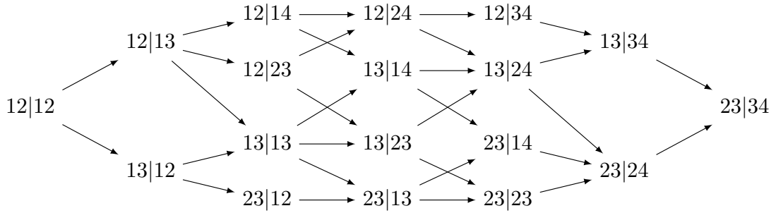
Figure 7.1: All chains consisting only of the 2-minors.
