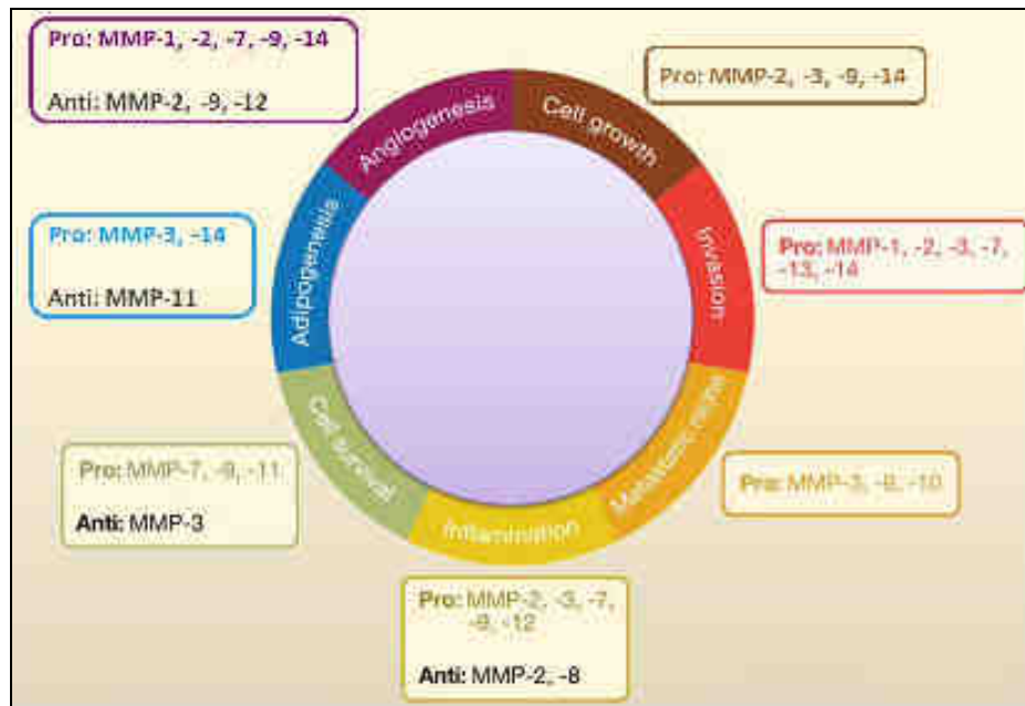
Figure 1.4 Modulation of the tumor microenvironment by MMPs. Summary of the various processes that are modulated by MMPs in the tumor microenvironment. Selected examples of MMPs that promote (pro) or suppress (anti) these processes. This image illustrates the complexity of the tumor microenvironment, which is largely influenced by MMPs. Modified from Kessenbrock, et al., 2010.
