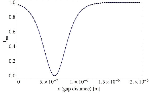
Figure 6.15: T_{\text{on}} as a function of gap distance x between disk and waveguide for a ( p=1 m=57 ) WGM with intrinsic optical Q \simeq 4 \cdot 10^4 . Black dots correspond to individual calculations of T_{\text{on}} by the overlap integral method described in chapter 1. The blue line is a fit using Eq. 6.4. Remarkably both are in very good agreement, even though they are derived by entirely different methods. For this WGM the critical coupling regime occurs around x=600 nm.
