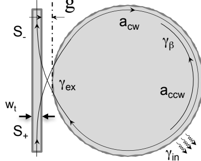
Figure A.1: Schematic illustrating the parameters used for the WGM doublet splitting description, where rough resonator sidewalls scatter energy between clockwise and counterclockwise propagating modes.
