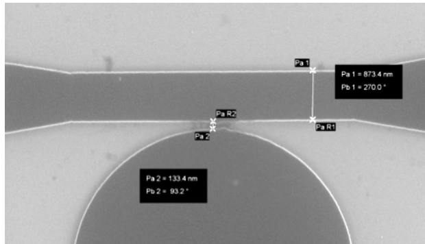
Figure 4.7: SEM micrograph of developed resist showing how non-optimal exposure parameters lead to proximity effects between disk and taper. The disk is 2.5 \mu\text{m} in radius, the waveguide is \sim 900 \text{ nm} wide at its thinnest and the gap between the two is roughly 100 \text{ nm} . Remaining resist residue is visible between the disk and the waveguide lending a grayish color to the area. Notice also the increased sidewall roughness in the portion of the disk resonator closest to the waveguide.
