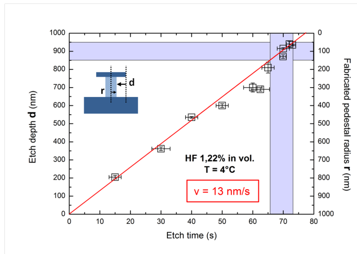
Figure 4.19: Derivation of the HF undercut speed at 4 °C. The solution consists of 2.5 mL of 50% concentration HF diluted in 100 mL DI water ( \Rightarrow 1.22 % HF in volume). The left axis represents the one-sided undercut depth d (see inset figure). The right axis gives the corresponding AlGaAs pedestal radius r , for a 1 \mu\text{m} radius disk. 70 \pm 3 s etch times reliably produce disk resonators with a pedestal radius of \sim 100 nm (blue target region) such as the one shown in Fig. 4.23. These etch speeds were measured for AlGaAs unexposed to air. Data acquired in the team by Dac Trung Nguyen.
