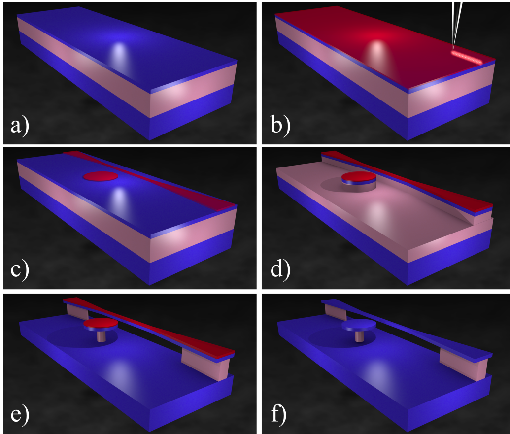
Figure 4.1: Main nano-fabrication steps. (a) The sample is composed from top to bottom of a 320 nm thick GaAs layer (blue) and a 1.8 \mu\text{m} thick \text{Al}_{0.8}\text{Ga}_{0.2}\text{As} sacrificial layer (beige) both epitaxially grown on a GaAs substrate. (b) Negative ebeam resist is spun on the sample and exposed using a focused electron beam (top right). (c) After the development step only the exposed resist remains on the sample. (d) The resist serves as an etch mask, protecting the disk and waveguide features during a non selective etch step through the top GaAs layer. (e) A dilute HF solution selectively under-etches the sacrificial \text{Al}_{0.8}\text{Ga}_{0.2}\text{As} layer. (f) The negative ebeam resist is removed yielding a finished device.
