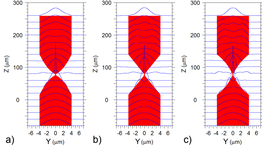
Figure 1.12: BPM comparison between the optical transmission of 3 different taper profiles: (a) calculated ‘optimal’ adiabatic (b) linear and (c) exponential. In red is the waveguide seen from the top, in blue the optical energy profile at different positions z along the guide. In all three cases \lambda=1.32 \mu\text{m} and the waveguide width is reduced from 8 \mu\text{m} to 200 \text{ nm} over a 60 \mu\text{m} tapering length. The power transmission is 96% for (a), 91% for (b) and only 86.6% for the exponential profile (c). Evidence of coupling to the second order mode is well visible in (b) and (c) at Z \simeq 40 \mu\text{m} .
