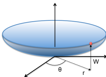
Figure 2.2: Deformation amplitude W of a point of the disk of coordinates r and \theta .
