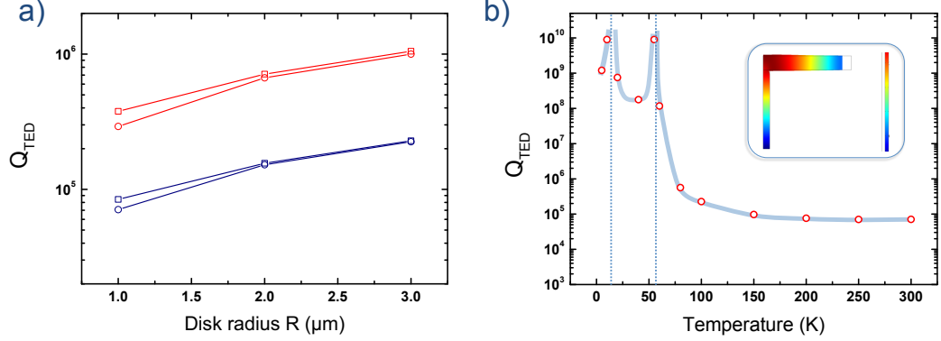
Figure 2.9: Thermoelastic damping. (a) FEM simulated values of Q_{\text{td}} for a 320 nm thick GaAs disk resonator with no AlGaAs pedestal (squares) and with a 150 nm radius pedestal (circles) as a function of the disk radius R , at room temperature. The red points are obtained using for GaAs the values \kappa = 33 \text{ W}/(\text{m}\cdot\text{K}) , c_p = 550 \text{ J}/(\text{kg}\cdot\text{K}) from [98]. The blue points use \kappa = 55 \text{ W}/(\text{m}\cdot\text{K}) , c_p = 327 \text{ J}/(\text{kg}\cdot\text{K}) from [84]. In both cases \alpha_{th} = 5.7 \cdot 10^{-6} \text{ K}^{-1} . (b) Dependence of Q_{\text{td}} with temperature ( T ) using the temperature dependent values \kappa(T) , c_p(T) and \alpha_{th}(T) from [84], illustrating the rise in Q_{\text{td}} at low temperature. The vertical dashed lines indicate the temperatures for which \alpha_{th}(T) changes sign: 56 K and 12 K [84]. The blue curve serves as a guide to the eye. The inset serves to illustrate the strain temperature (a.u.) during contraction of the breathing mode, red=hotter, blue=cooler.
