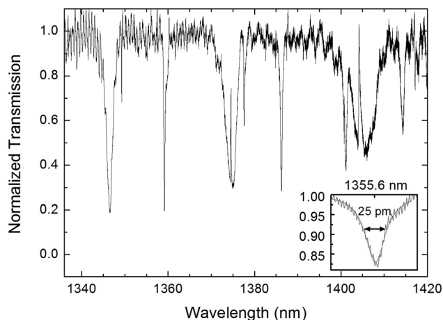
FIG. 2. Transmission spectrum of a suspended tapered waveguide coupled to a 7.4 \mu\text{m} diameter GaAs disk. Inset: a fine optical resonance at \lambda = 1355 nm, measured on another disk. The small amplitude oscillations in the base transmission correspond to Fabry-Perot fringes of the waveguide and are not noisy in nature.
