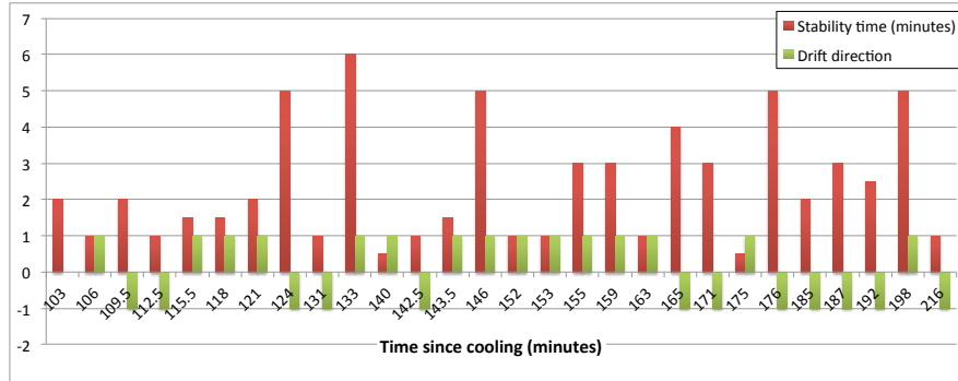
Figure C.2: This diagram illustrates the un-optimized setup’s coupling stability measured over the course of a three and a half hour period, underscoring the problem of thermal drift. The average time the setup stays coupled is under two and a half minutes. The green bar (which takes the value \pm 1 ) indicates the drift direction and illustrates the seemingly random nature of the process.
