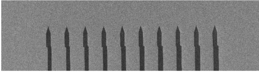
Figure 4.5: SEM micrograph displaying poor alignment between the tapered region of the waveguide (top) exposed in write-field mode with a 10\ \mu\text{m} column aperture and the straight segment of the coupling waveguide written in FBMS mode with a 60\ \mu\text{m} column aperture. Only half of the waveguides and no disks were exposed for this testing procedure. For scale each waveguide is \sim 10 micrometers in width.
