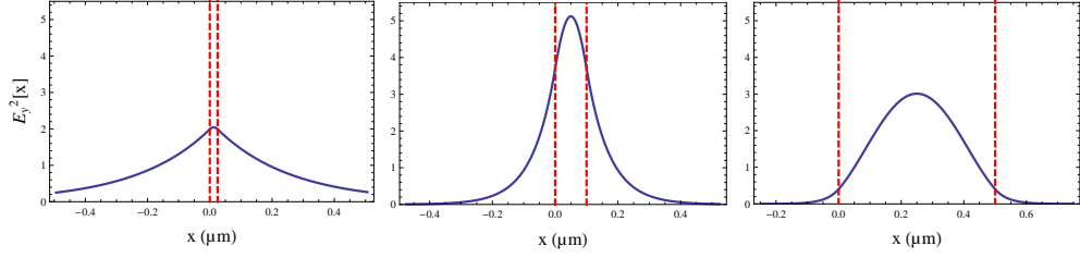
Figure 1.7: Plot of the transverse electric field squared ( E_y^2 ) for the fundamental guided mode of a GaAs slab for three distinct slab thicknesses : from left to right h=25 nm, h=100 nm and h=500 nm.
