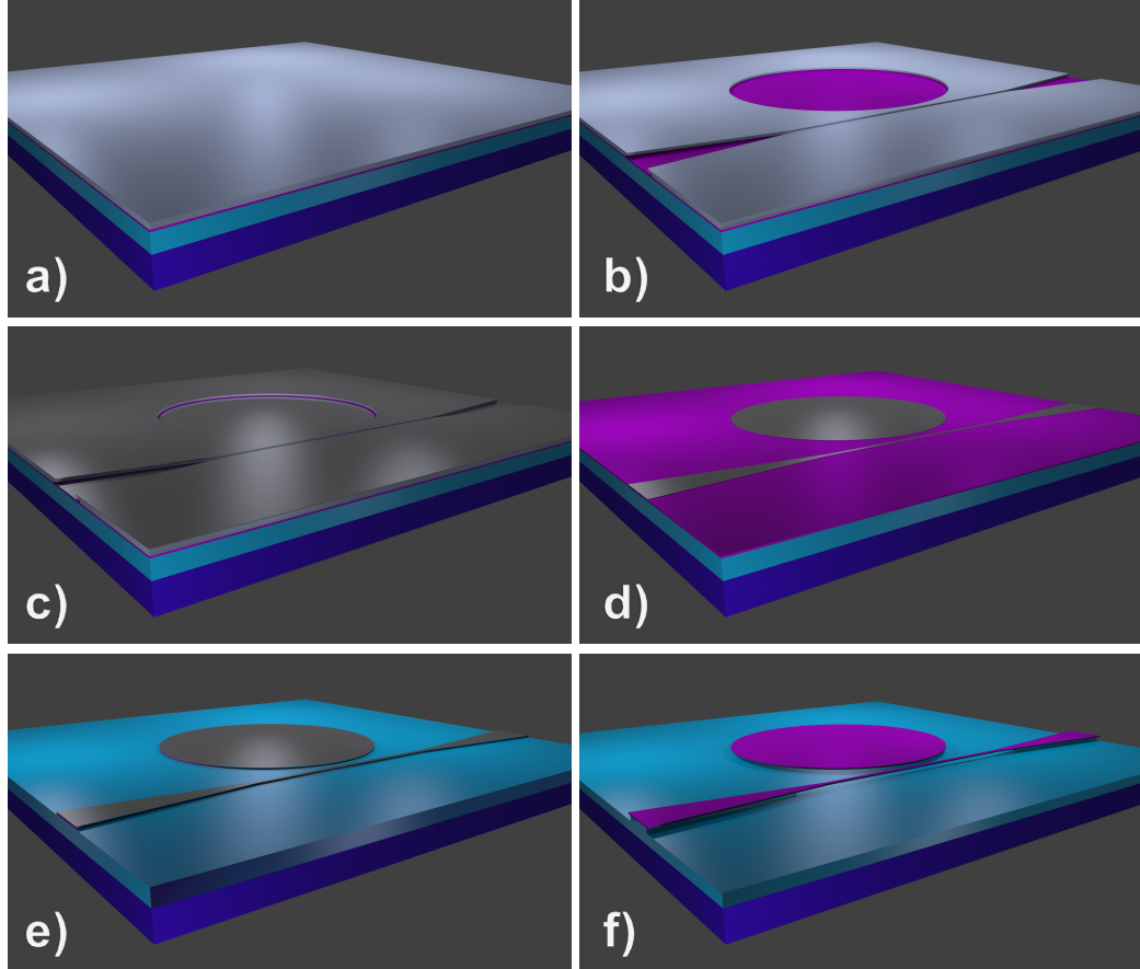
Figure 4.24: Main nano-fabrication steps. (a) The sample is composed from top to bottom of a 300 nm thick LPCVD silicon nitride layer (purple) over a 3 \mu\text{m} thick SiO 2 sacrificial layer (light blue) on top of a silicon substrate (deep blue). Two coats of PMMA (white) are spun and baked on the sample (see section 4.1.3). (b) The resist is exposed in the ebeam lithography system and developed : only the unexposed resist remains on the sample (see section 4.2.2). (c) A 40 nm thick cobalt layer is evaporated upon the entire sample. (d) A lift-off in warm acetone dissolves the PMMA and only leaves the cobalt etch mask in place (see 4.2.3). (e) The cobalt etch mask protects the disk and waveguide patterns during an ICP-RIE dry etch through the top SiN layer (see 4.2.4). (f) The cobalt is removed in Piranha etchant and the sacrificial SiO 2 layer is selectively under-etched using Buffered Oxide Etchant (BOE), isolating the SiN disk resonator on a SiO 2 pedestal and locally freeing the coupling waveguide (see 4.2.5).
