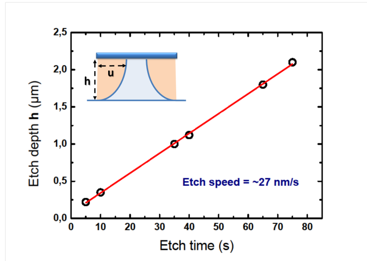
Figure 4.15: Determination the etch speed of the BCK etchant at 4^\circ\text{C} with no stirring. The etch depth h (see inset figure) is plotted as a function of time. We experimentally verify that the ratio of etch depth h to lateral undercut u is \sim 1.3 , in excellent agreement with the quantitative model of an ideal diffusion controlled etch profile [140].
