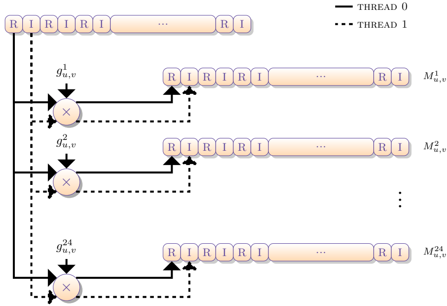
Figure 5.5: Two sample threads from a thread block for Gabor filter bank.
