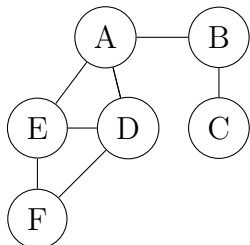
Figure 1.5: Graph example (G) with 6 vertices
