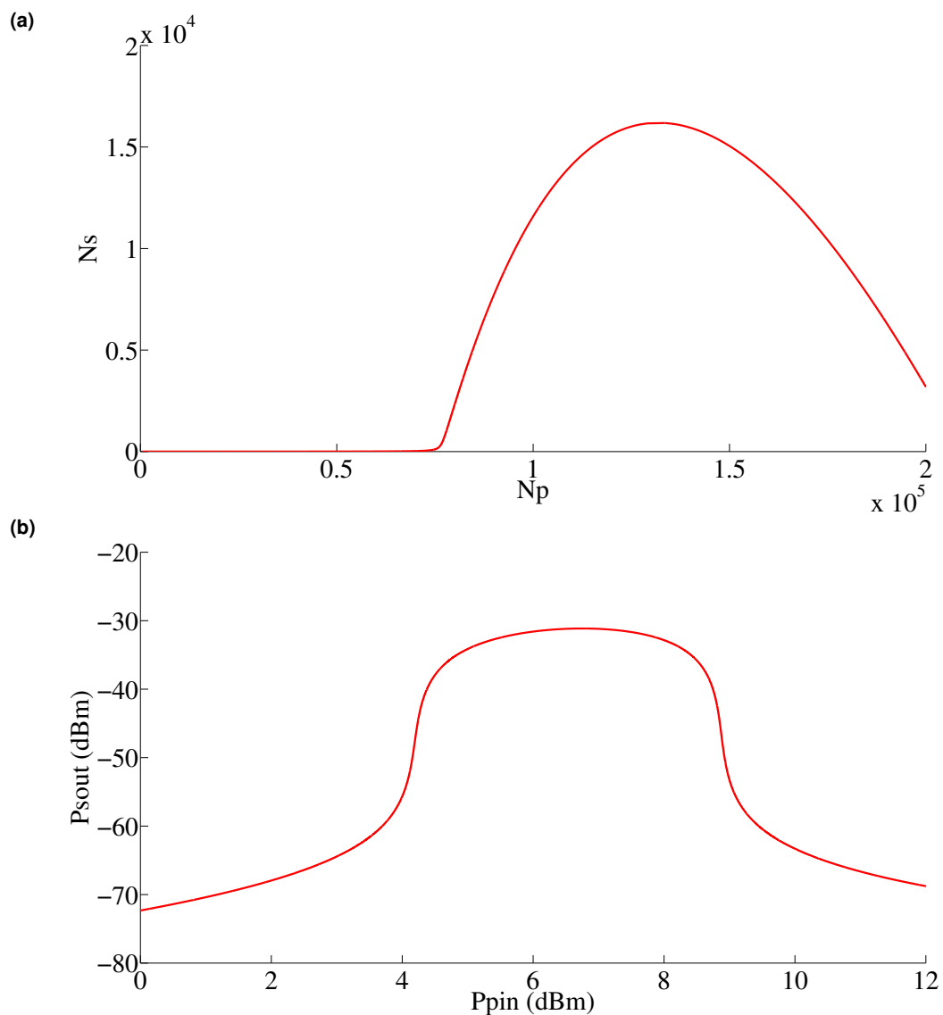
Figure 3.3: (a) The number of Stokes photons as a function of the number of pump photons. (b) The output Stokes power as a function of the input pump power. These curves were plotted using the typical parameters of the doubly resonant cavity we studied afterwards (see 3.3), taking \tau_{fc} = 0.3 ns for the free-carrier lifetime, Q_p = 4900 and Q_s = 235000 for the pump and Stokes quality factors, g_R^B = 30 cm/GW for the Raman gain in bulk silicon, and V_R = 2.78 \mu m^3 for the Raman volume.
