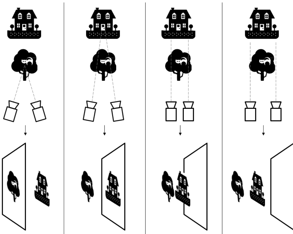
Figure 3.1: The toed-in and parallel camera configurations and the variations in the rendered depth relative to the screen plane in function of the dual-camera convergence angle and of the camera-base distance; adapted from [Mendiburu 2009] and [Sony 3D Television & Film 2010].
