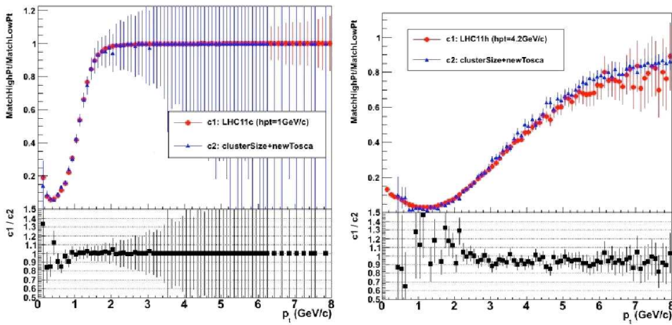
Figure 7.6: Comparison between data (red points) and simulations (blue points) of the Muon Trigger efficiency as a function of p_T for two sets of p_T cuts. Black points in the low panels represent the ratios of the two sets of points.
