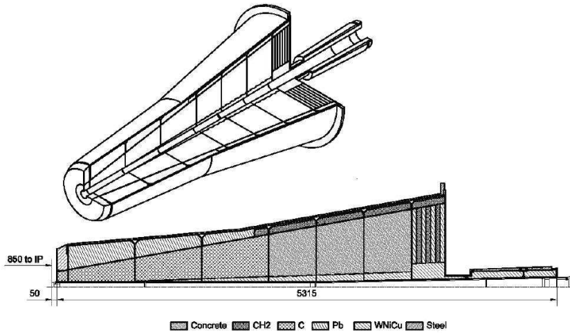
Figure 5.2: Design of the front absorber.
