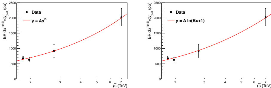
Figure 8.15: Energy dependence of the \Upsilon(1S) cross section at midrapidity, with overlaid power-law (left) and logarithmic (right) fit functions.
