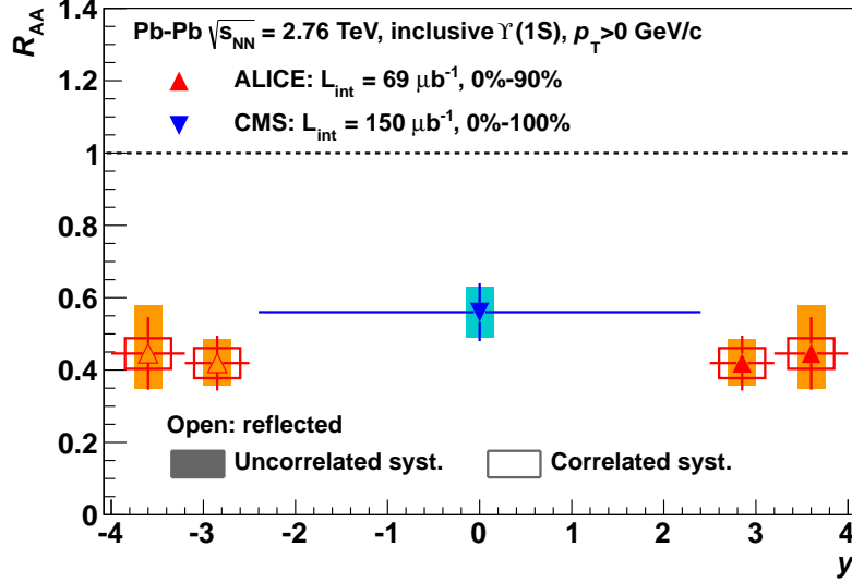
Figure 9.4: Comparison of ALICE and CMS \Upsilon(1S) inclusive R_{AA} as a function of the rapidity.
