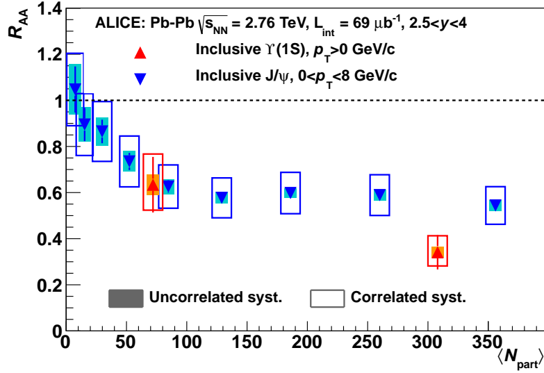
Figure 9.1: Comparison of ALICE \Upsilon(1S) and J/\psi inclusive R_{AA} in the same kinematic window as a function of the average number of participants.
