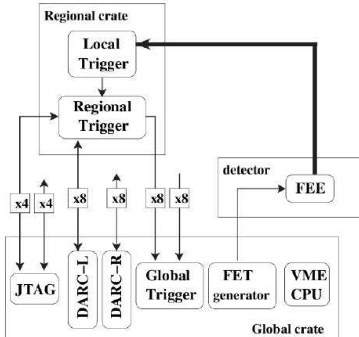
Figure 5.12: Schematic design of the Muon Trigger electronics.
