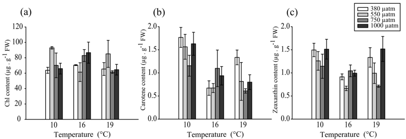
Figure 7 : Chlorophyll compounds (a), carotene (b) and zeaxanthin (c) contents in the four p\text{CO}_2 treatments at 10^\circ\text{C} , 16^\circ\text{C} and 19^\circ\text{C} . Results are expressed by mean \pm standard error, n = 3 (or 6).
