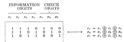
Figure 4.1: Codes "parity check".
