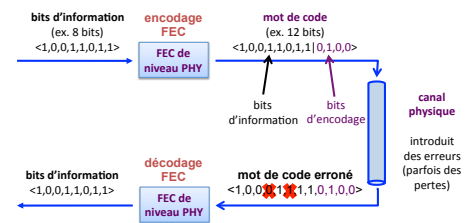
Figure 2.1: Codes FEC de la couche PHY.
