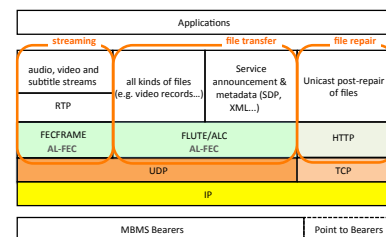
Figure 1.2: Pile protocolaire des services 3GPP/MBMS.
