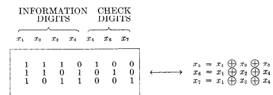
Figure 4.1: Codes "parity check".
