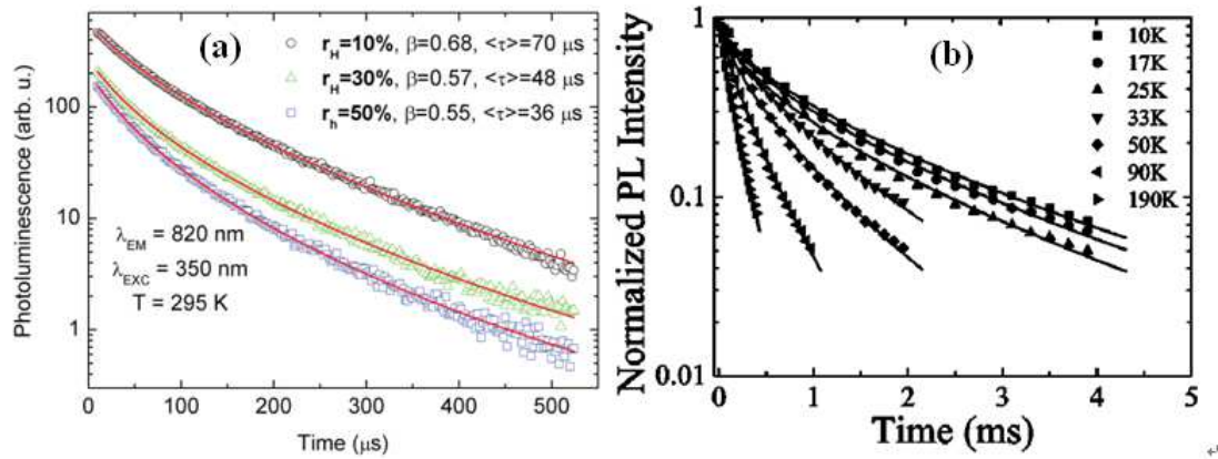
Figure 1.3: Non-single exponential PL decays measured (a) at room temperature for samples fabricated by reactive magnetron sputtering [37] ; and (b) at the indicative temperatures for sample containing 18 at.% Si excess [38] .
