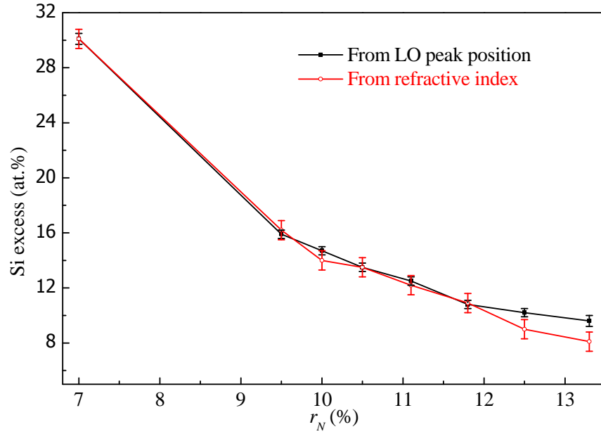
Figure 4.3: Si excess evolution versus r_N with experimental error bars for classical co-sputtered samples. The Si excess values have been deduced from FTIR and ellipsometric measurements.
