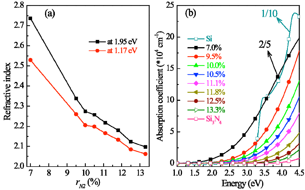
Figure 4.2: For as-deposited layers, (a) refractive index evolution as a function of the nitrogen rate r_N for two energies, 1.17 and 1.95 eV; (b) absorption coefficient versus energy from 1.0 to 4.5 eV for different r_N investigated and pure \text{Si}_3\text{N}_4 and Si layers.
