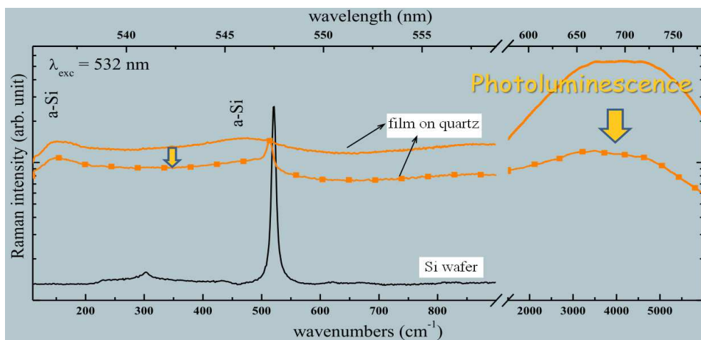
Figure 2.10: Raman spectra of Si wafer (black curve), 750°C-annealed (orange curve) and 1100°C-annealed (orange square) SRSN layers deposited on quartz.
