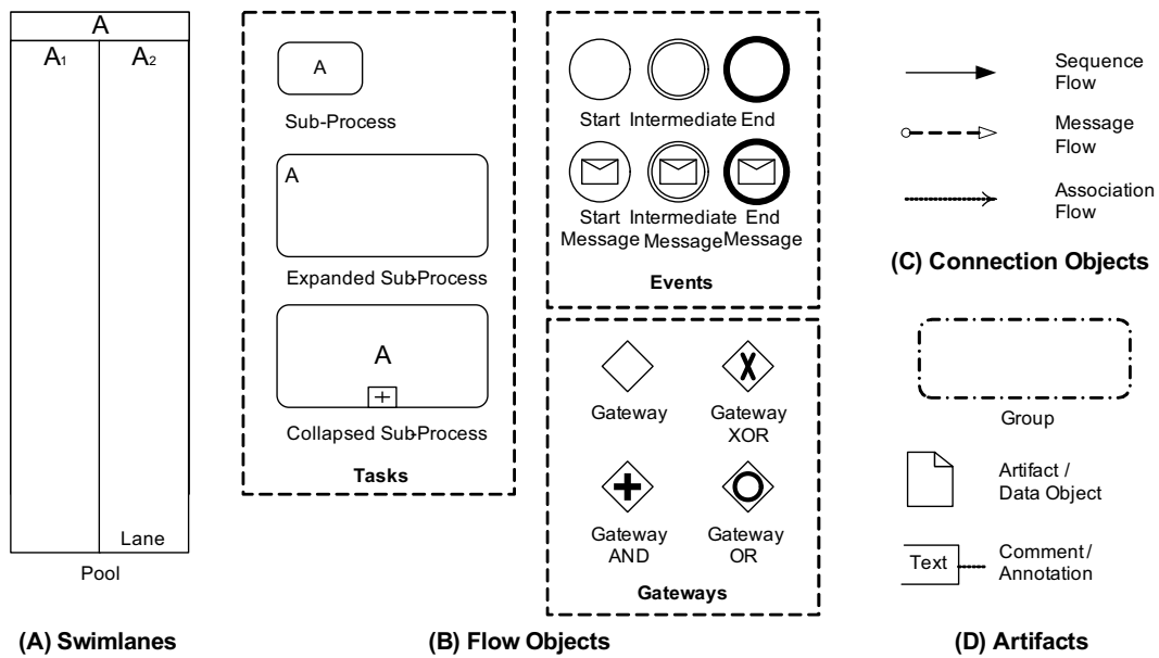
Fig. 2.6: Graphical notation for core set of BPMN elements
