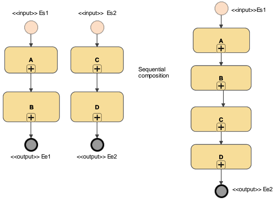
Fig. 7.1: Sequential composition operator for business process fragments
