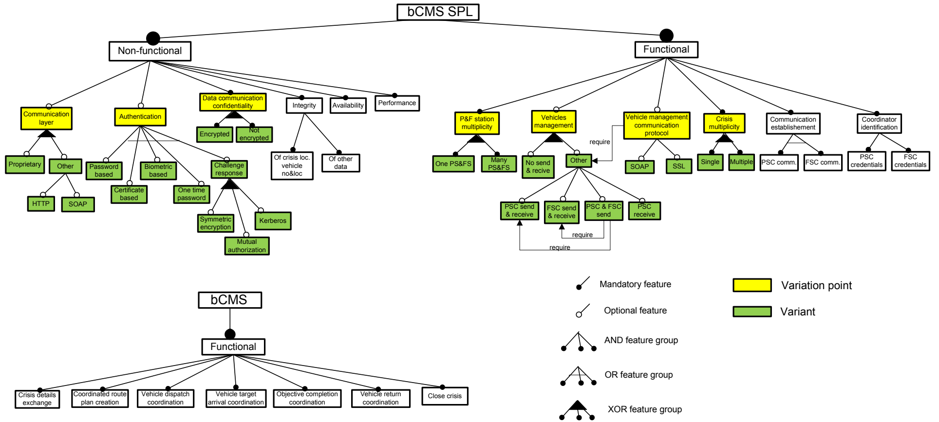
Fig. 6.3: Complete feature diagram of the bCMS system
