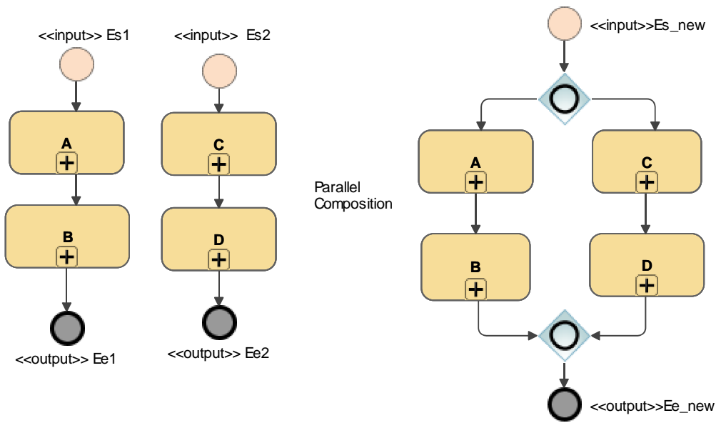
Fig. 7.4: Choice composition operator for business process fragments
