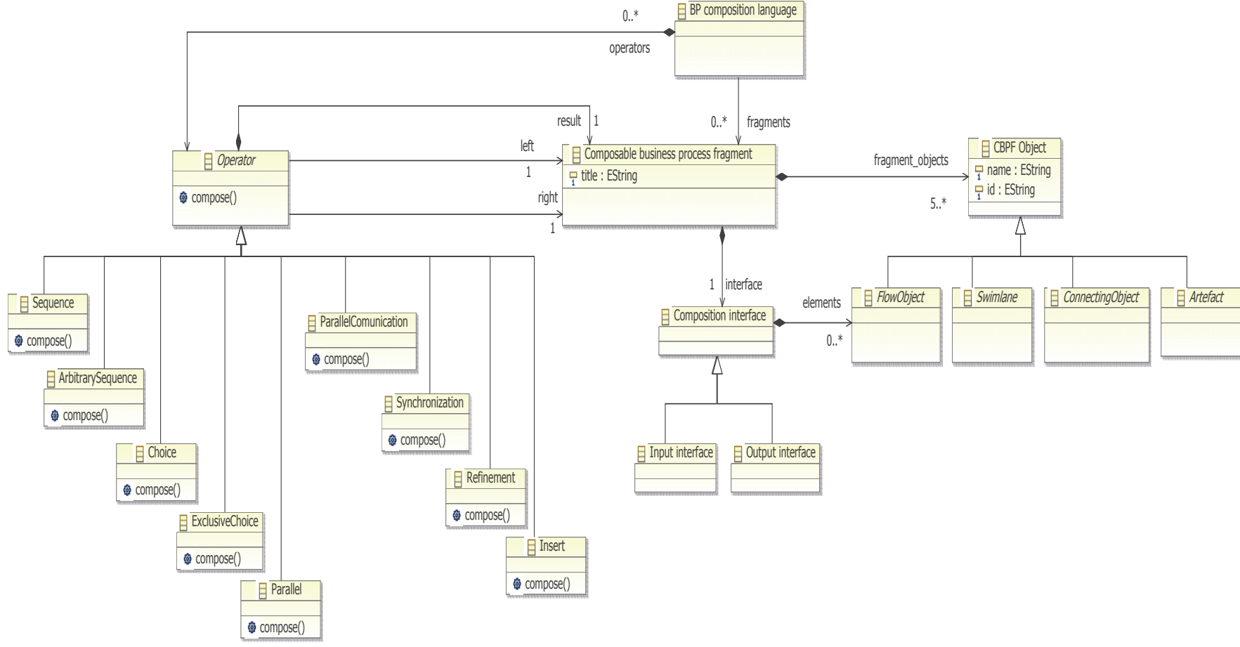
Fig. 4.8: Excerpt of language meta-model: composition operators
