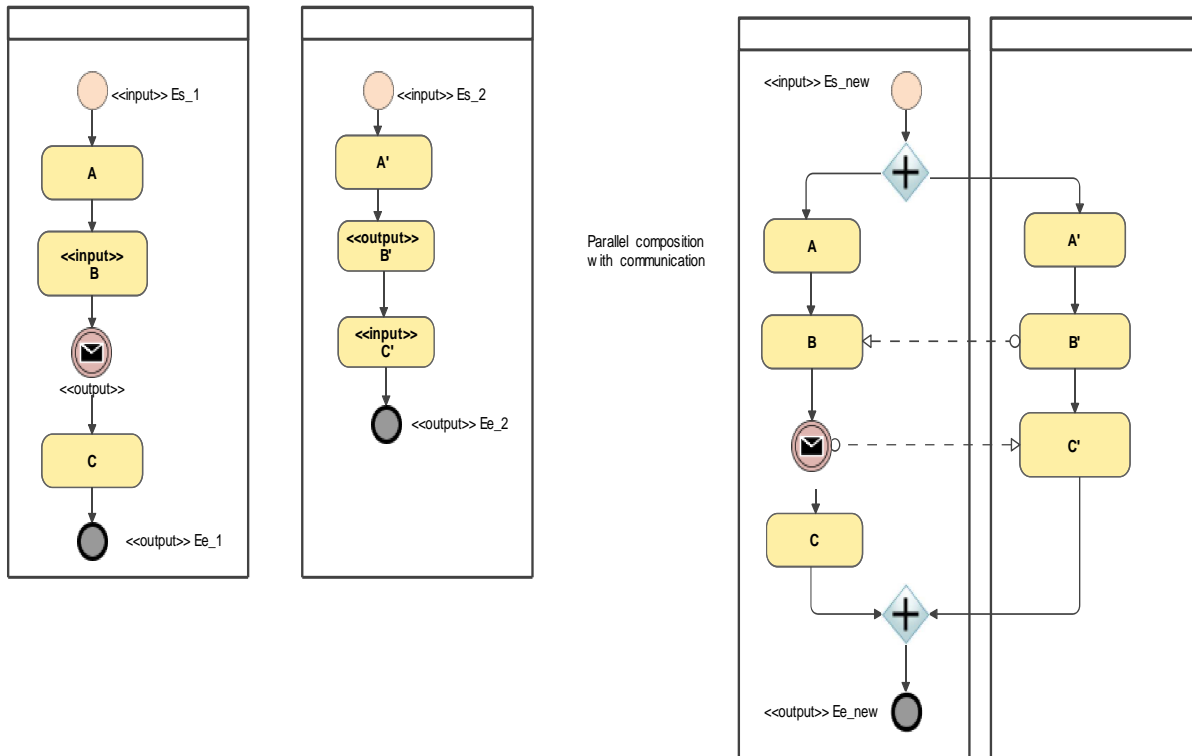
Fig. 7.6: Parallel with communication composition operator for business process fragments
