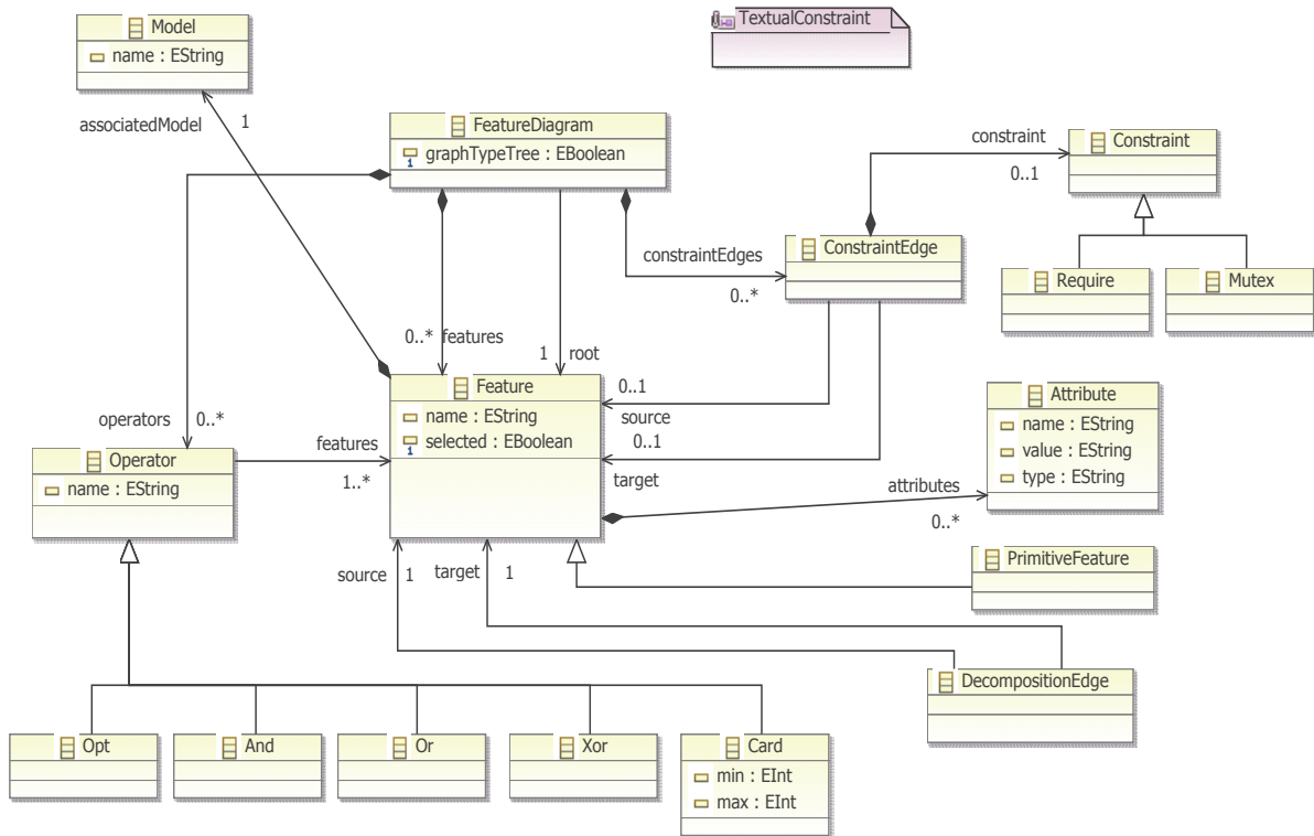
Fig. 3.2: Feature diagram meta-model
