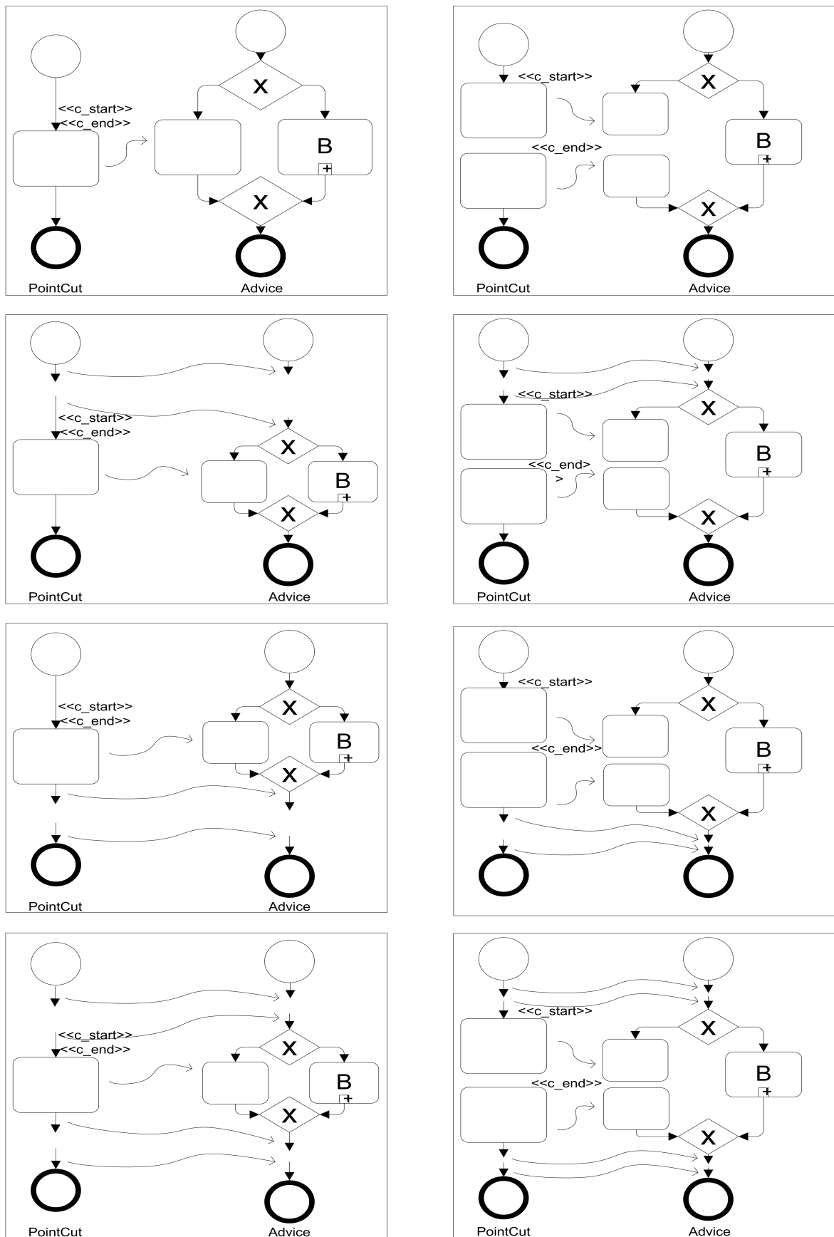
Fig. 7.15: The eight aspects for the choice composition
