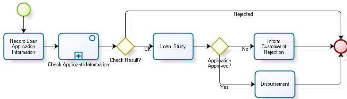
Fig. 2.8: Simple BPMN diagram example - part 2
