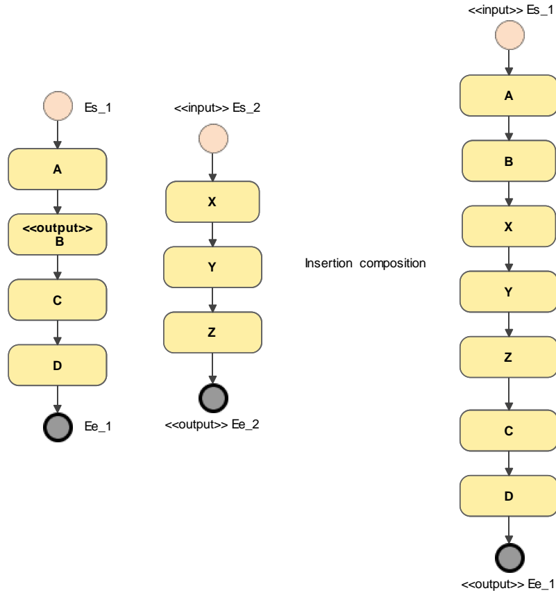
Fig. 7.9: Insert after composition operator for business process fragments
