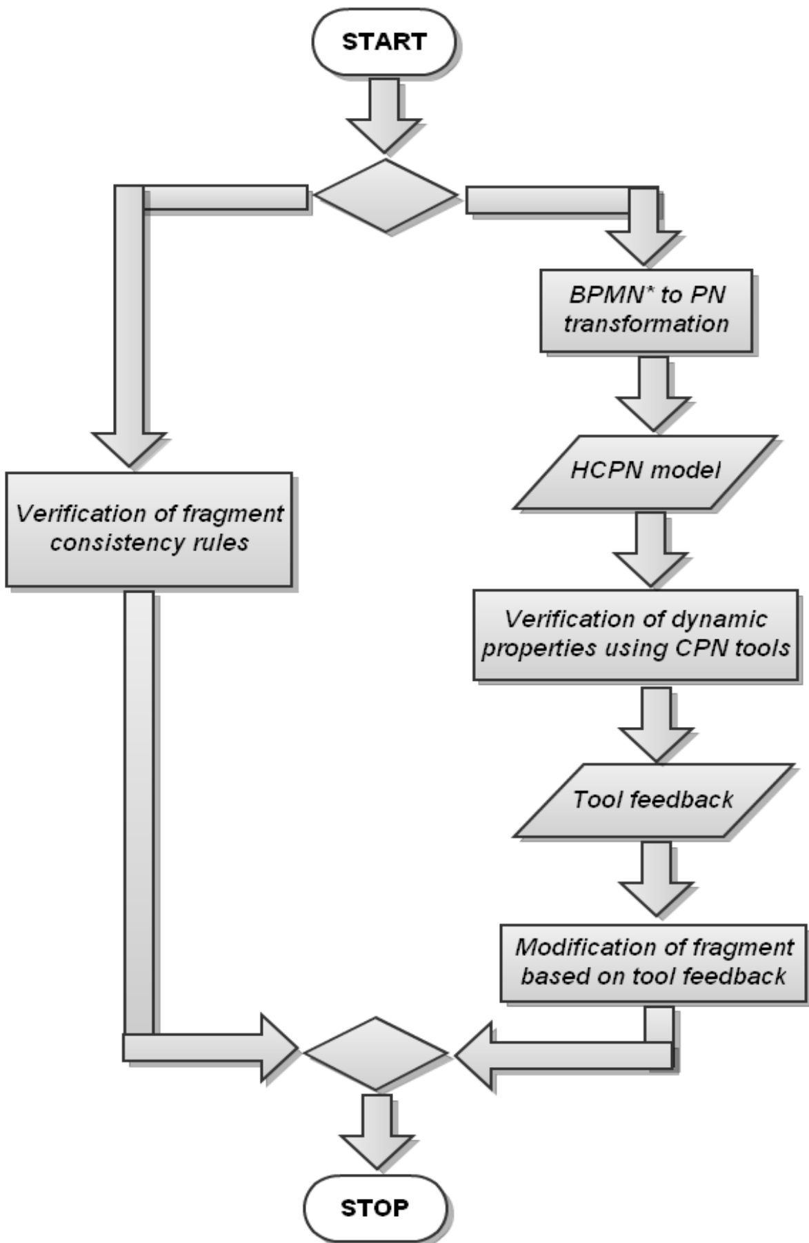
Fig. 3.5: Complete process of verification of business process fragments
