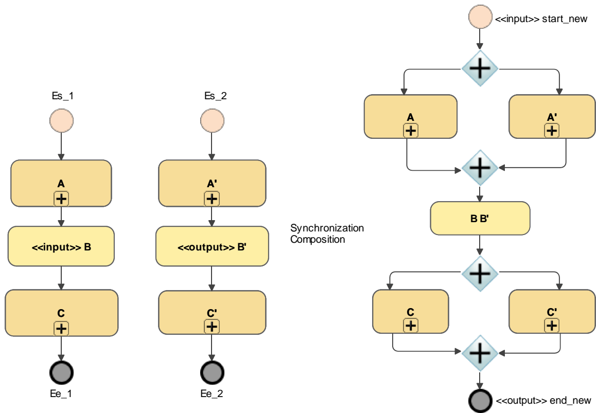
Fig. 7.8: Synchronization composition operator for business process fragments
