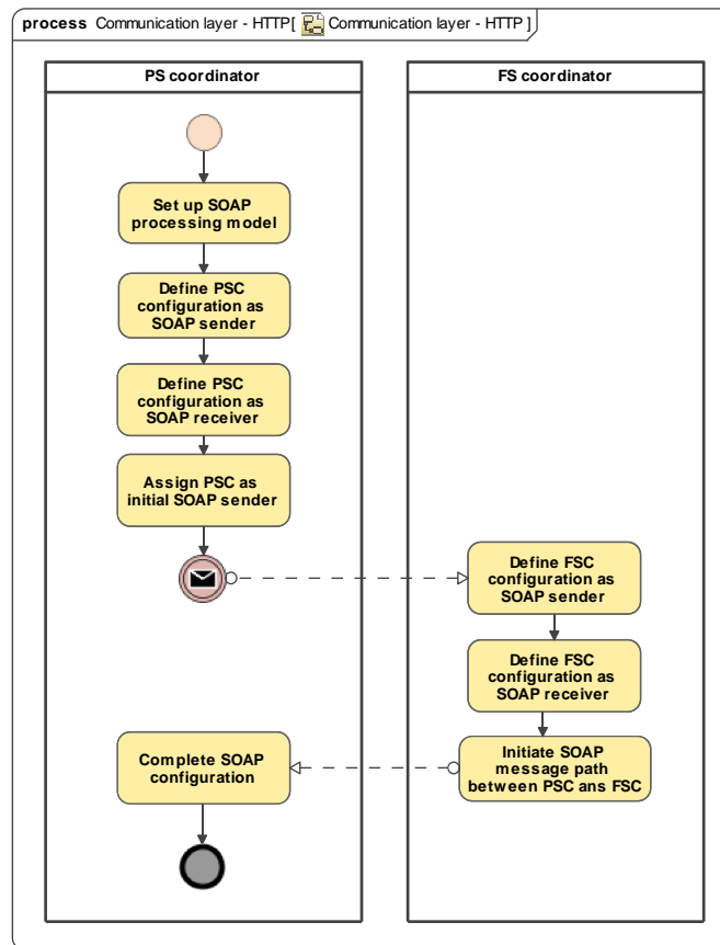
Fig. A.23: SOAP based communication layer business process fragment
