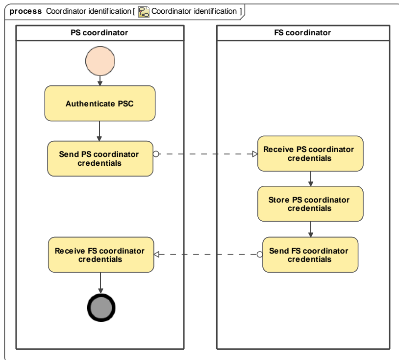
Fig. A.2: Coordinator identification business process fragment
