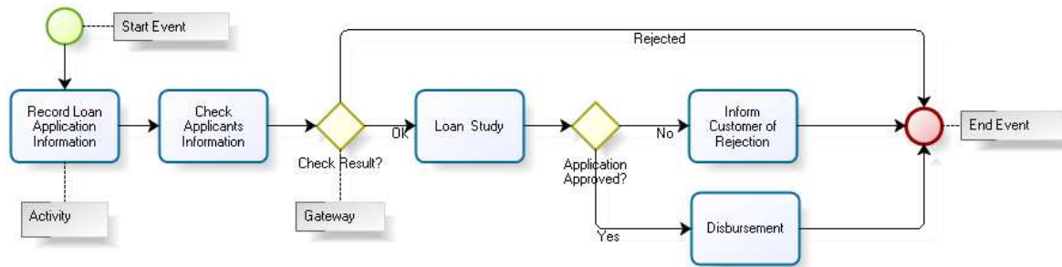
Fig. 2.7: Simple BPMN diagram example - part 1
