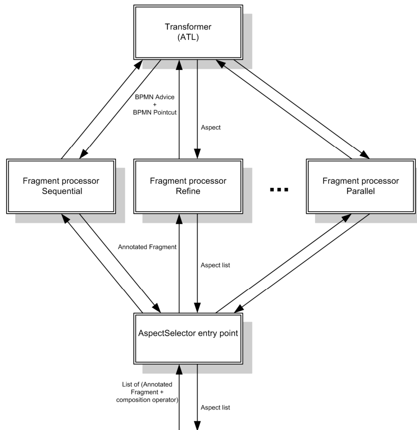
Fig. 6.24: Architecture of the Fragment to aspect adapter module
