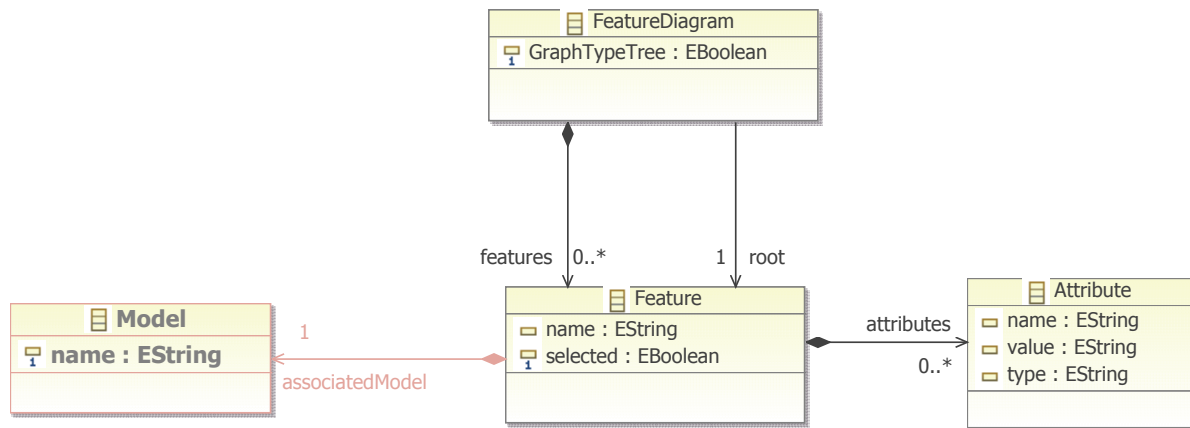
Fig. 3.6: Feature diagram meta-model: associating fragments to features
