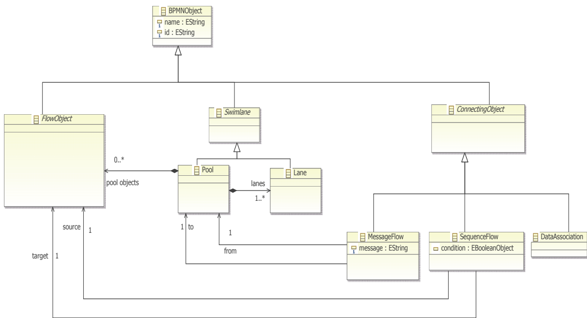
Fig. 4.4: Excerpt of language meta-model: swimlanes and connecting objects
