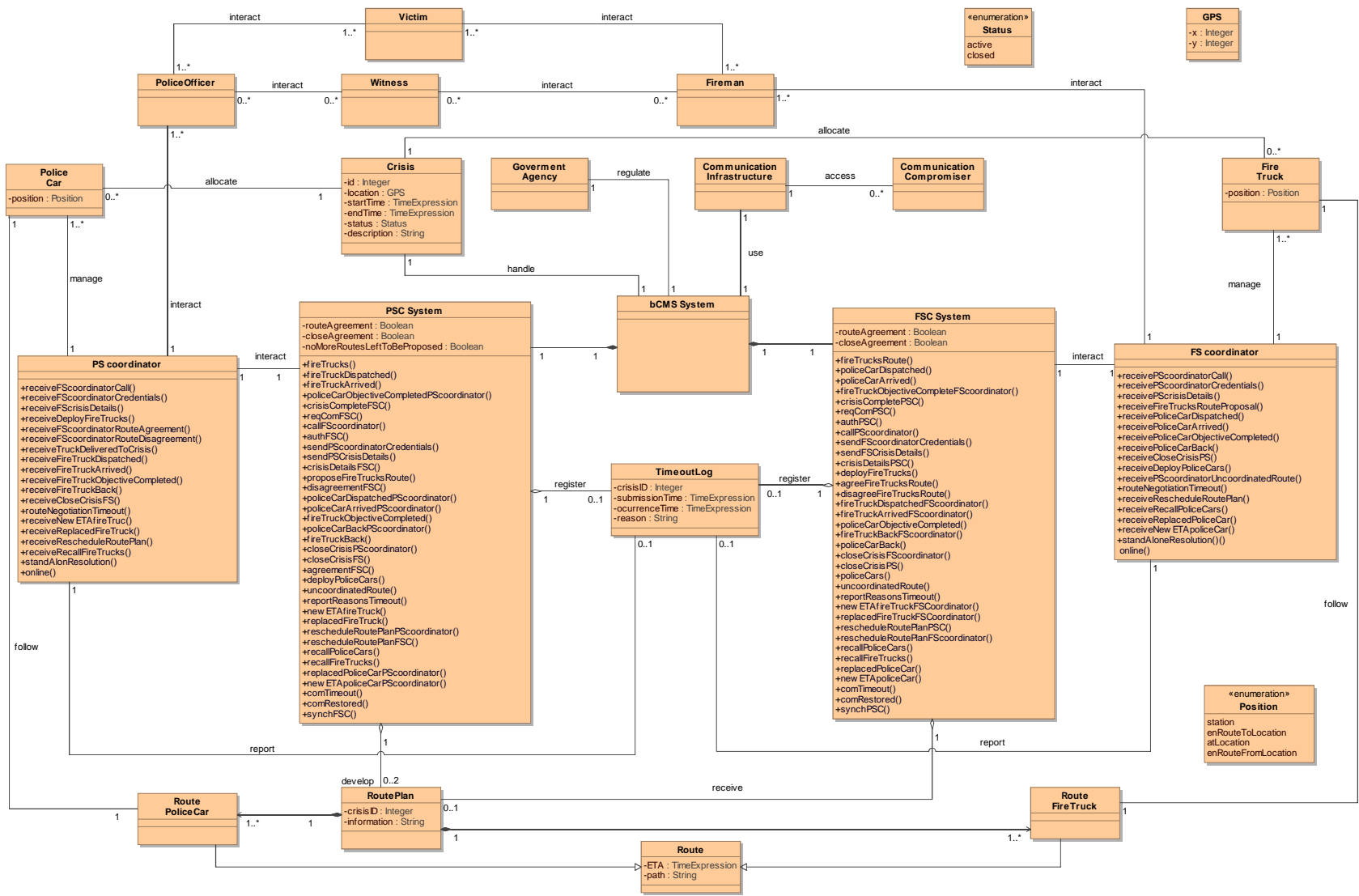
Fig. 6.2: Domain model of the BCMS system
