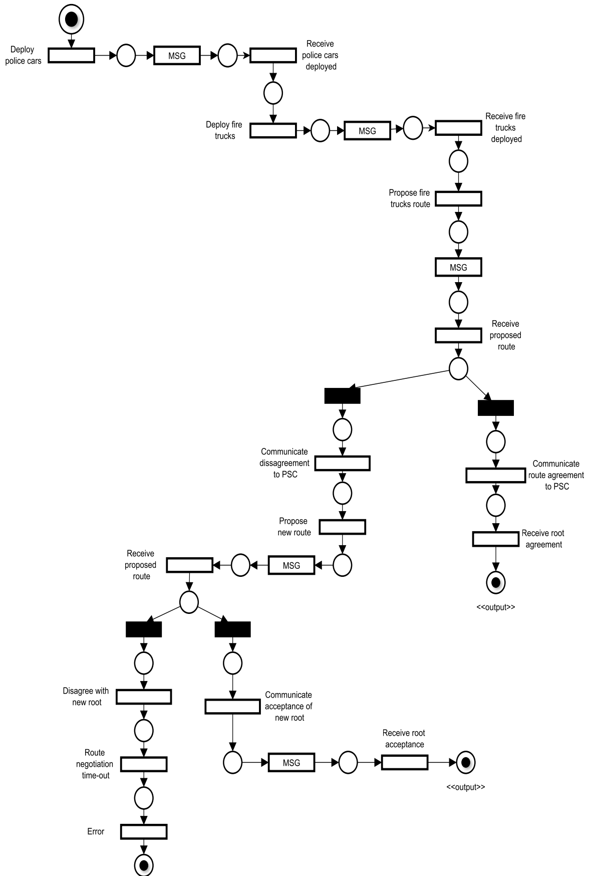
Fig. 6.11: Transforming the Creation of coordinated route plan business process fragment into a HCPN
