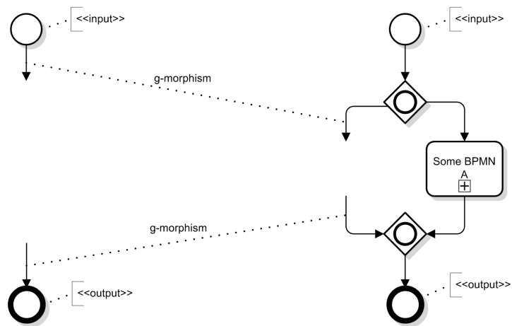
Fig. 7.13: Pointcut and Advice built for Choice composition
