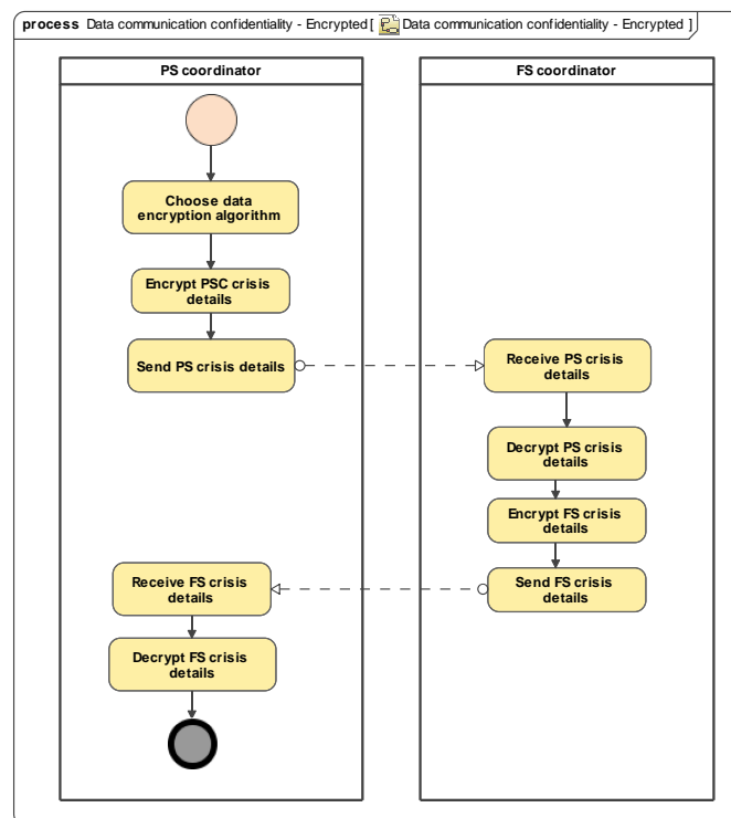
Fig. A.16: Encrypted data communication business process fragment
