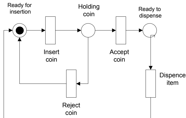
Fig. 2.9: Vending machine example using place/transition Petri nets
