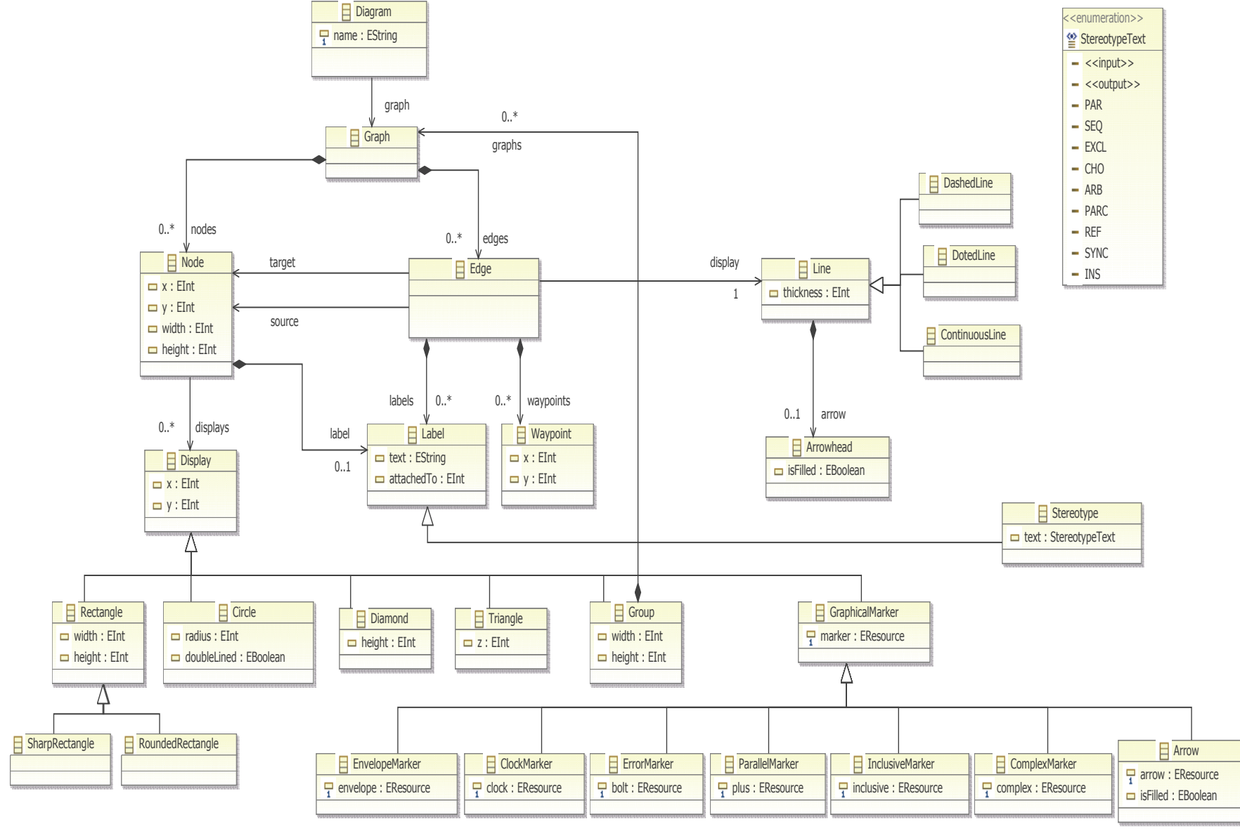
Fig. 4.13: A general model of diagrams for describing the concrete syntax of the language
