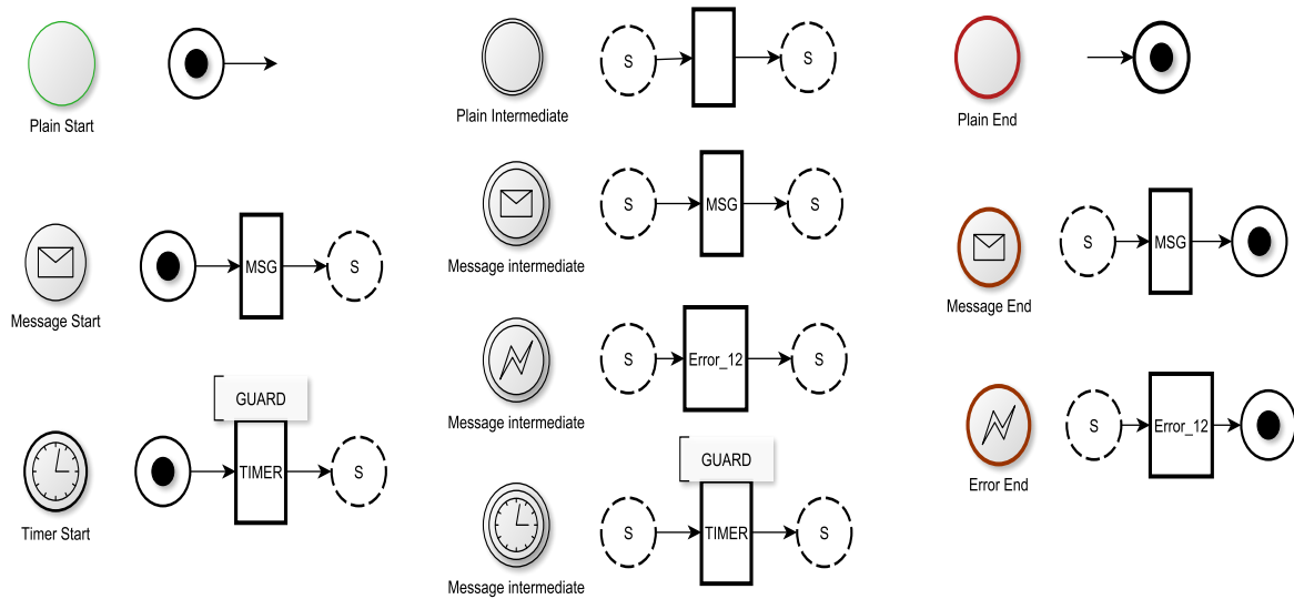
Fig. 4.20: Mapping template from CBPF to HCPN: events
