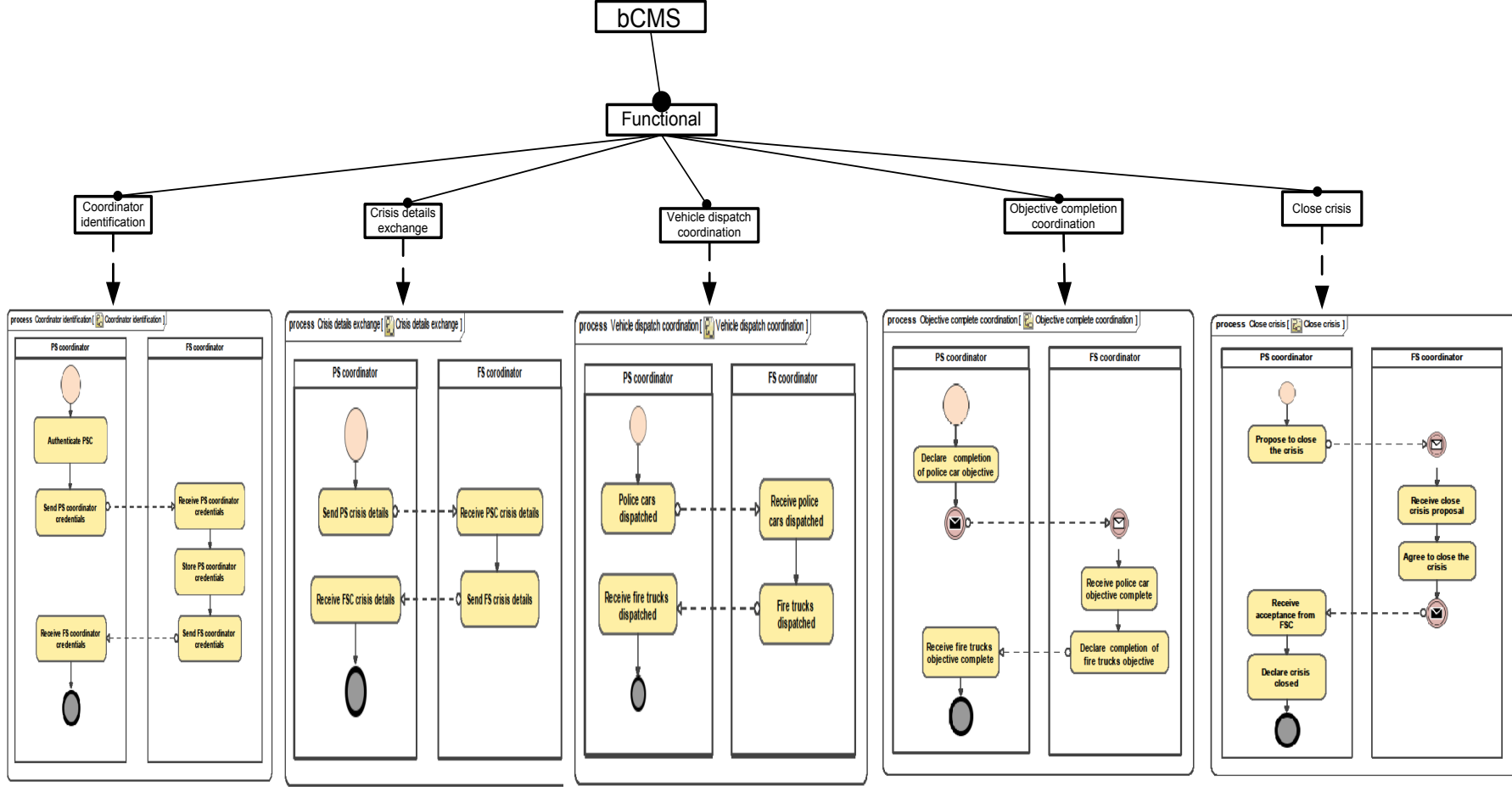
Fig. 6.12: Connecting features to business process fragments for the bCMS case study
