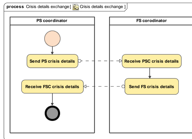
Fig. A.3: Crisis details exchange business process fragment
