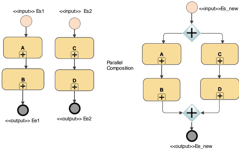
Fig. 7.2: Parallel composition operator for business process fragments
