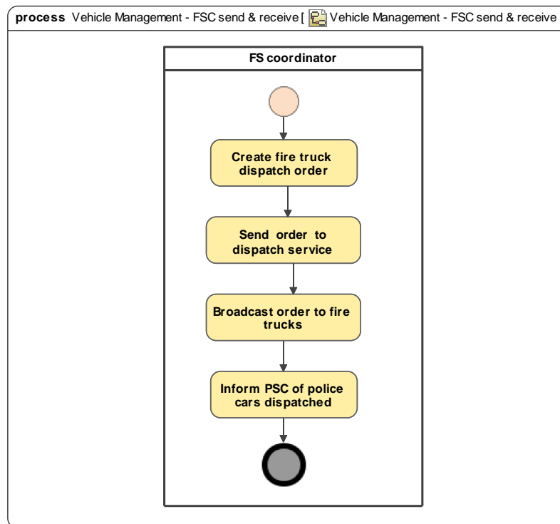
Fig. A.11: Vehicle management - FSC send and receive business process fragment
