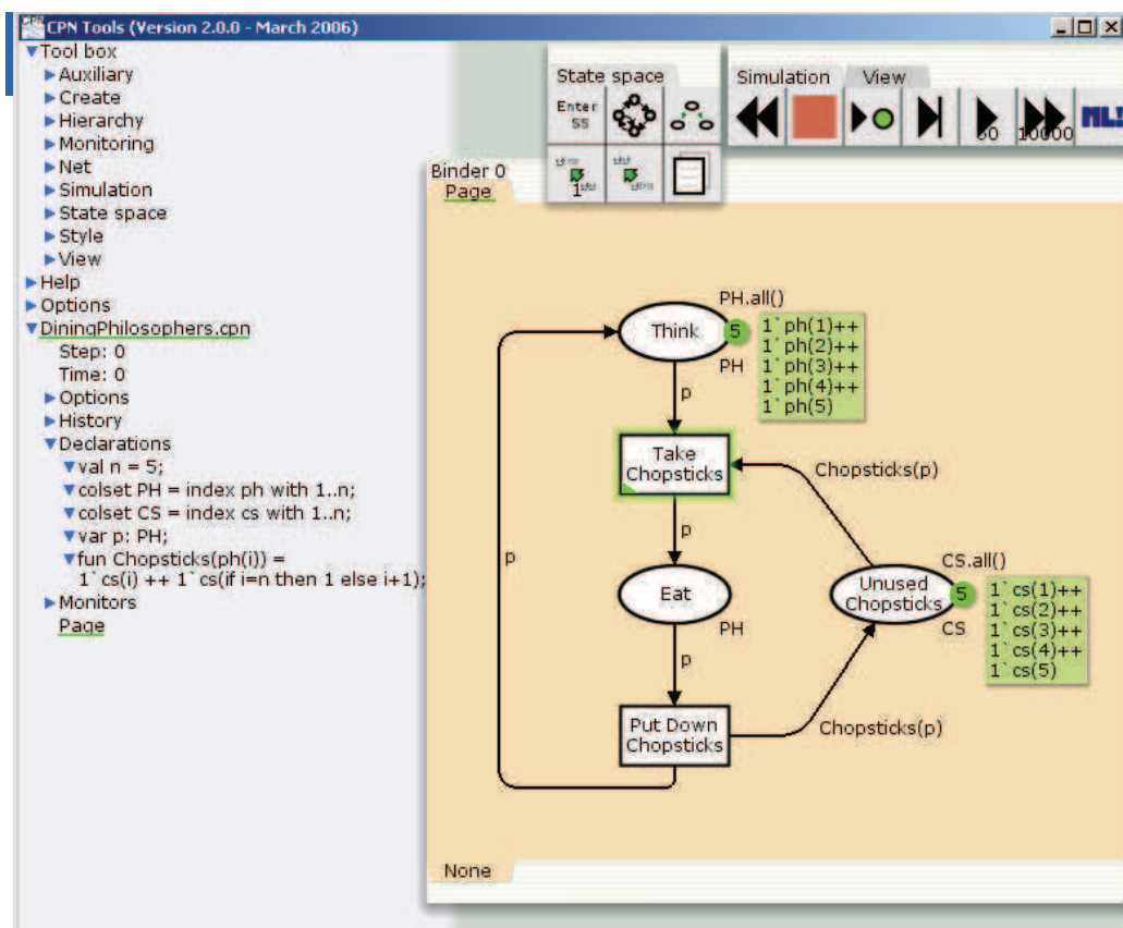
Fig. 6.23: Screen-shot of CPN Tools interface
