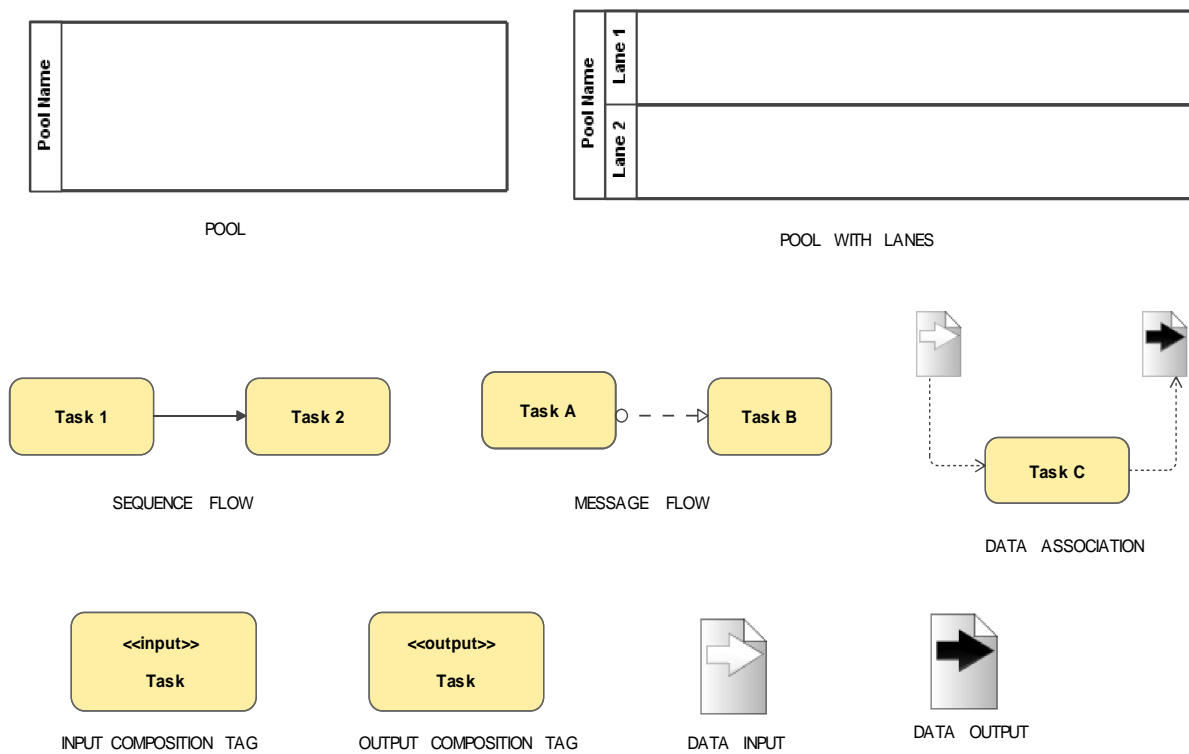
Fig. 4.11: Graphical concrete syntax for: swimlanes, connecting objects and artifacts
