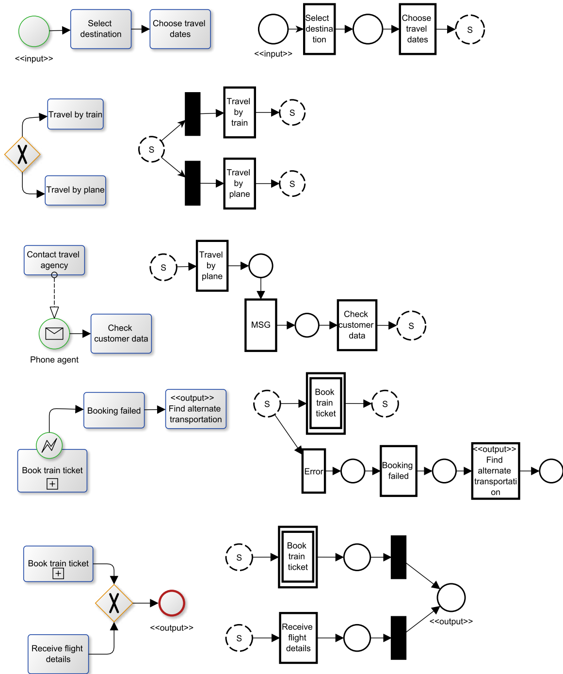
Fig. 4.22: Mapping transportation reservation fragment to HCPN: Step 1
