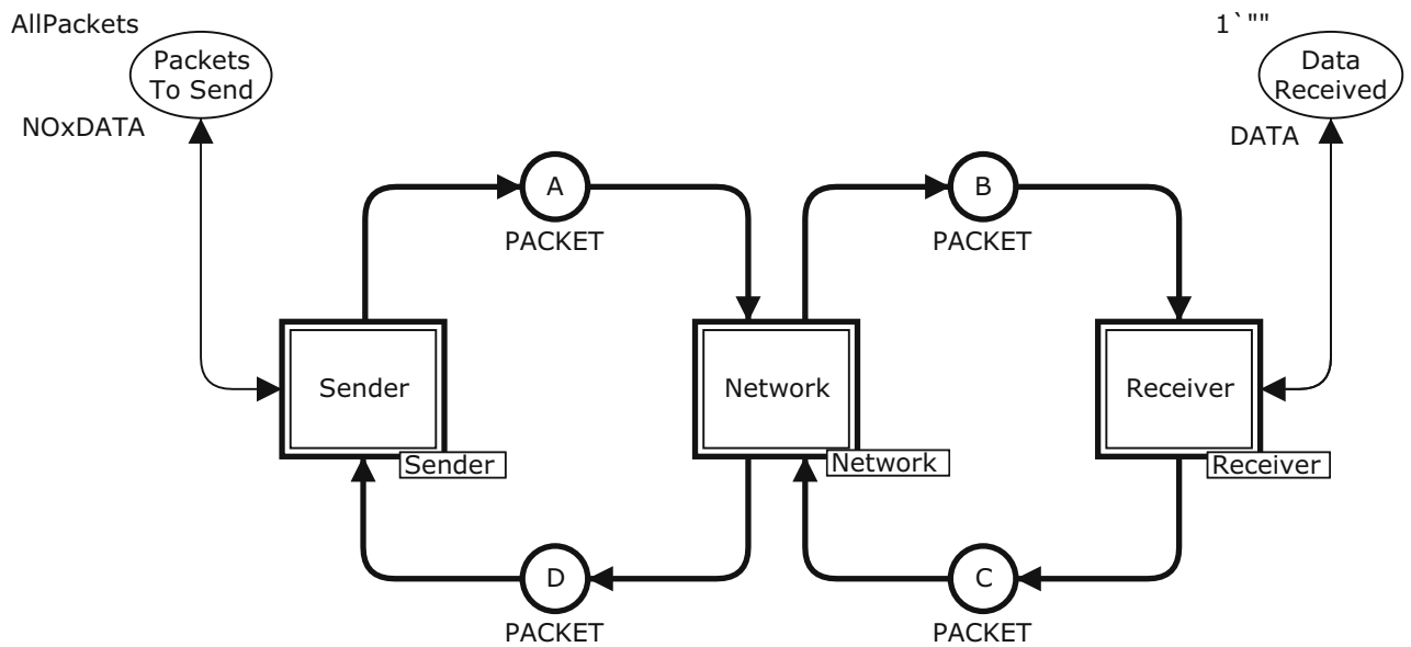
Fig. 2.11: High level hierarchical view of the communication protocol
