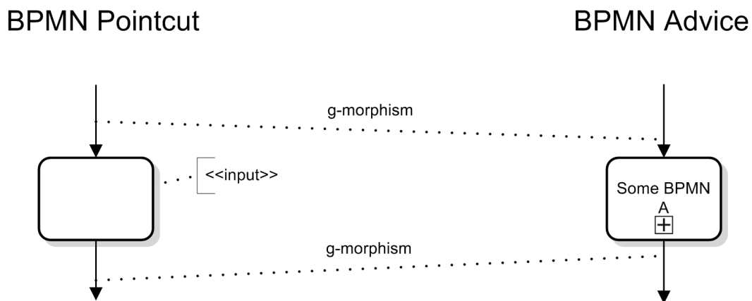
Fig. 7.17: Pointcut1 and Advice built for Refinement composition
