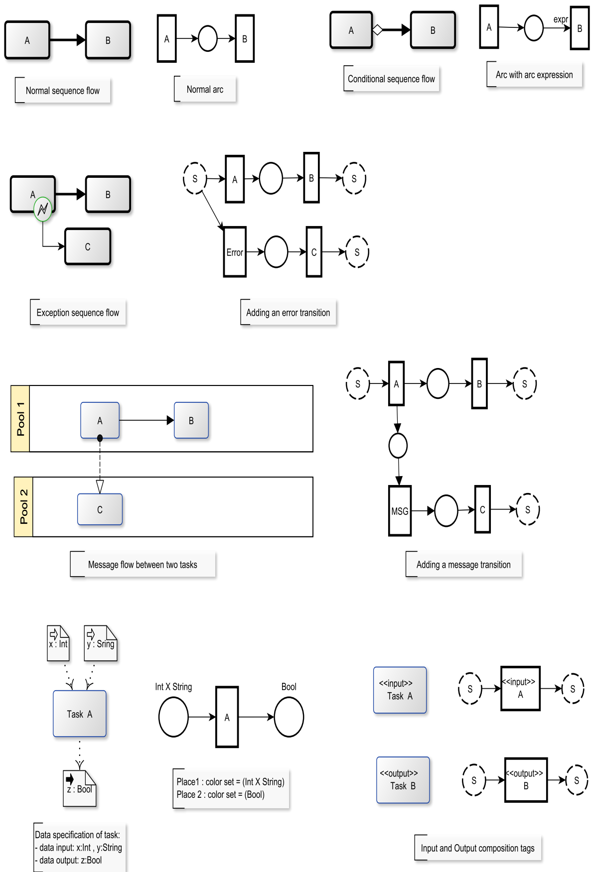
Fig. 4.21: Mapping template from CBPF to HCPN: sequence flow, message flow, data association, data objects and composition tags
