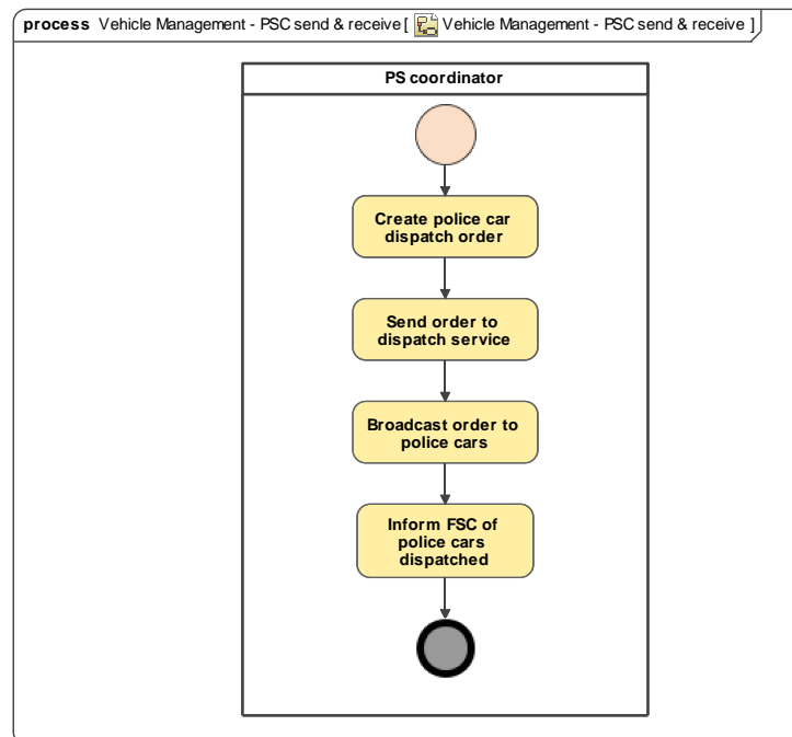
Fig. 6.7: PSC send and receive business process fragment
