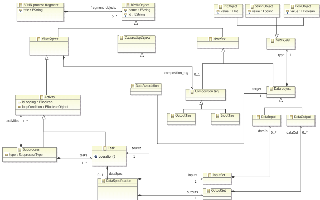
Fig. 4.5: Excerpt of language meta-model: newly introduced concepts
