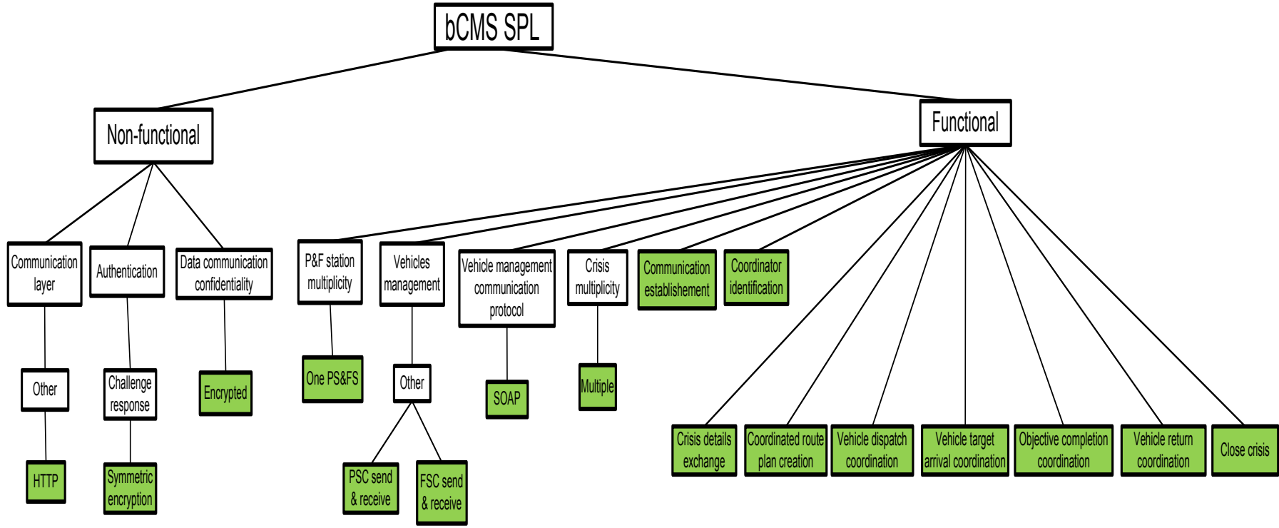
Fig. 6.13: Feature diagram configuration of bCMS product
