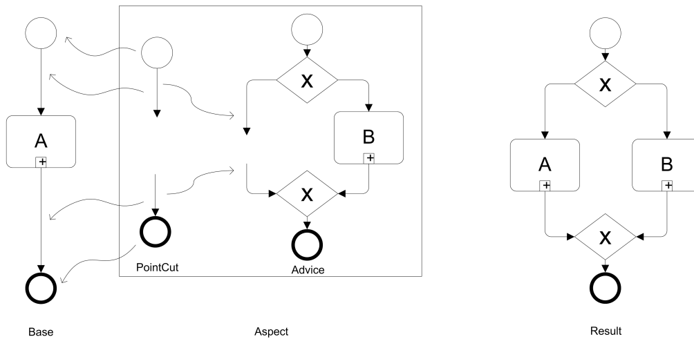
Fig. 7.14: Exclusive choice composition of processes with aspects
