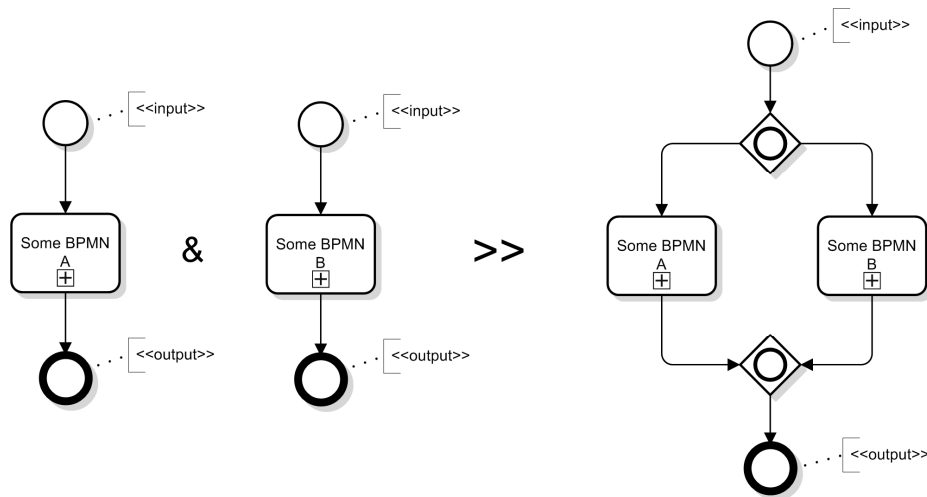
Fig. 7.11: Choice composition of business process fragments
