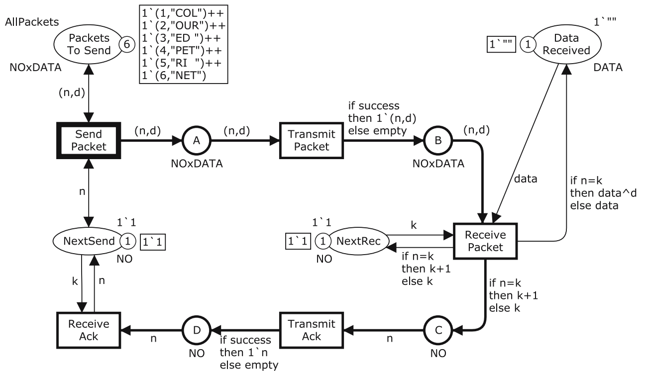
Fig. 2.10: Basic HCPN model of the simple communication protocol
