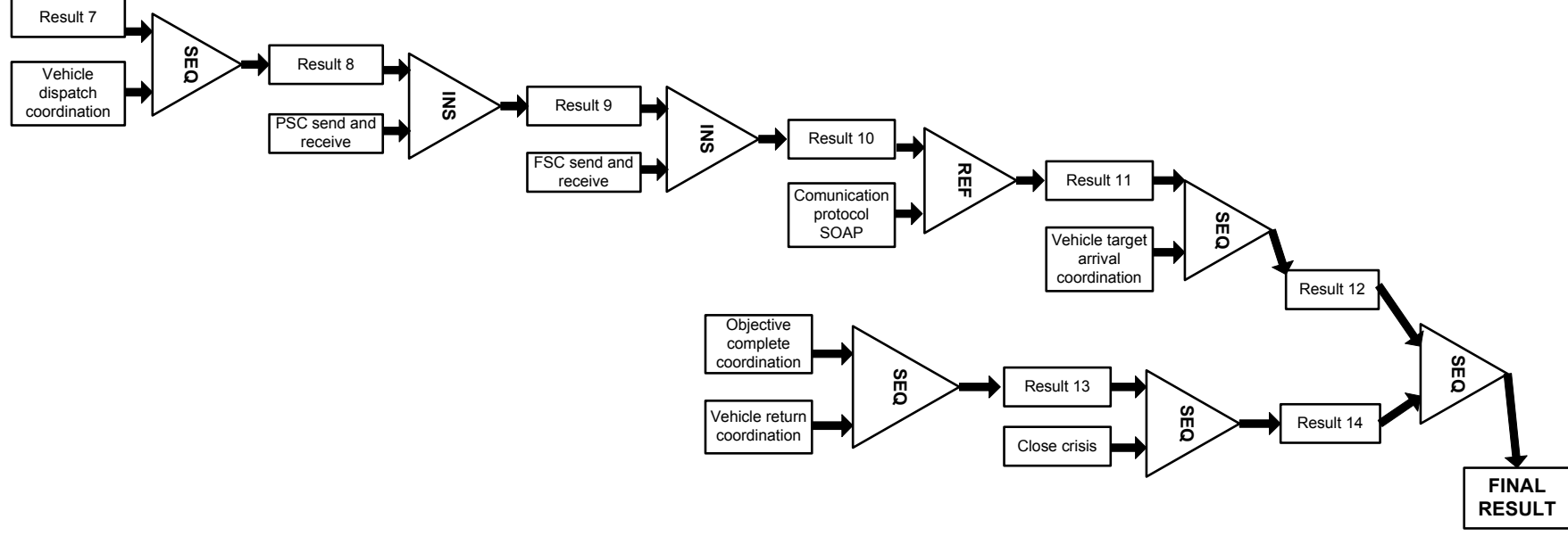
Fig. 6.17: Second part of composition workflow for bCMS example
