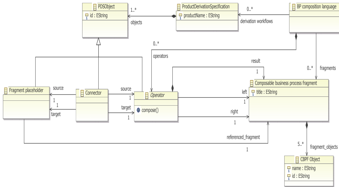
Fig. 4.9: Excerpt of language meta-model: support for product derivation specification
