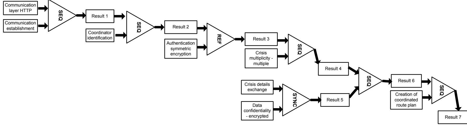
Fig. 6.16: First part of composition workflow for bCMS example
