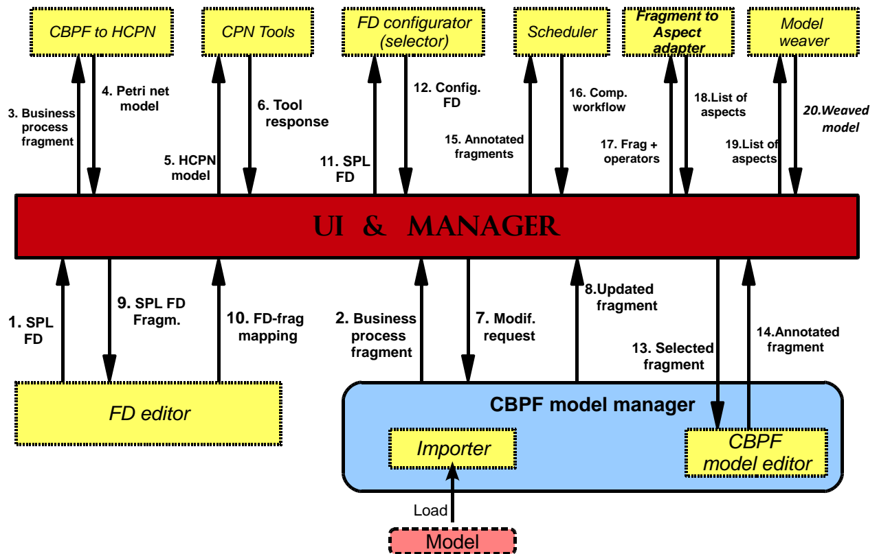
Fig. 6.19: Usage of the SPLIT tool
