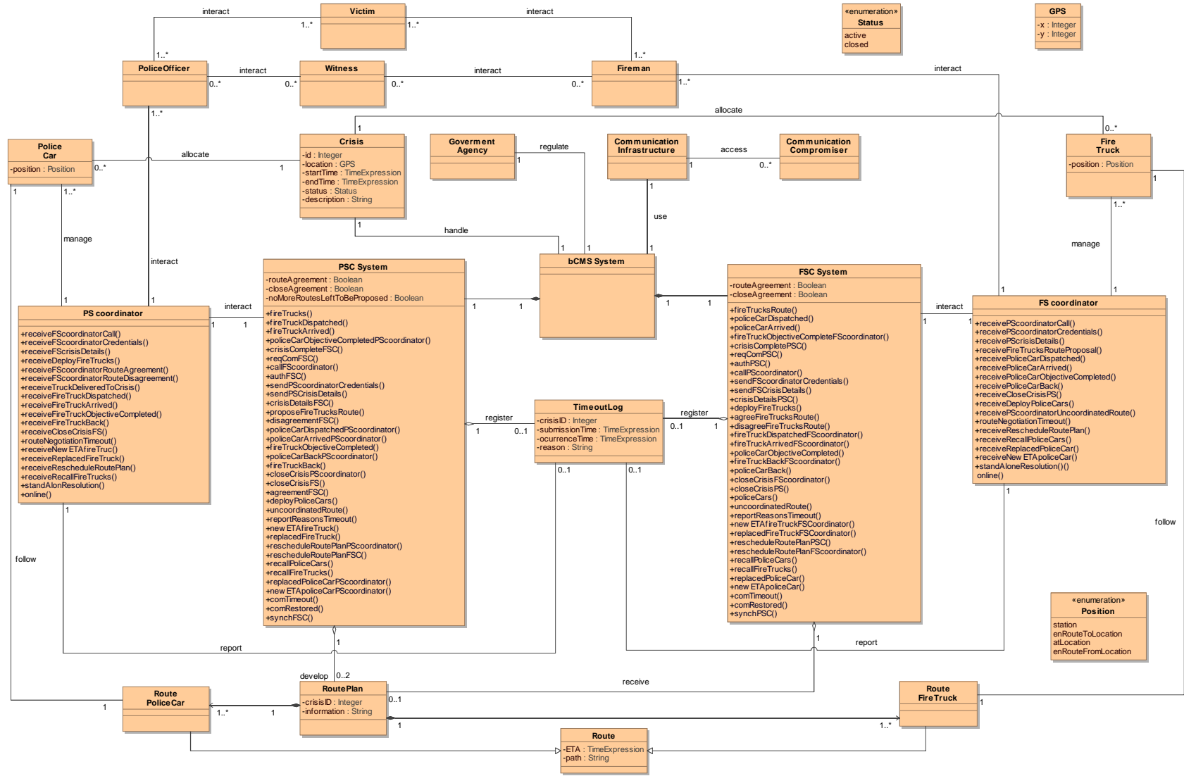
Fig. 6.2: Domain model of the BCMS system
