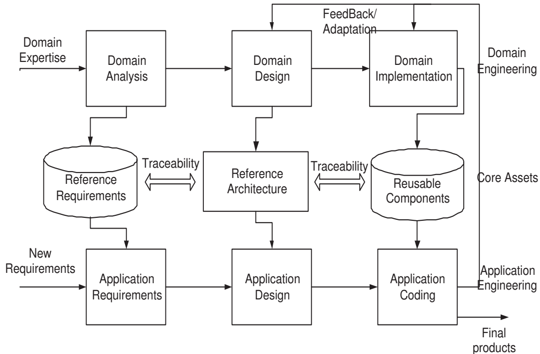
Fig. 2.1: General SPL engineering process [PBvdL05]
