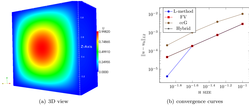
Figure 3.7: Diffusion problem
