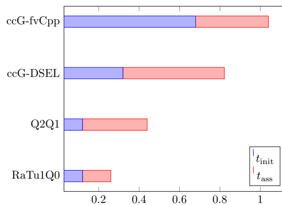
Figure 3.18: Comparison of different methods and implementations for the test case of §3.5.5
