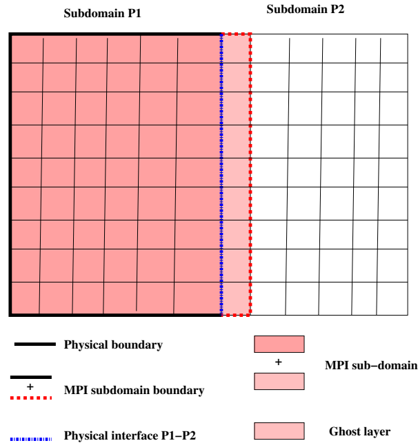
Figure 4.7: Mesh partition, sub-domain boundaries and interfaces
