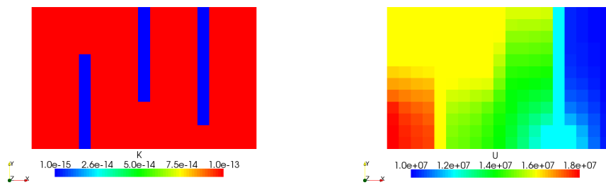
(b) Permeability field
