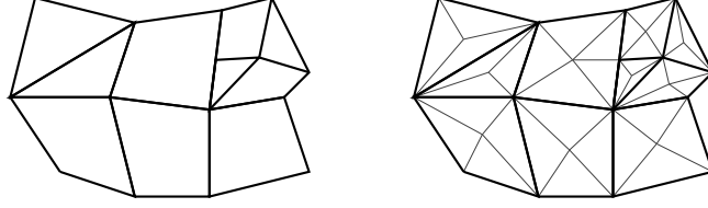
Figure 2.1: Left. Mesh \mathcal{T}_h Right. Pyramidal submesh \mathcal{P}_h
