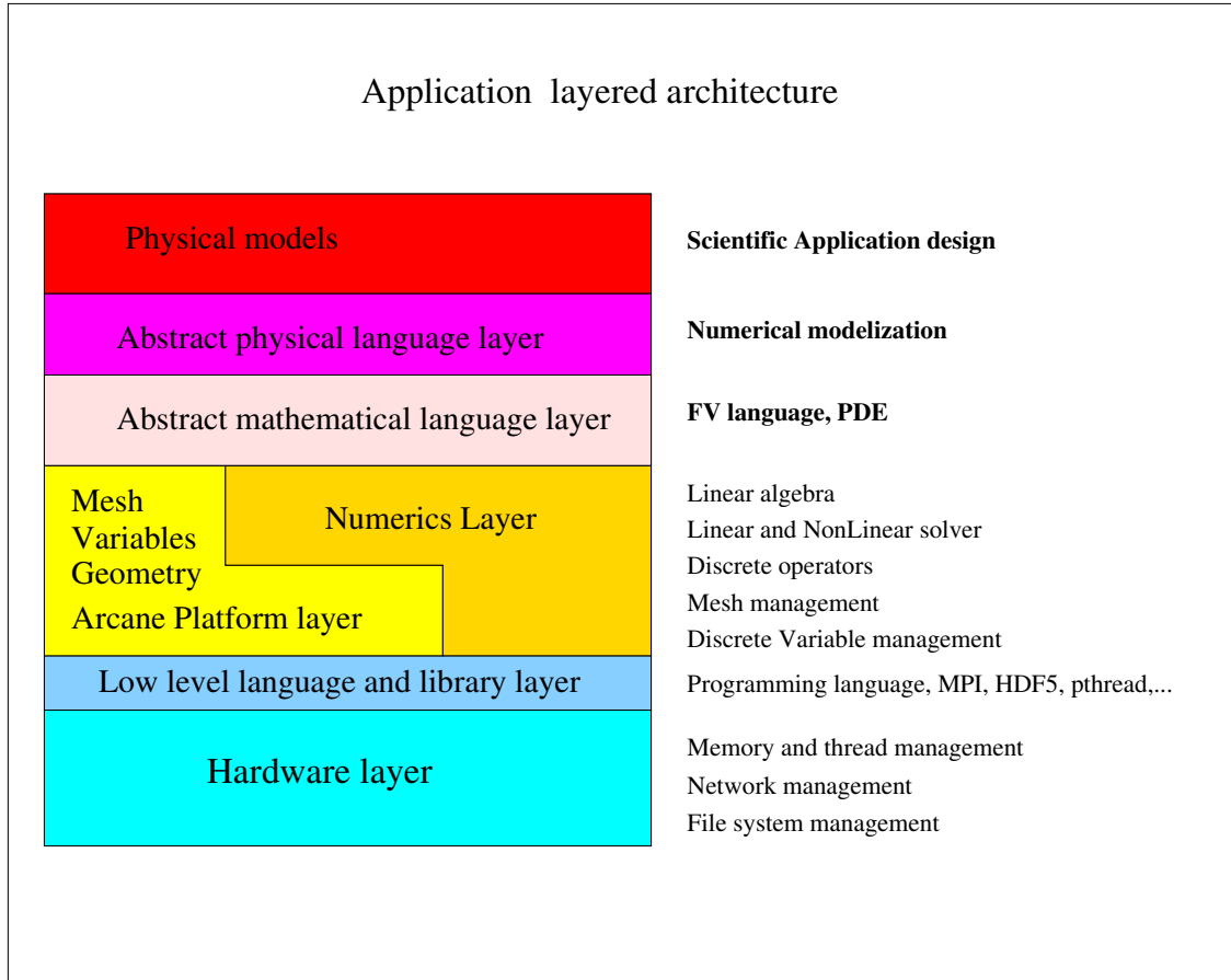
Figure 1.2: Layer Architecture.
