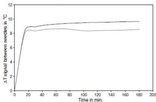
Fig. 1 Kinetics of sensor temperature difference during the non-stationary period (1) under zero flow conditions (black line) and (2) under medium, midday flow conditions, J=0.7 \text{ L m}^{-2} \text{ h}^{-1} (grey line)
