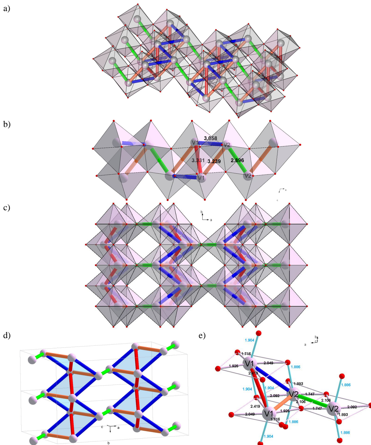
Figure 4. Structure of HTP-VO 2 (B). a): perspective view; b): projection in (101) with V-V distances; c): projection in (110); d) perspective view with highlighting of V-V bonding scheme (oxygen ions not shown); e): perspective view with V-O distances.
