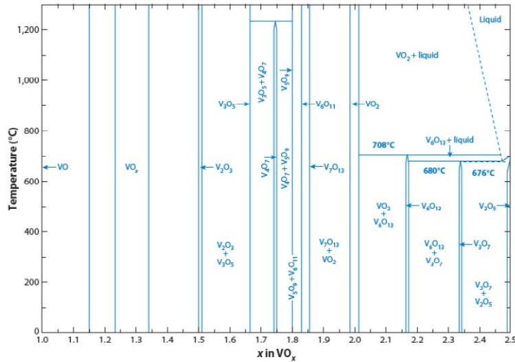
Figure 1. \text{VO}_x phase diagram [4].
