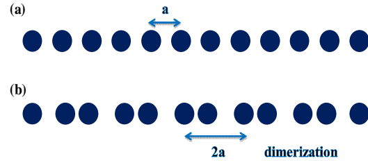
Figure 5. Representation of a 1D system (a) before and (b) after the Peierls transition.
