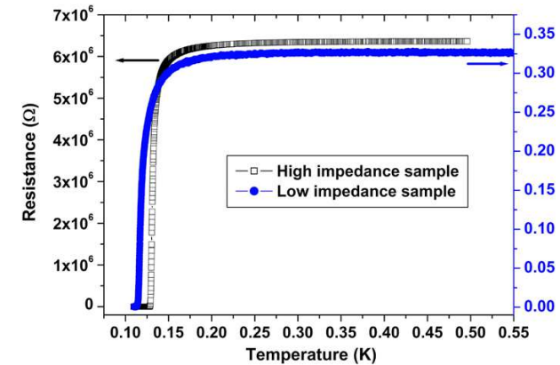
Fig. 2 (Color online) Resistance as a function of temperature for superconducting films which design has been adapted for either JFET or SQUID readout
