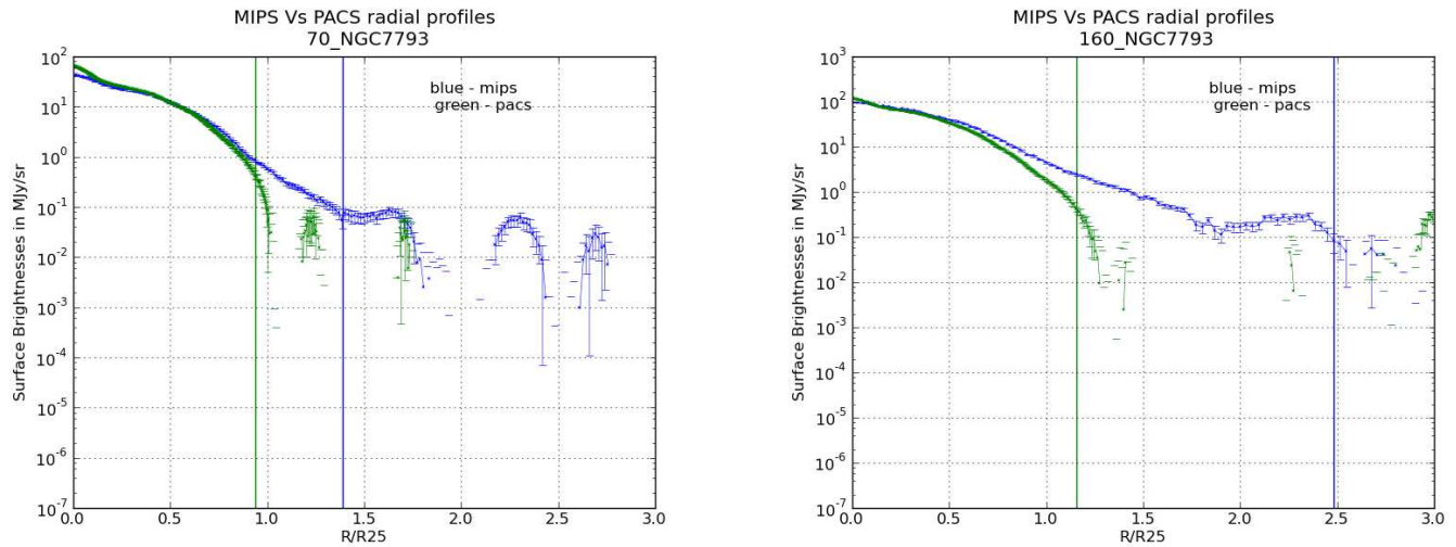
Figure 2.2: We give in these figures surface brightnesses obtained for NGC7793 in rings associated with original map grid for MIPS (blue) and PACS (green), for 70\mu m (left) and 160\mu m (right) after convolving to resolution of SPIRE 500. In abscissa are shown values of R/R25 .
