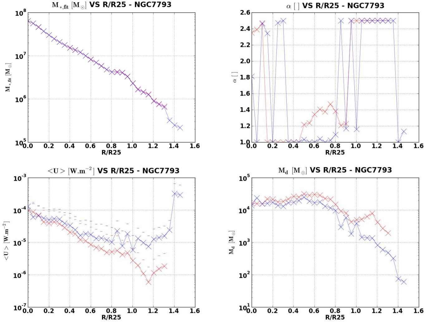
Figure 2.6: We give in these figures fitting results against R/R_{25} radii for NGC 7793. M_{\star,fit} are values of the stellar mass necessary to remove the NIR-MIR stellar continuum, if we suppose that the only stellar source at these wavelengths is a 1 Gyr old stellar population. The errorbars on the figure representing \langle U \rangle are values of \sigma(\langle U \rangle) , the standard deviation of the distribution of U along the line of sight.
