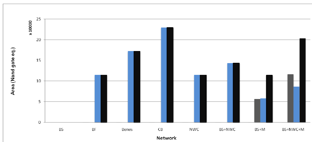
Figure 5. 19 HSPA 800 data
