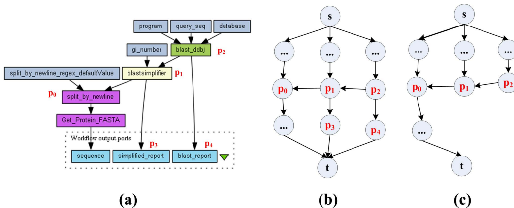
Figure B.2: (a) Example of non-SP workflow from myExperiment ("blastsimplifier" ( p_1 ) and "blast_ddbj" ( p_2 ) are trace nodes and links "blastsimplifier( p_1 ) \rightarrow simplified_report( p_3 )" and "blast_ddbj( p_2 ) \rightarrow blast_report( p_4 )" are trace links); (b) the specification of (a). If the two trace links in (a) are removed, (b) will not be non-SP graph anymore and the workflow will be an SP workflow (the SP version of the specification is shown in (c)). Recall that this removal should actually be done very carefully since removing trace links implies removing part of the workflow outputs (see section 5.5.3).
