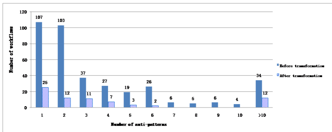
Figure 5.9: Distribution of number of anti-patterns among workflows in myExperiment, before and after applying DistillFlow.
