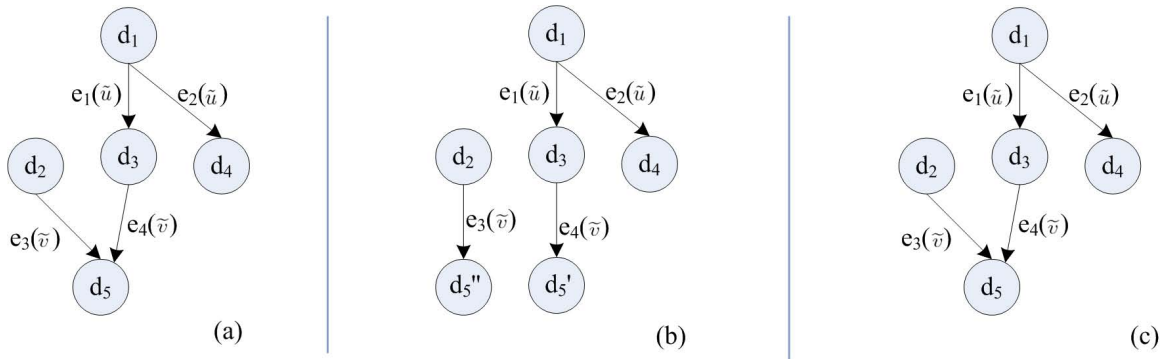
Figure 4.7: Data dependency graphs for runs in Figure 4.6.
