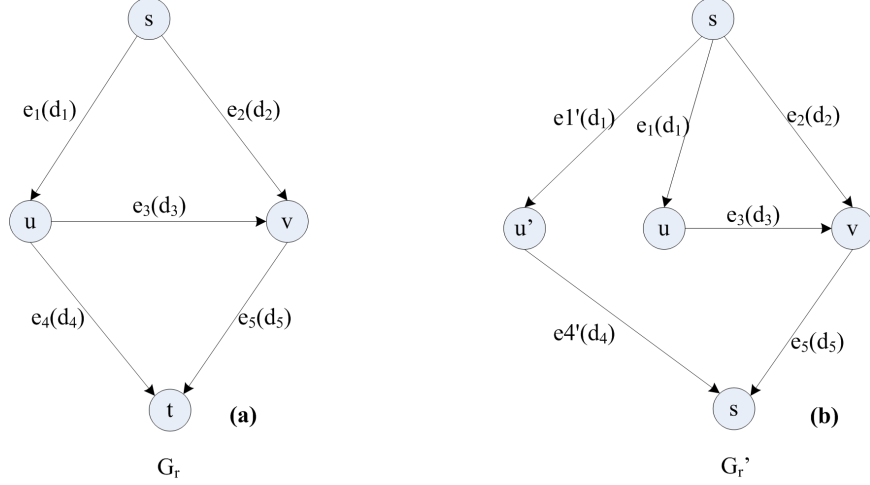
Figure 3.2: Two graph illustrating provenance related notions
