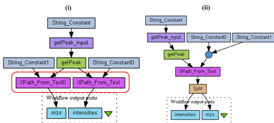
Figure 5.13: Example of workflow (myExperiment 941)
