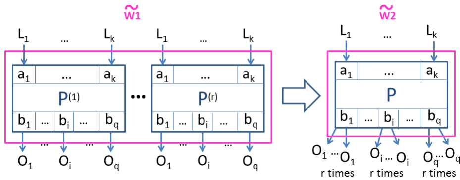
Figure 5.3: Transformation for anti-pattern (A)
