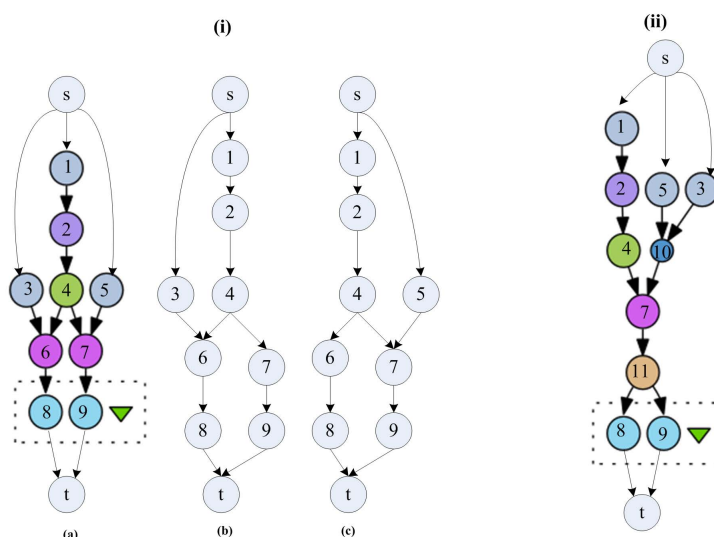
Figure 5.14: Specification graphs of workflows in Figure 5.13 ((i).(b) and (i).(c) are the two forbidden subgraphs induced by node #4 in (i).(a), (ii) is the SP graph obtained when nodes #6 and #7 are merged into one node, called #7)
