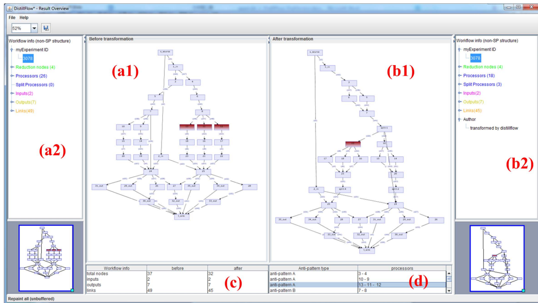
Figure A.3: Visualizing both initial workflow and distilled workflow. The initial workflow and distilled workflow are respectively represented in panels (a1) and (b1). The panels (a2) and (b2) respectively display metadata of the two versions of workflows (number of processors, links, authorship information etc.) while panel (c) provides the metadata of the two graphs displayed in (a1) and (b1) (number of total nodes, links etc.). The panel (d) is particularly important and provides a table of all the anti-patterns detected in the original workflow. Here, the user has clicked on anti-pattern "13-11-12" in the anti-pattern information panel (d) which has automatically highlighted the corresponding anti-pattern both in the initial workflow (panel (a1)) in which three vertices are involved and in the distilled workflow (panel (b1)) in which the anti-pattern has been removed by the system, merging vertices "13", "11" and "12", resulting in only one vertex, numbered 13.
