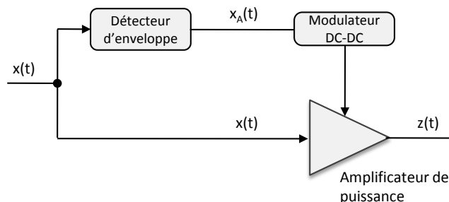
FIGURE 1.8 – Architecture de la technique ET
