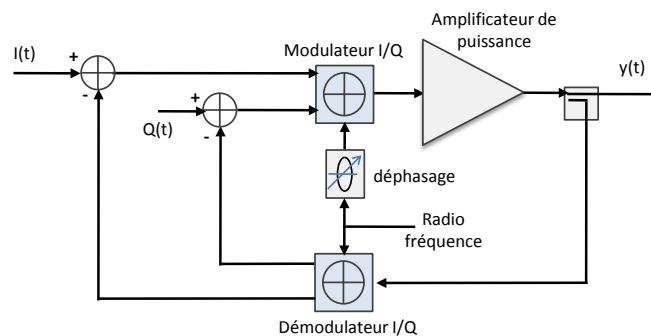
FIGURE 1.10 – Architecture de la technique feedback cartésien
