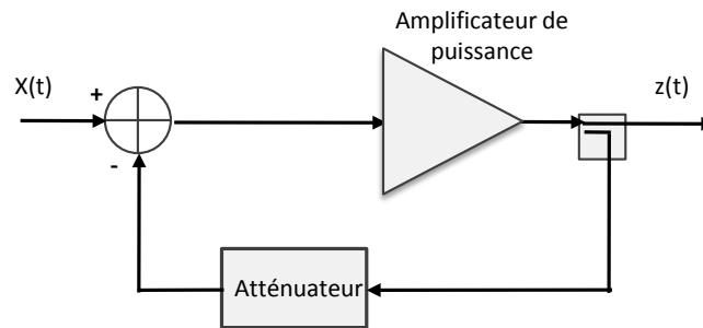
FIGURE 1.9 – Principe de la technique FeedBack
