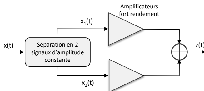
FIGURE 1.6 – Architecture de la technique LINC
