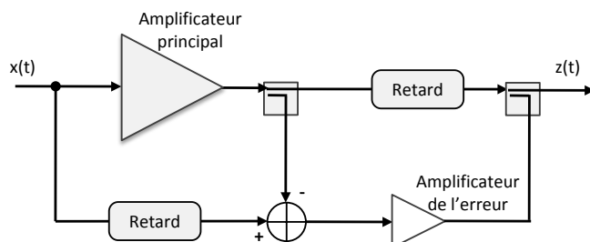
FIGURE 1.11 – Architecture de la technique FeedForward
