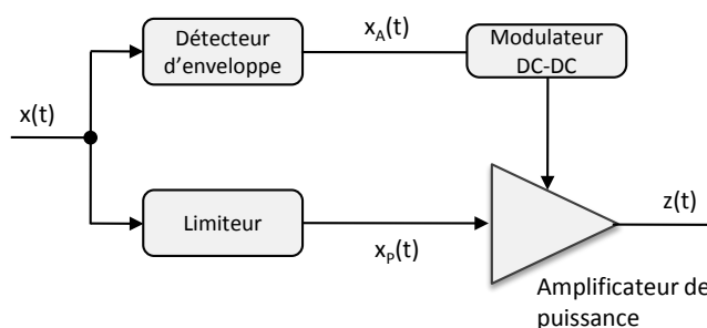
FIGURE 1.7 – Architecture de la technique EER
