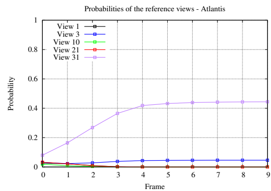
(g) Marginal joint probabilities of the views
