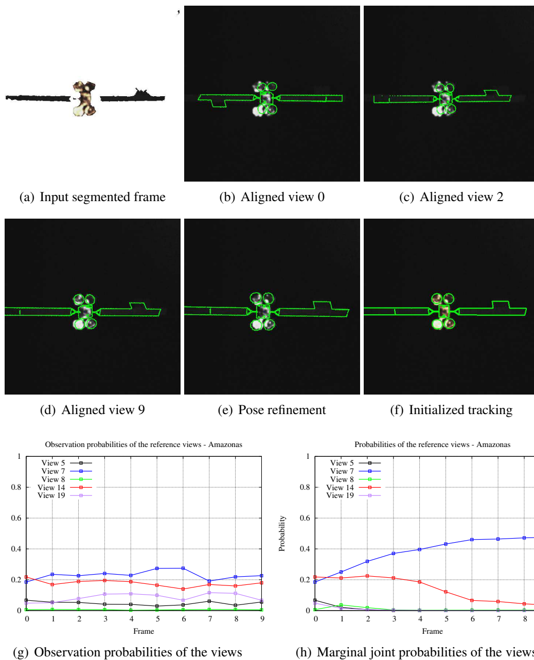
Figure 3.24 – Segmentation, detection and pose estimation process - Amazonas sequence
