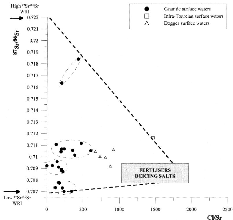
Fig. 4. Plot of the ^{87}\text{Sr}/^{86}\text{Sr} vs. Cl/Sr ratios in surface waters draining the different types of granitoids in the regional framework (see Fig. 1).
