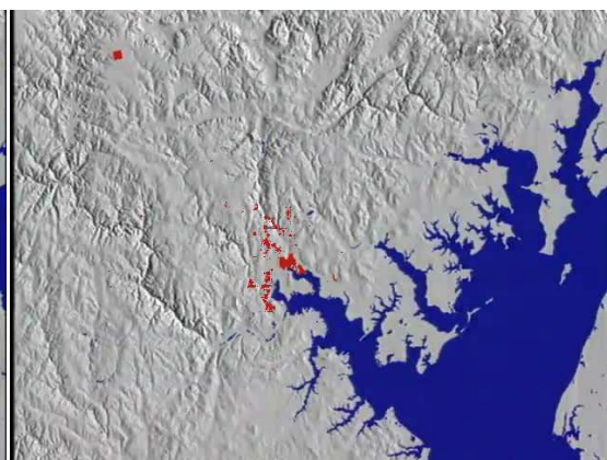
(e) Simulation 15
