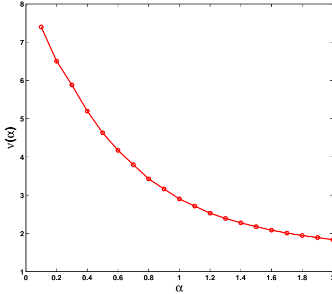
Figure 4.15: Connected length exponent \nu(\alpha) as a function of the correlation exponent \alpha calculated from (4.2.17) and (4.2.18).
