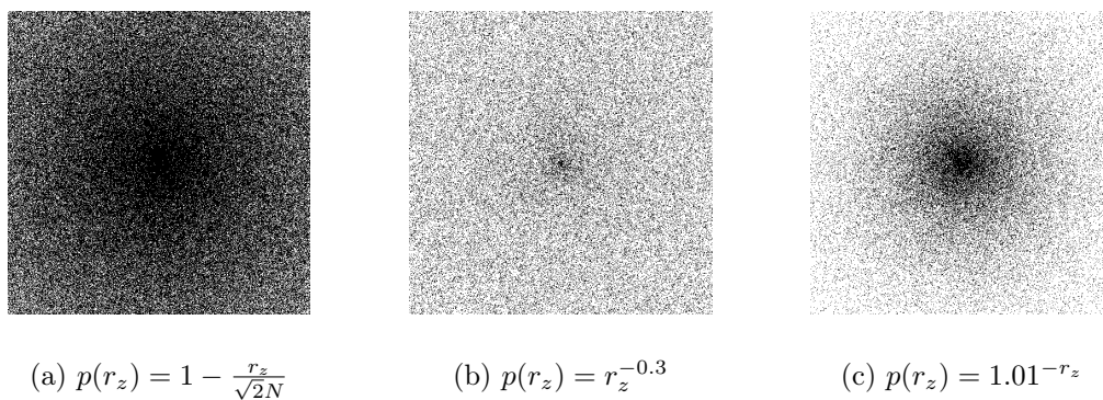
Figure 4.8: Gradient percolation with different probability functions of the distance r_z from site z to center of square lattice of size 501 \times 501 .
