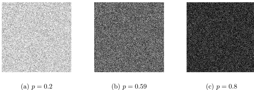
Figure 4.7: Site-Percolation with different probability p on square lattice of size 501 \times 501 .
