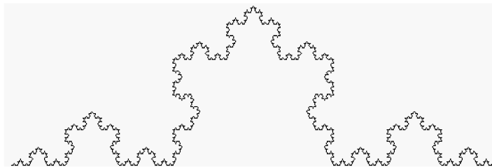
Figure 4.1: Koch curve.
