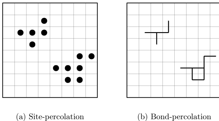
Figure 4.6: Two main types of percolation
