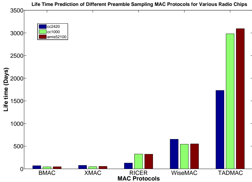
FIGURE 5.7: Lifetime prediction of AA alkaline battery is evaluated for various MAC protocols and radio chips. TAD-MAC along with amis52100 or cc1000 radio chips have major difference in comparison with other MAC protocols and cc2420 . It is noteworthy to mention here that for low traffic rate amis52100 and cc1000 are preferable but for higher traffic rate cc2420 is more suitable.
