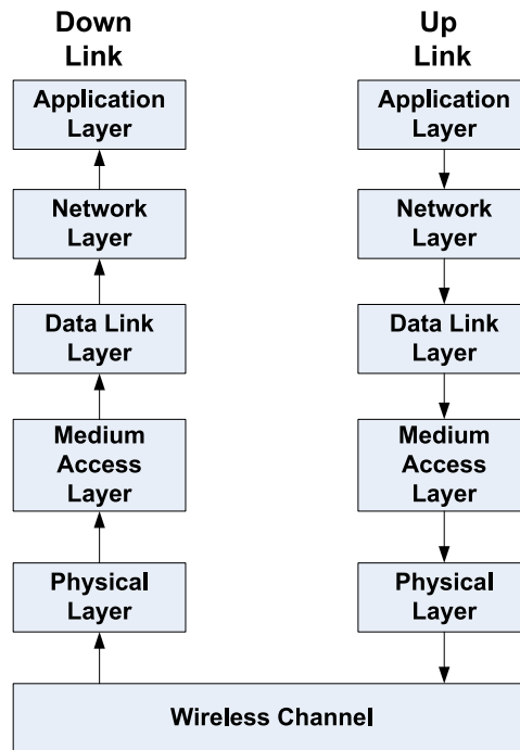
FIGURE 2.1: Reduced OSI model of wireless sensor networks for transmission (up link) and reception (down link).
