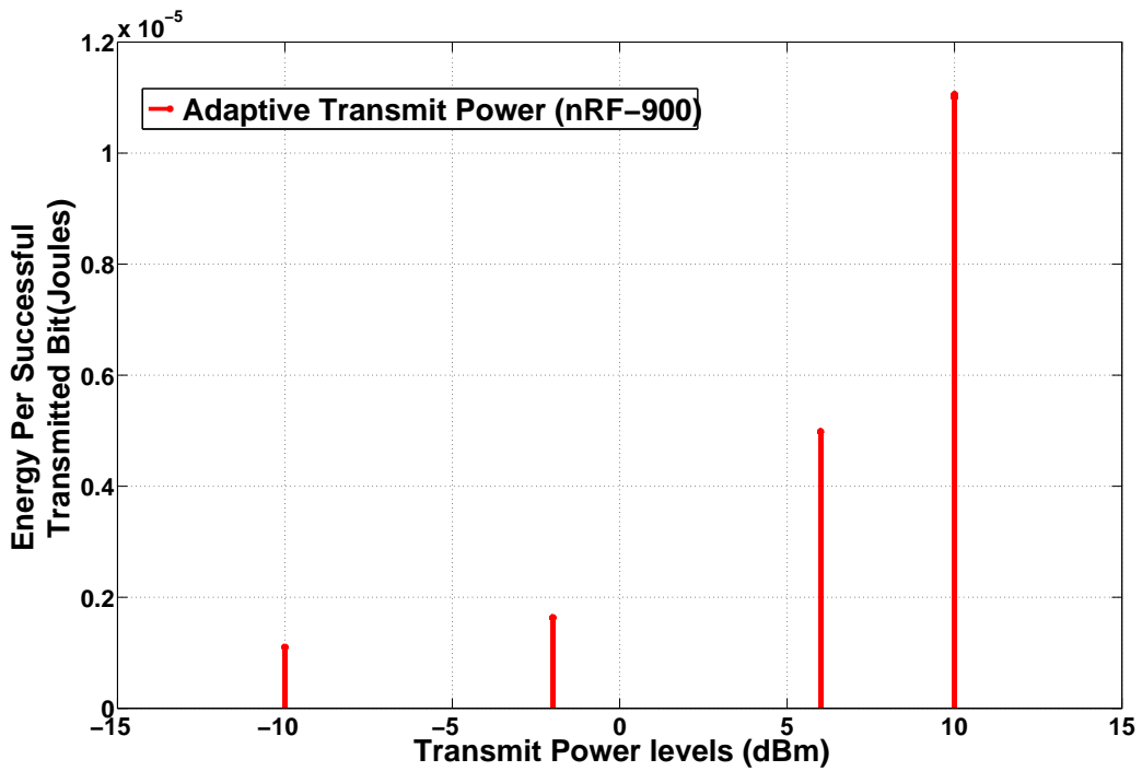
FIGURE 6.10: Best possible energy efficiency versus transmit power levels of nRF-900 after applying the adaptive transmit power optimization algorithm under the channel variations of model-d .
