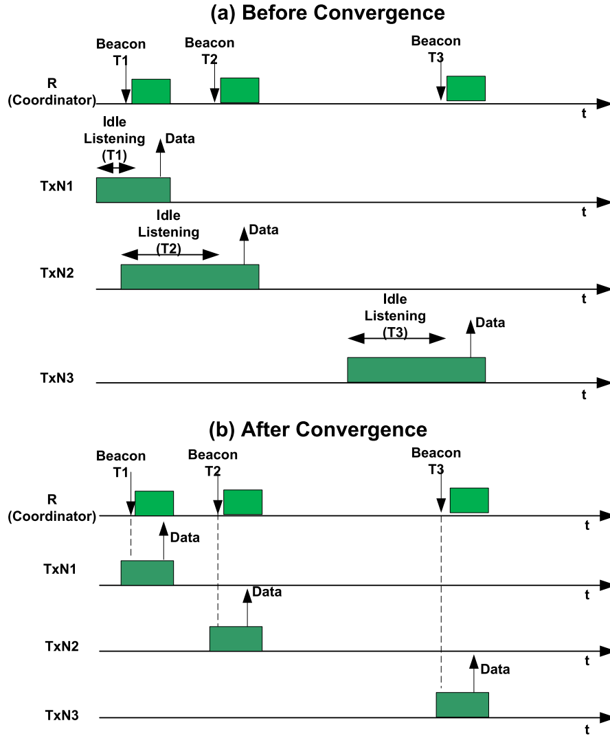
FIGURE 4.1: Traffic-aware dynamic MAC protocol is divided into two phases; the evolution phase before convergence (a) and the steady state phase after convergence (b). It is important to note that in the second phase the receive node (coordinator) has adapted its I_{wu} schedule as such that the idle listening is reduced.
