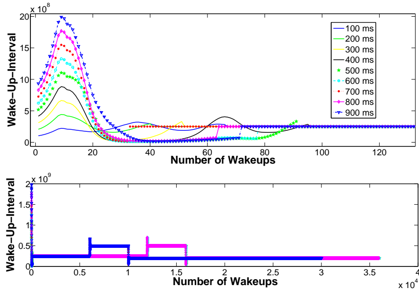
FIGURE 4.11: Wake-up interval adaptation for number of different initial wake-up interval values. Top figure is a zoomed version of the bottom one, also showing the behavior of convergence under variable traffic.
