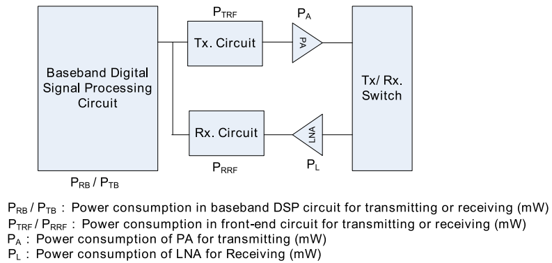
FIGURE 2.8: Component-based power model for WSN.
