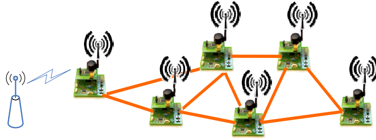
FIGURE 1.1: Sensor networks consisting of small nodes with an ability to sense the physical environment and communicate the information to the local (more powerful) base station.
