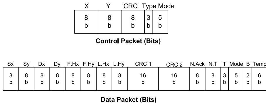
FIGURE 3.3: The Control Packet (wake-up-beacon and acknowledgment) consists of geographical network address (x,y) of the receive node which transmits the control packets, cyclic redundancy check (CRC) and the last byte contains the type of packet (3-bits) and the mode of communication (5-bits). The data packet consists of the network address of source and destination as well as the hop-addresses of the next and last hop-node, along with few bytes for acknowledgment number, temperature, battery, and N.T is frame buffer indicator.
