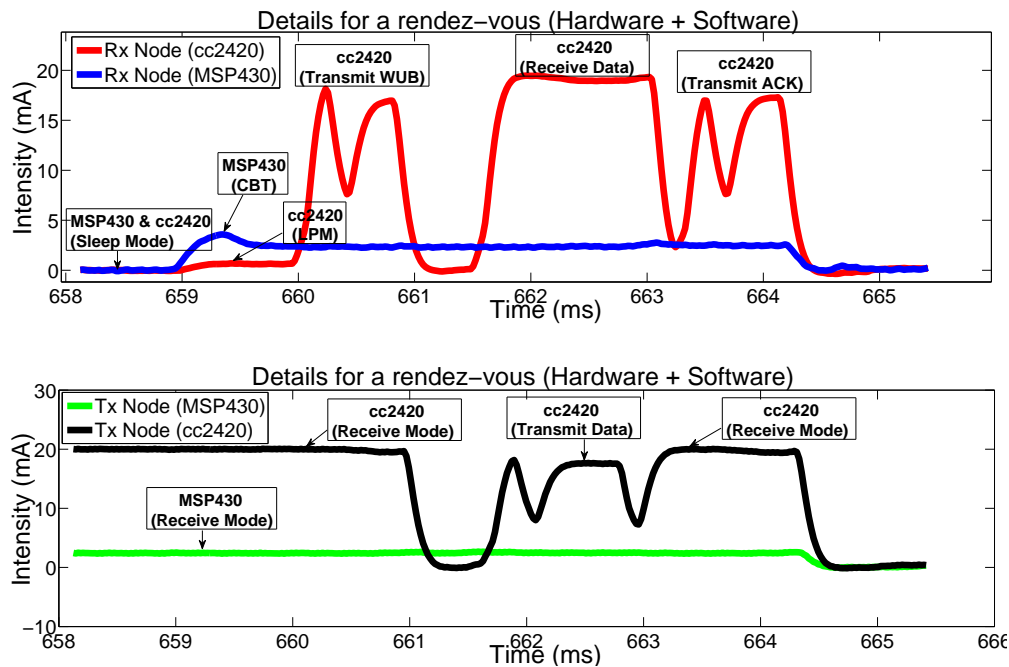
FIGURE 3.10: Details of software and hardware consumption: the software component i.e. MSP430 consumes 0.0 \mu A , 0.01 \mu A , 2.5 mA , and 3.7 mA , in sleep, low power mode (LPM), transmitting, and receiving modes respectively. Whereas, the hardware component i.e. cc2420 consumes 0.0 \mu A , 0.4 mA , 17.6 mA , and 19.6 mA , in sleep, low power mode (LPM), transmitting, and receiving modes respectively.
