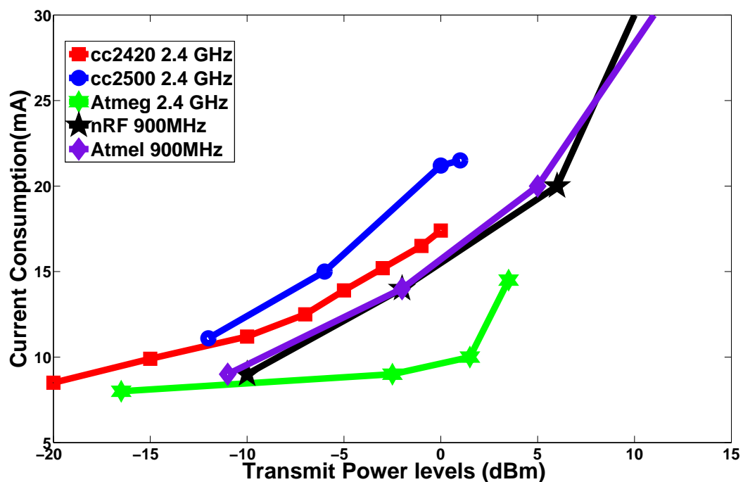
FIGURE 6.1: Power profile characteristics of different radio transceivers operating at 2.4GHz and 900MHz. The curves show the current consumption against various power levels of the radio.
