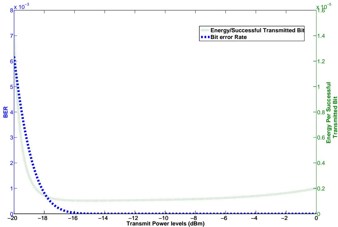
FIGURE 6.2: Energy per successful transmitted bit and corresponding bit error rate versus different transmit power levels under fixed noise ( -90\text{dBm} ).
