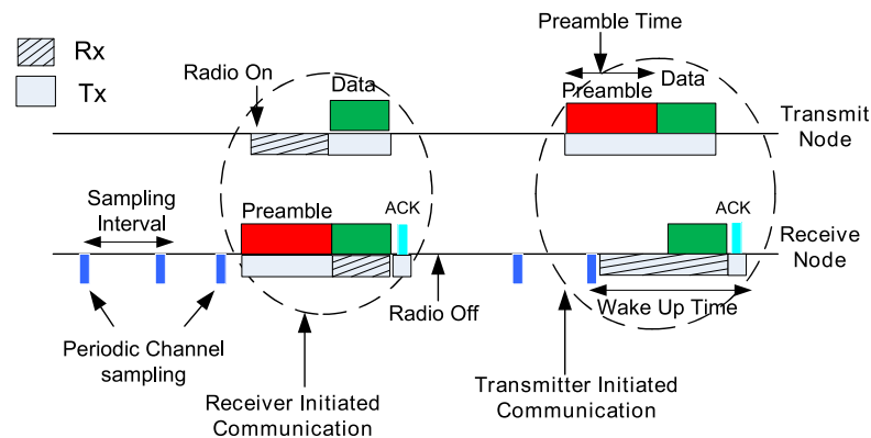
FIGURE 2.2: General mechanism of preamble sampling protocols. The communication can either be initiated by receive or transmit node. If the communication is initiated by the receiver then the receive node will send the preamble to the transmit node and the transmit node will respond with the data packet, whereas if it is initiated by the transmitter then the preamble will be sent by the transmit node followed by the data.
