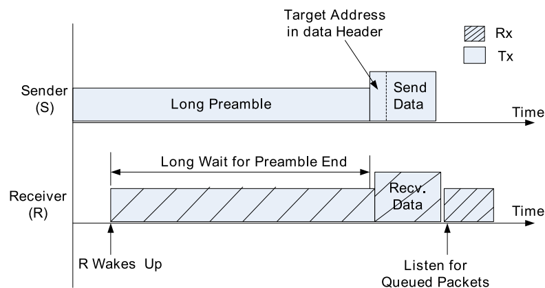
FIGURE 2.3: BMAC protocol.
