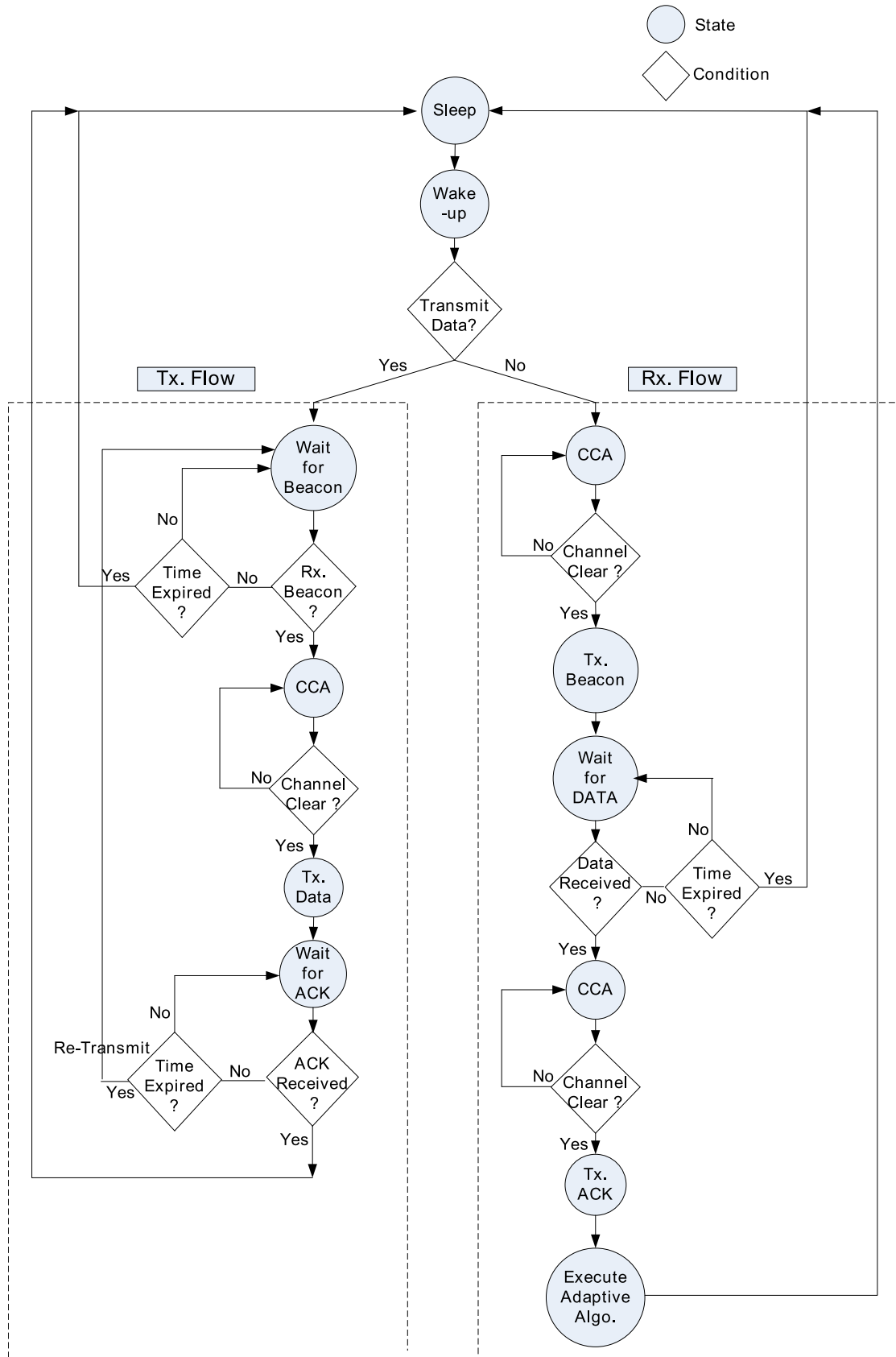
FIGURE 4.16: State machine being used to simulate TAD-MAC protocols in WSNet simulator. The scheduler moves to the next state based on the occurrence of an event, otherwise it keeps on waiting until the timer expires and then it proceeds backward.
