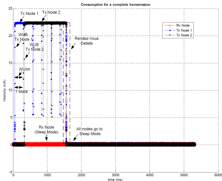
FIGURE 3.6: Total current consumption: two nodes want to transmit the data to the same destination node. In this particular case, after 5 blocks , the transmitter wakes up and sends its WUB , and a rendez-vous (detailed in Fig. 3.8) occurs between the two nodes on the single channel. The total current consumption including the cc2420 and MSP430 is 22.5mA.
