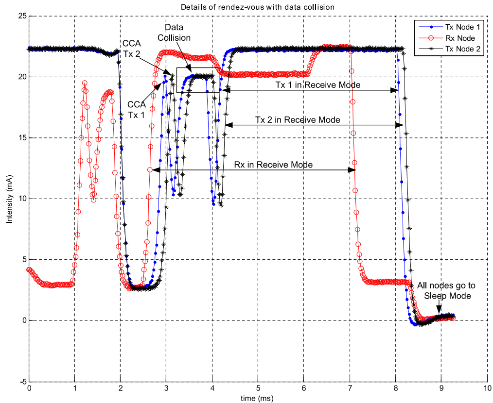
FIGURE 3.11: Unsuccessful communication because of data collision, which is one of the bad executing scenario as mentioned in the energy model. This results in extra power consumption because of the waiting of ACK for the transmit nodes and data packet for the receive node. After about 4 msec. of wait in monitoring state, all nodes go to sleep mode.
