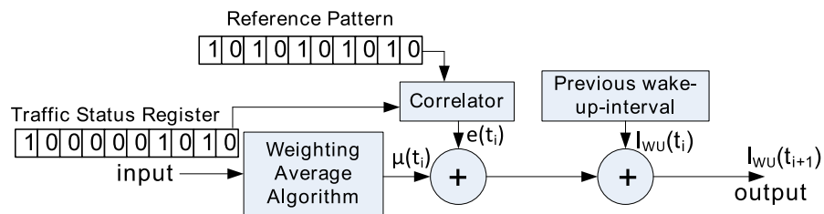
FIGURE 4.4: Adaptive wake-up interval system.
