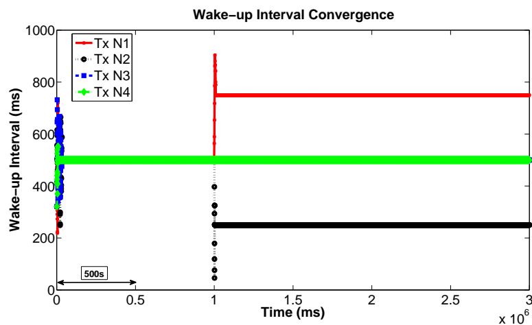
FIGURE 5.4: Convergence of wake-up interval towards a steady state value for variable sensing rates. The traffic rate for node 1 and node 2 changes from 1 s to 1.5 s and 500 ms respectively.
