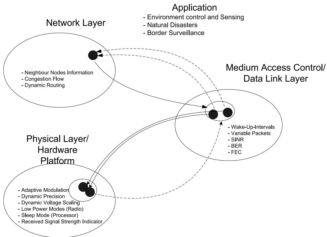
FIGURE 2.6: Generic framework: the parametric-based cross layer interaction between the network, link/medium access control and the physical layers for the given application. Performance metrics such as SINR , BER , RSSI , etc., can help to adjust different parameters such as FEC selection, Wake up Intervals , Adaptive Modulation , Dynamic Precision etc.
