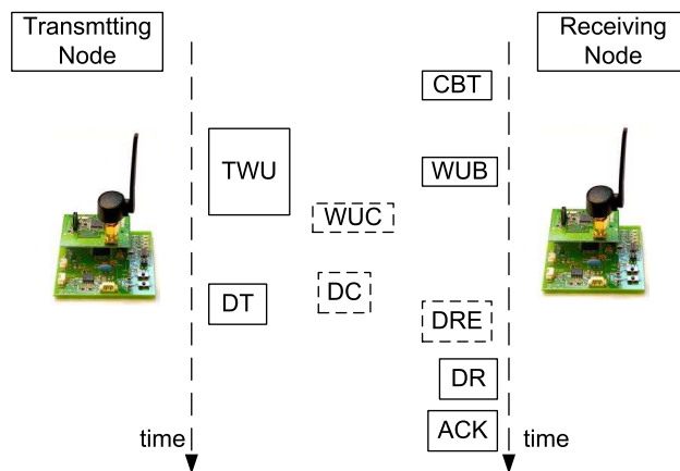
FIGURE 3.12: Communication phase between transmit nodes and receive nodes : The energy model is based on execution traces of different scenarios which occur during the communication. These scenarios include: CBT (calculation before transmission), TWU (transmitter wake-up), WUB (wake-up-beacon), WUC (wake-up-collision), DT (data transmission), DR (data received), DC (data collision), DRE (data received with errors) and ACK (acknowledgment of data).
