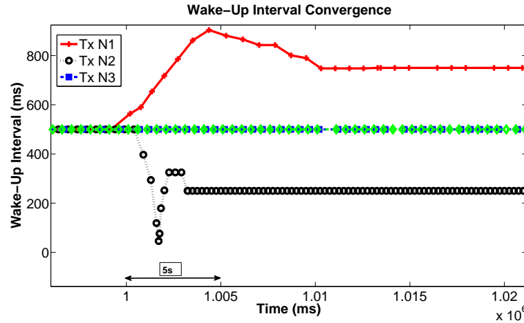
FIGURE 5.5: Zoomed version of Fig. 5.4 to show convergence after changing the traffic rate. It can be seen that the receive node converges very efficiently as soon as the traffic changes. In this particular example, the traffic rate for node 1 and node 2 changes from 1 s to 1.5 s and 500 ms respectively. Node 1 converges to a steady wake-up interval value of 750 ms, whereas node 2 converges to 250 ms for the traffic pattern of [10101010...].
