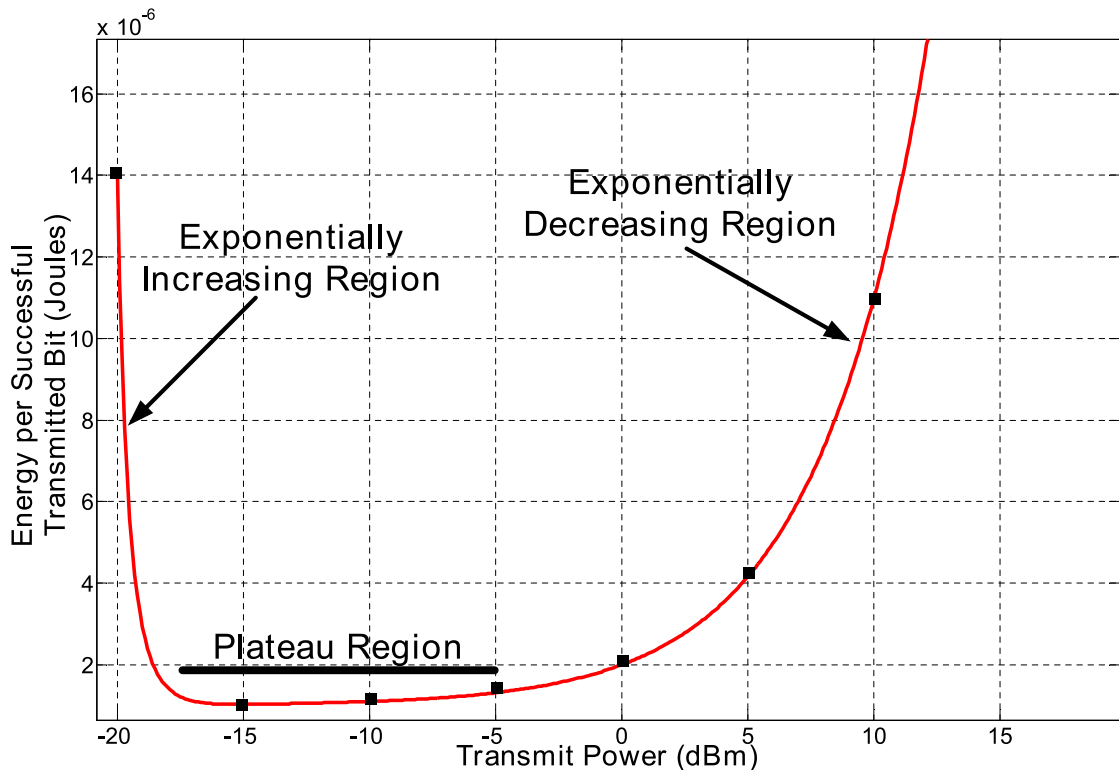
FIGURE 6.3: Energy consumption under fixed noise power ( -90\text{dBm} ) against different transmit powers.
