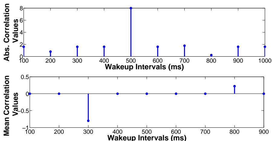
FIGURE 4.8: Behavior of e variable against different (fixed) wake-up interval values calculated through correlation technique. First is the mean of the absolute value of correlation and second is only the mean of correlation.
