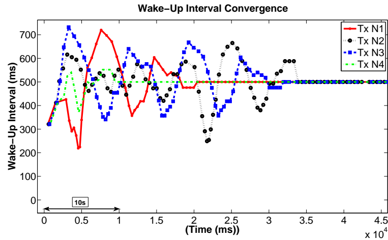
FIGURE 5.3: Receive node adaptation with respect to transmit nodes based on the wake-up interval for a fixed data rate i.e. 1 s. It is to mention here that the reference clock's increment is 1 (ms), therefore all the time values are in ms.
