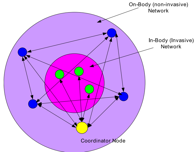
FIGURE 5.2: Hybrid network topology: invasive sensor nodes are connected with a coordinator through star network, whereas non-invasive nodes are configured through mesh topology.
