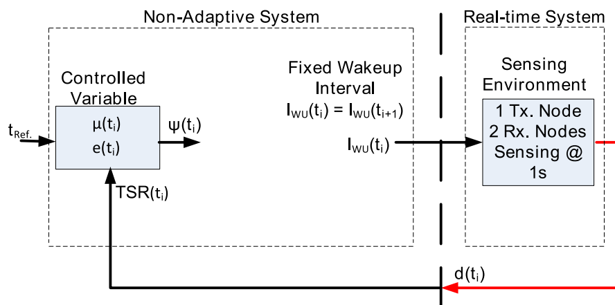
FIGURE 4.6: The open loop form of the system consists of two parts. The first one is a non-adaptive system that compute \psi (for the purpose of analyzing controlled variables) but does not used it to update the wake-up interval whereas, the second part is real-time system which is the wireless sensor network.
