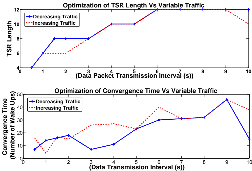
FIGURE 5.6: Optimization of the TSR length and the corresponding convergence speed for different data transmission rates, starting from two packets per second to one packet in ten seconds. It can be seen that the convergence speed increases as the rate reduces, this is due to the fact that with reduced rate TSR is filled slowly and it results in slow convergence speed.
