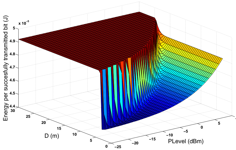
FIGURE 3.16: Total energy per successfully transmitted useful bit between nodes i and j as a function of the distance D_{i,j} and of the transmission power level P_{Level} .
