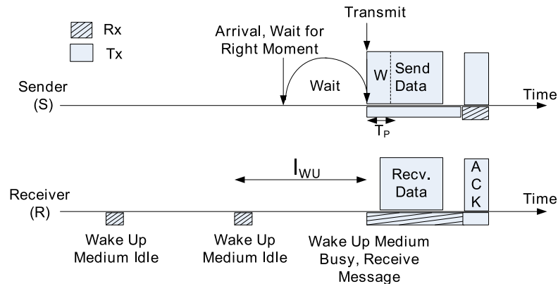
FIGURE 2.5: WiseMAC protocol.
