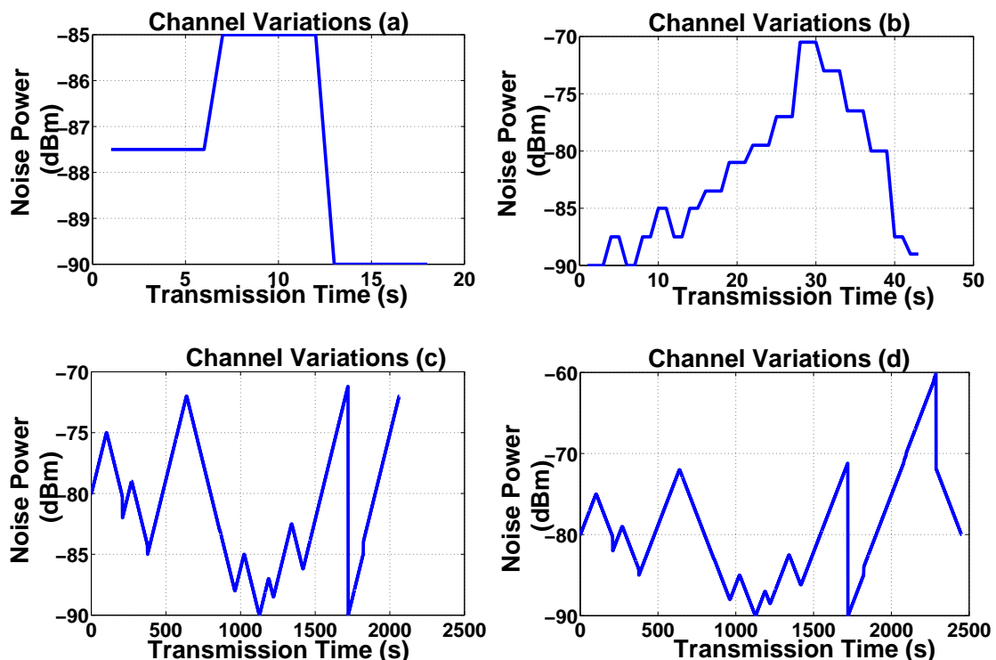
FIGURE 6.4: Different variants of varying noise power based Channel profiles. The limits of variations of the noise power are according to the maximum power that is available in most widely used radio transceivers for WSN.
