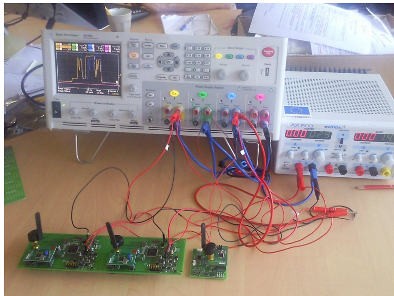
FIGURE 3.5: The platform setup for measurements is constituted of three WSN PowWow nodes connected to the DC Power Analyzer. The external power supply of 3.3 volts is used. Four modules of the N6705A are connected with the cc2420 and MSP430, to measure the current consumption of each component of the connected nodes as shown in Fig. 3.10.
