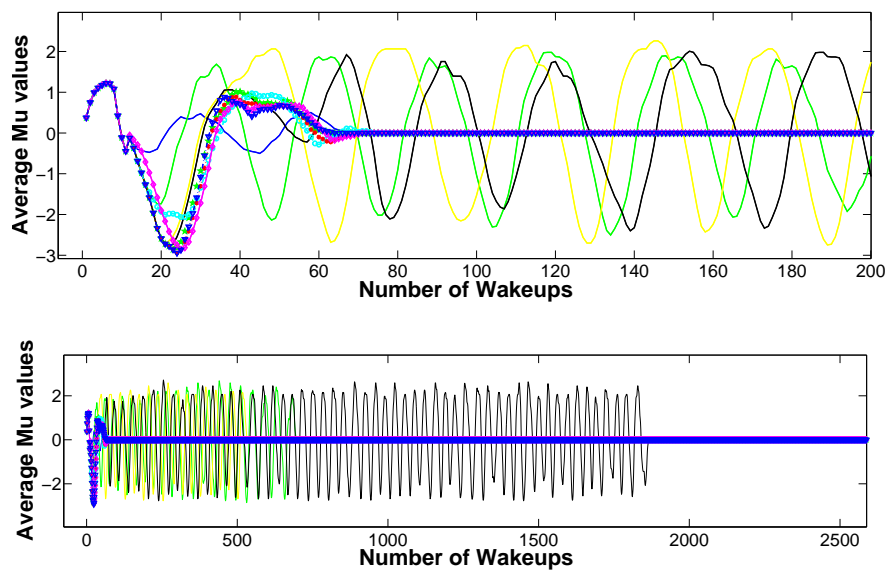
FIGURE 4.14: Variable \mu behavior for number of different initial wake-up interval values. Top figure is a zoomed version of the bottom one.
