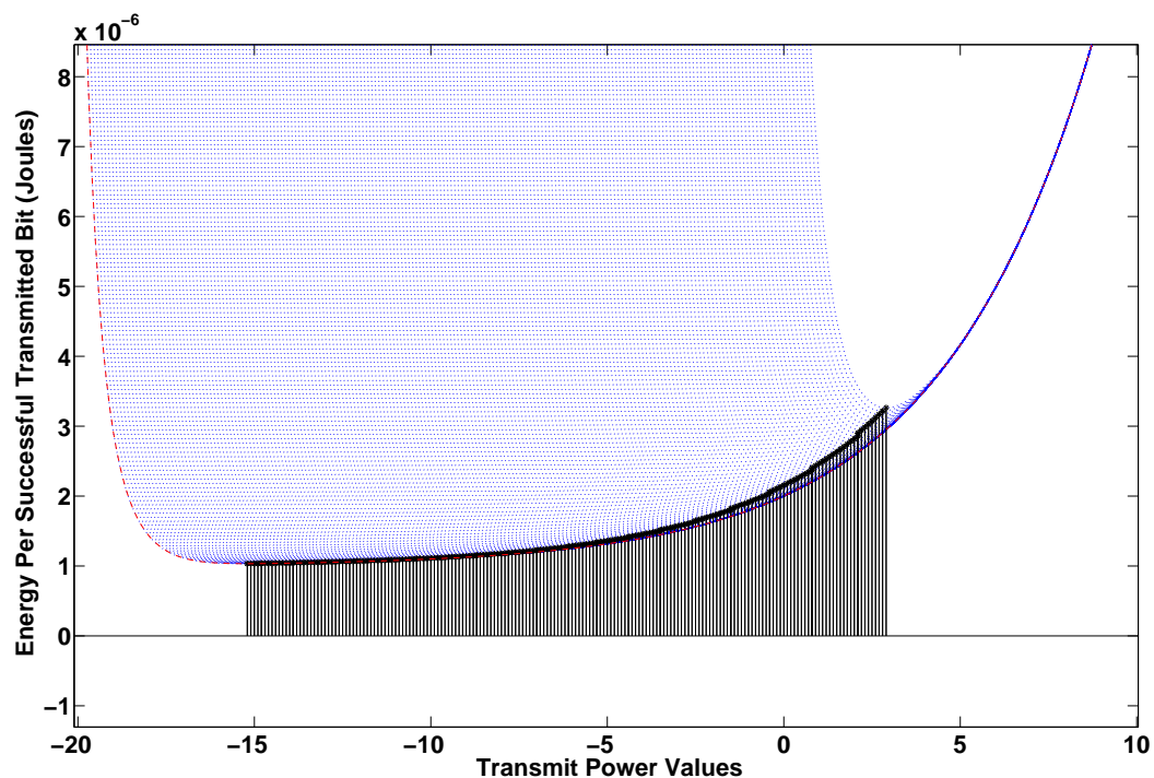
FIGURE 6.7: Energy consumption versus number of different transmit power values. Optimal points on each curve is identified and can be seen by a dark black line. Whereas, the outlined curve (in red) represents the best possible result for energy efficiency.
