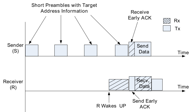
FIGURE 2.4: X-MAC protocol.
