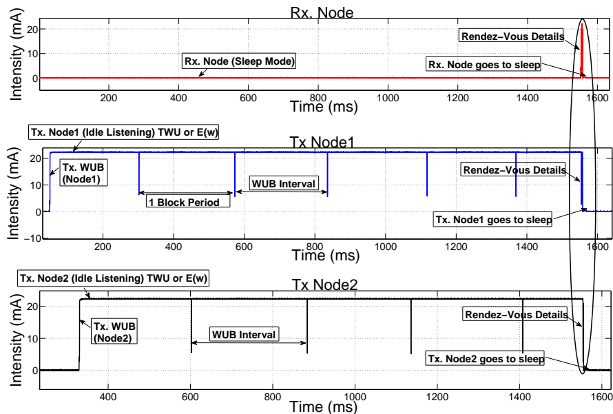
FIGURE 3.7: Same as Fig. 3.6, only three nodes are presented separately for clarity.
