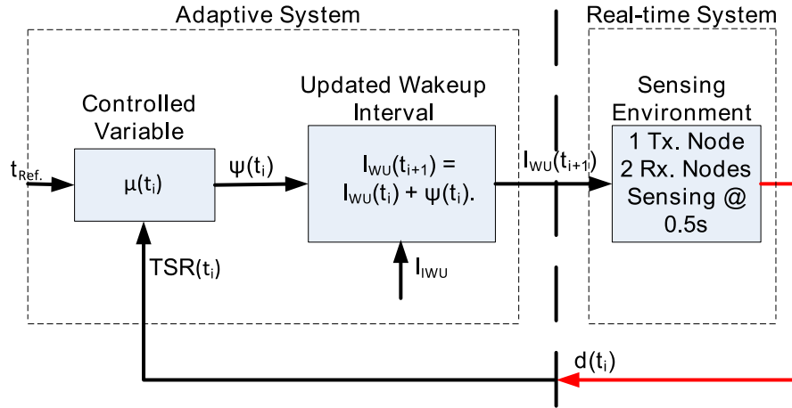
FIGURE 4.10: Closed-loop form of the system considers the influence of feedback into the computation of the update of the wake-up interval in the adaptive system. It is to note that only \mu and e are considered as controlled variables in the adaptive system.
