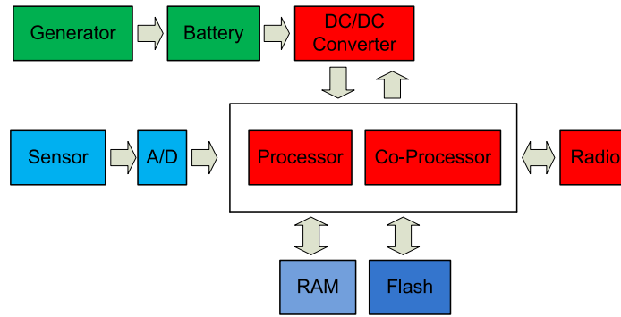
FIGURE 2.9: Basic Block Diagram of Wireless Sensor Node.
