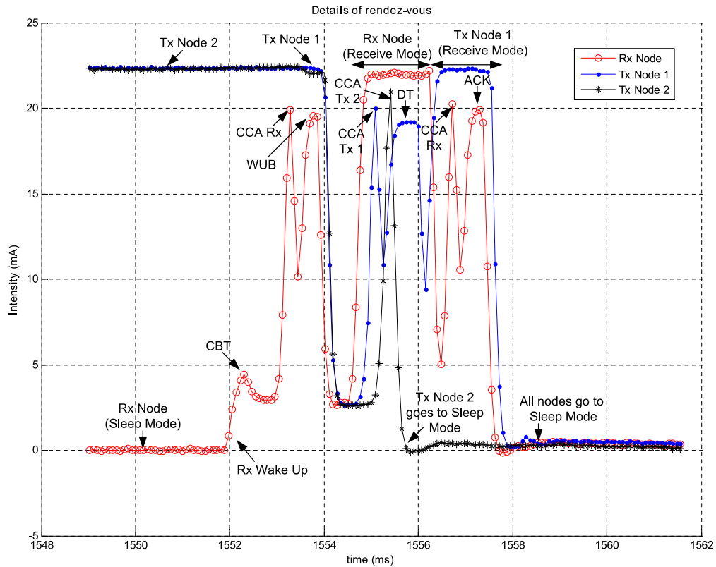
FIGURE 3.8: Details of a rendez-vous: three phases i.e. WUB , DT and ACK are clearly shown, and all the events are described during the rendez-vous. The Tx node 1 senses the channel first and hence occupies the channel before the Tx node 2 . Therefore the collision is being avoided.
