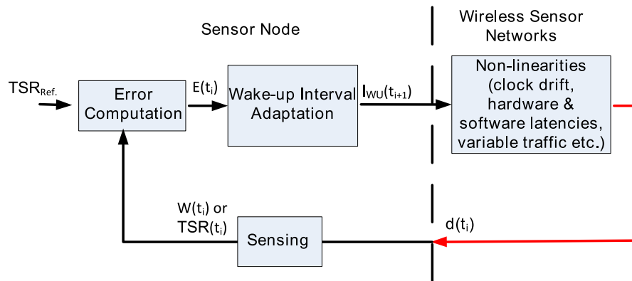
FIGURE 4.5: System model used to characterize the adaptive wake-up interval algorithm.
