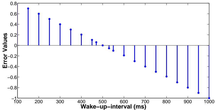
FIGURE 4.9: Variations of e variable against different (fixed) wake-up interval values computed by counting number of ones in TSR.
