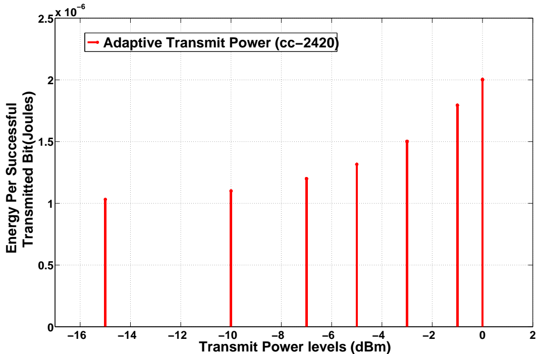
FIGURE 6.8: Best possible energy efficiency versus transmit power levels of cc-2420 after applying the adaptive transmit power optimization under the channel variations of model-c .
