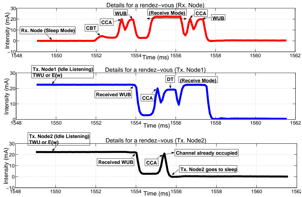
FIGURE 3.9: Same as Fig. 3.8, only three nodes are presented separately for clarity.
