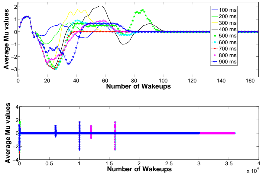
FIGURE 4.12: Behavior of \mu for number of different initial wake-up interval values. Top figure is a zoomed version of the bottom one.
