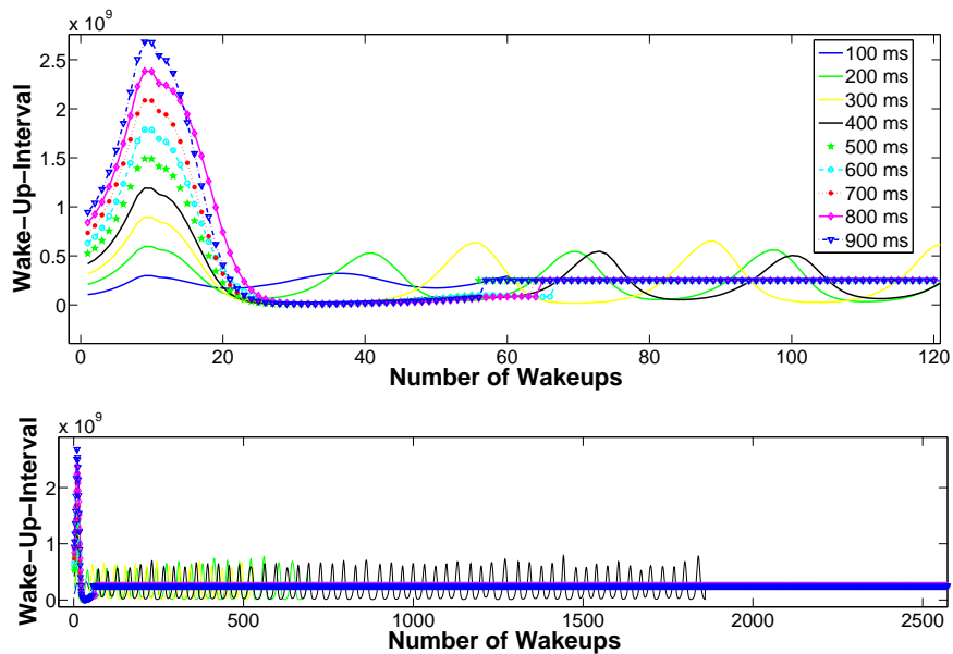
FIGURE 4.13: Behavior of wake-up interval adaptation for number of different initial wake-up intervals. Few initial wake-up interval values result in oscillation and hence converge much later than others. The top figure is a zoomed version of the bottom one.
