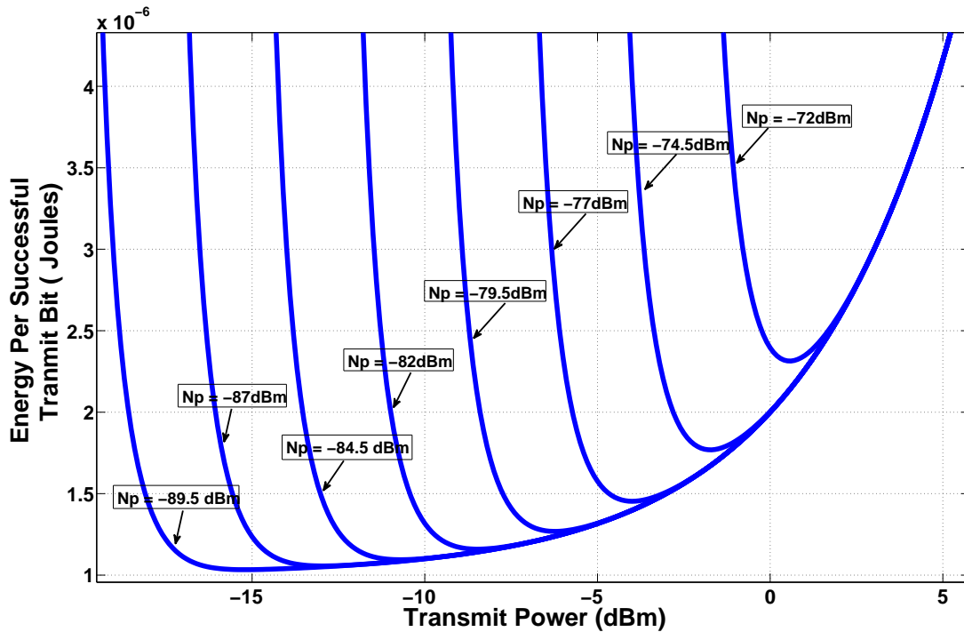
FIGURE 6.5: Energy consumption versus transmit power under varying but fixed noise power N_p .
