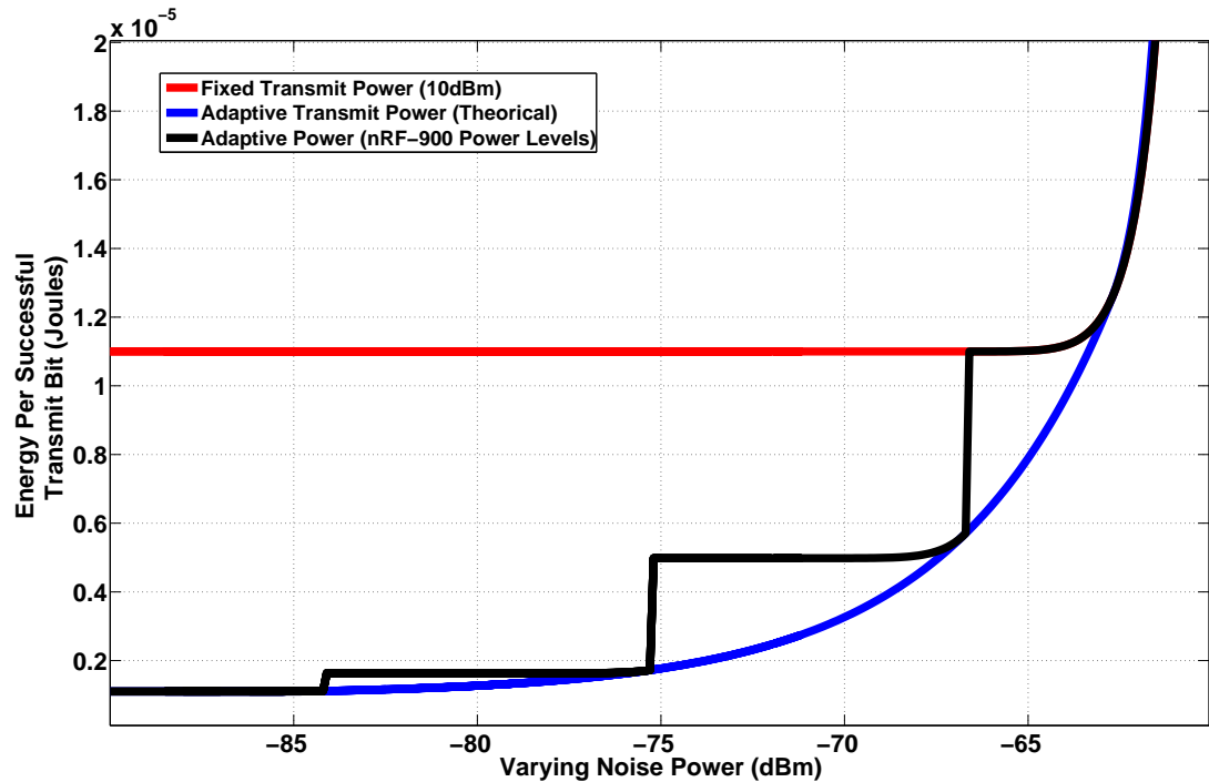
FIGURE 6.13: Comparison between an adaptive transmit power optimization versus the fixed transmit power at maximum level of nRF-900 i.e. (10dBm).
