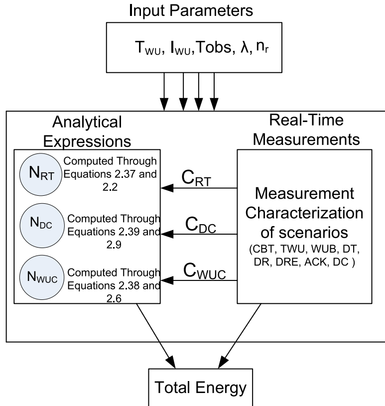
FIGURE 3.13: Hybrid Energy Model. The model utilizes the real-time measurements with an identification of typical scenarios that can occur in asynchronous WSN communication. By the help of the analytical model which evaluates the expressions for number of re-transmissions, number of wake-up-collisions and number of data collisions, the total global cost and the total energy consumption is evaluated.
