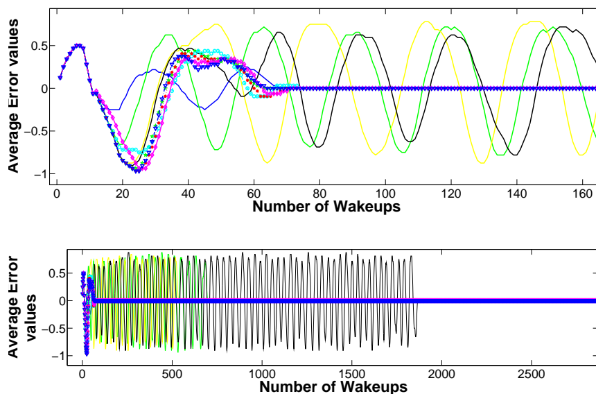
FIGURE 4.15: Behavior of variable e for number of different initial wake-up interval values. Top figure is a zoomed version of the bottom one.
