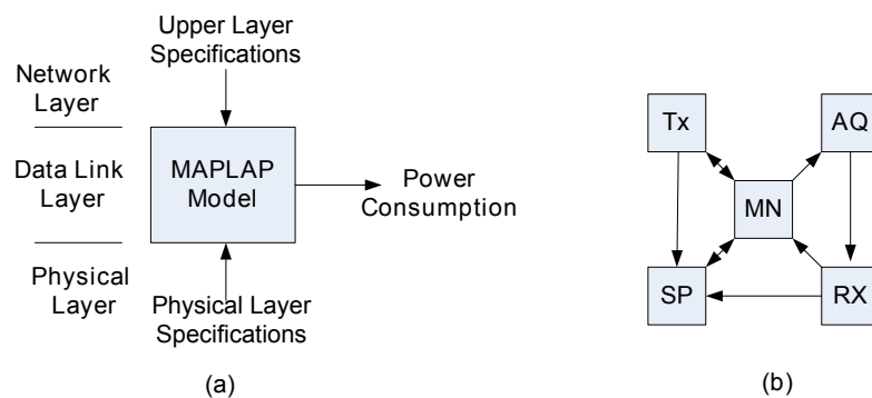
FIGURE 2.7: (a) MAC And Physical LAYER Power (MAPLAP) Model. (b) State-based wireless sensor networks.
