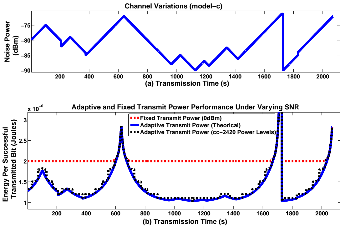
FIGURE 6.9: (a): Channel variations 'model-c'. (b): Performance of the adaptive transmit power technique against the channel variations of model-c over time.
