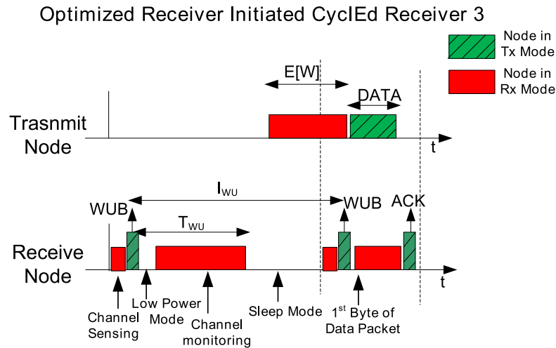
FIGURE 3.4: Optimized 3-way handshake receiver initiated cyclEd receiver scheme. The N -Data slots are not necessary to avoid the collision, instead the receiver only requires the first byte of the data packet. Therefore, the idle channel monitoring is irrespective of data slots but adjustable according to the application.
