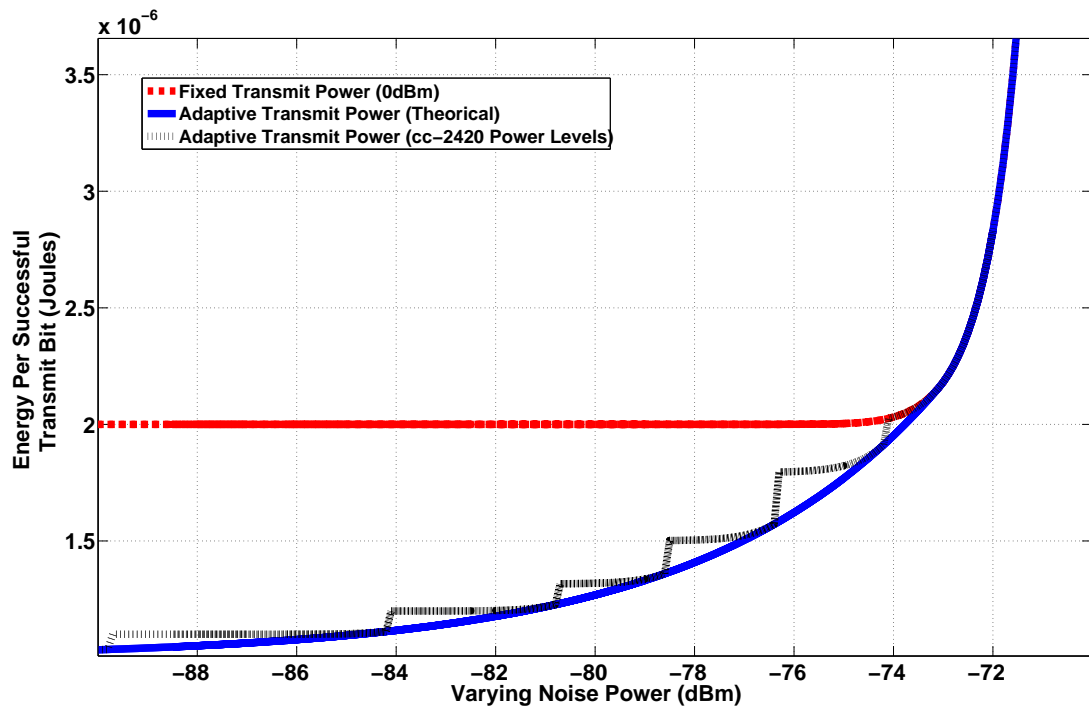
FIGURE 18: Comparison of energy performance between an adaptive transmit power optimization versus the fixed transmit power at maximum level of cc-2420 i.e. (0 dBm).
