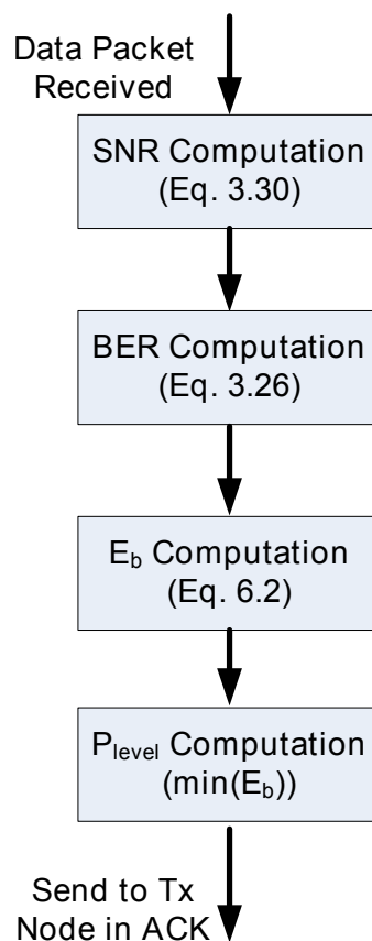
FIGURE 6.6: Execution flow of adaptive transmit power control technique.
