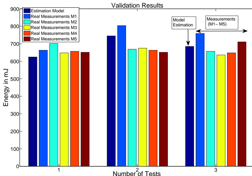
FIGURE 3.15: Test 1, Test 2 and Test 3 correspond to fixed parameters settings of I_{wu} , T_{wu} , T_{obs} , and TWU as 100ms , 5ms , 300s , 2s , whereas the data reception at node C varies from 1s , 500ms and 100ms . Y-Axis represents the energy consumed in mJ for an observation time of 300s .
