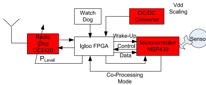
FIGURE 3.2: Hardware block diagram of PowWow. The key components in terms of power consumption are processing units (T.I MSP430, Actel IGLOO FPGA), DC/DC converter (used for voltage scaling), and the radio chip (T.I. cc2420).
