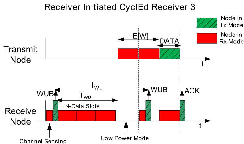
FIGURE 3.1: RICER3 is a 3-way handshake receiver initiated cycled receiver scheme. The N -data slots are placed in order to avoid the collision which happens when two nodes send the data to the same destination node at the same time in response to the wake-up-beacon. E[w] is the expected waiting time, T_{wu} is the total wake-up time of the receiver, I_{wu} is the wake-up interval of each node, WUB is the wake-up-beacon signal and Ack is the acknowledgment signal.
